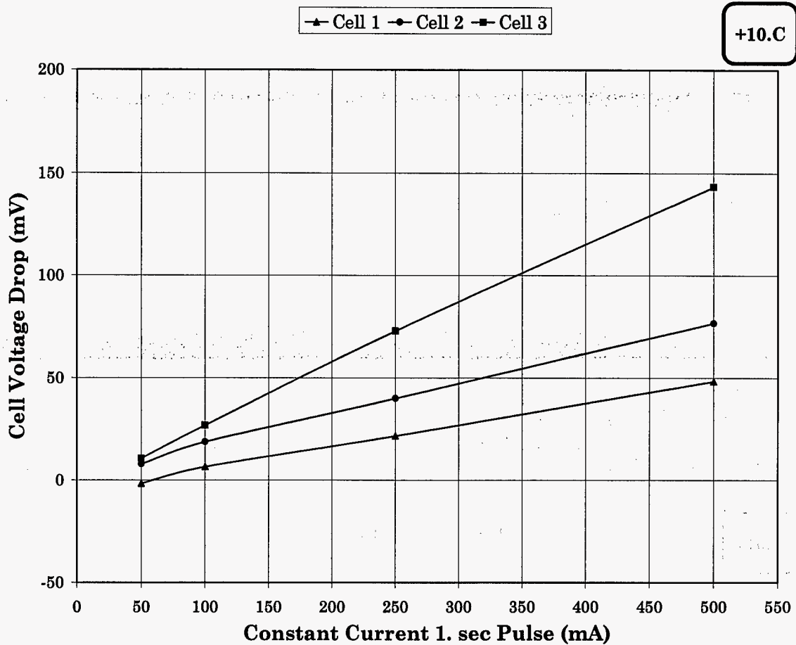
Figure 8B. Cell voltage drop at 10°C as a function of current pulse amplitude. Pulse duration = 1 sec., all cells had accumulated 80 - 100 cycles.
