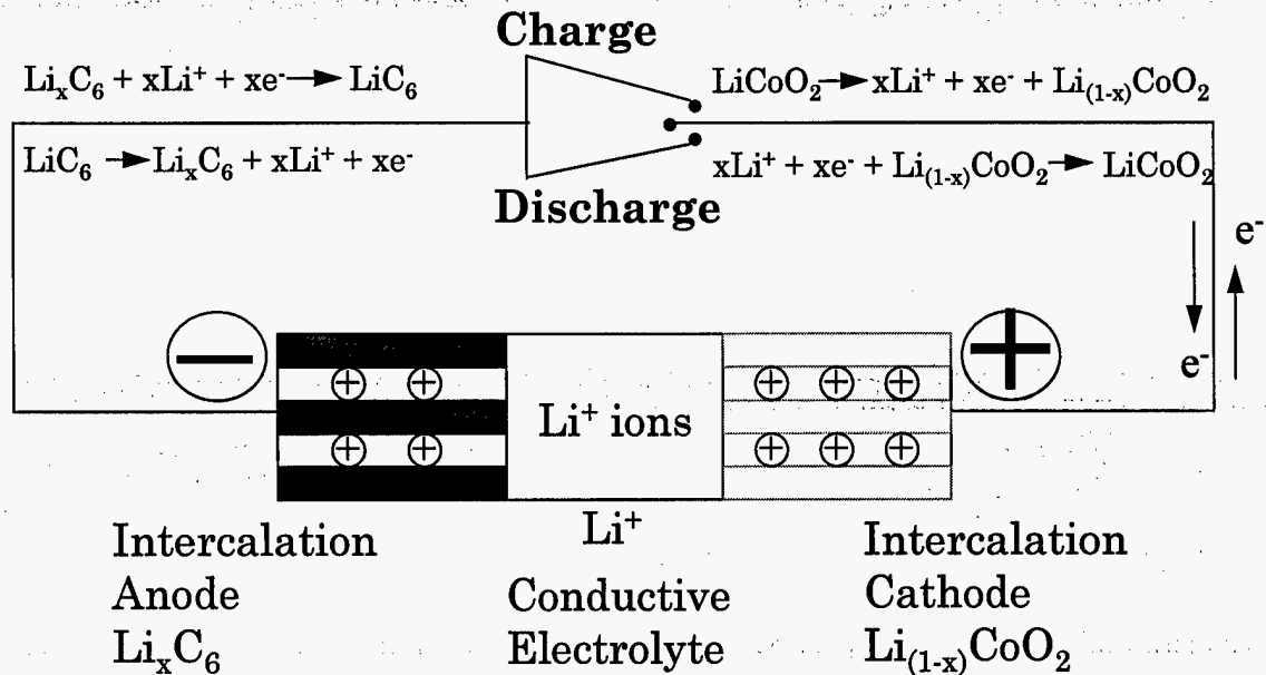
Figure 1. Schematic representation of a rocking-chair lithium-ion rechargeable battery.
