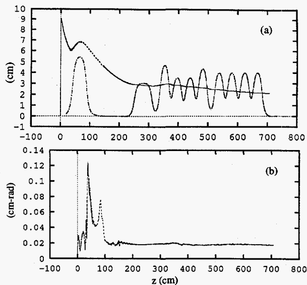
Figure 3: (a) Beam edge radius with overlay of axial magnetic field and (b) normalized emittance from the injector through the first eight cell magnets.
