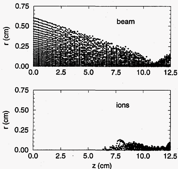
Figure 4: Simulation of space-charge-limited proton emission from target using IPROP. Beam and proton positions are shown after 6.7 ns.
