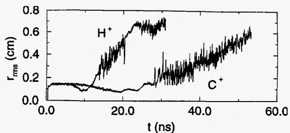
Figure 6: Beam RMS radius near target for ITS parameters with space-charge-limited emission of H^+ and C^+ ions from the target.
