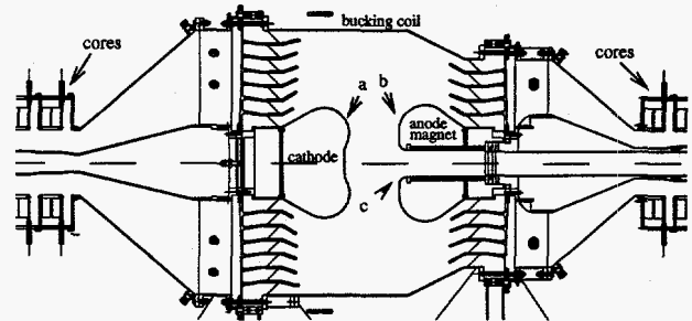
Figure 1: Layout of 4-pulse injector. The field stresses (kV/cm) with (without) the beam at the points marked are: (a) 184 (187), (b) 161 (157) (c) 185 (159).
