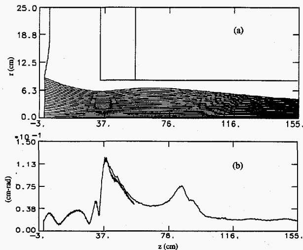
Figure 2: Simulation of 4 MeV, 4 kA diode in Fig. 2 using IVORY showing (a) particle positions and (b) normalized edge emittance vs. z .
