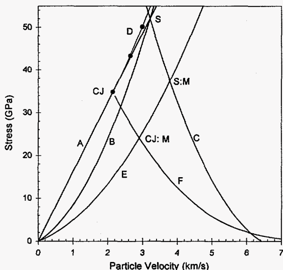
FIGURE 4. Hugoniot and isentropes relevant to calculating the reaction zone parameters. PBX 9501 is shown here. Explanations of the labels follow. (A) Detonation Rayleigh line. (B) Unreacted Hugoniot for the explosive. (C) Reflection of the unreacted Hugoniot for the explosive. (D) Explosive products Hugoniot. (E) PMMA window Hugoniot. (F) Explosives products isentrope calculated using the JWL EOS. (S) ZND spike point. (S:M) Spike point matched onto the PMMA Hugoniot. (CJ) Chapman-Jouguet or CJ state. (CJ:M) CJ state matched onto the PMMA Hugoniot. The matched spike and detonation points are those which would be observed.
