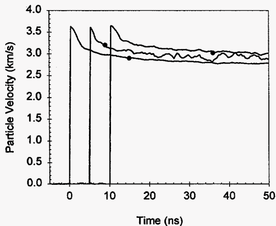
FIGURE 2. Wave Profile obtained for PBX9501, EDC-37, and PBX9404 shown left to right, respectively. The time origins for the EDC-37 and PBX9404 profiles have been shifted. The calculated ends of the reaction zones are shown as dots (see text).
