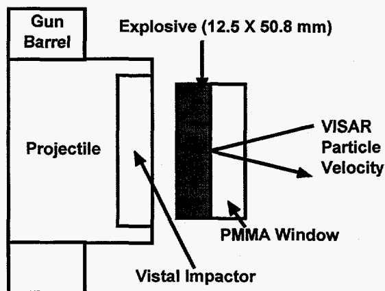
FIGURE 1. Cross section view of the projectile and target.
