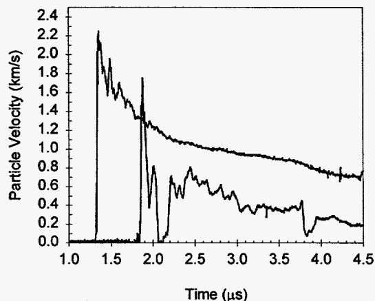
FIGURE 3. Detonation wave profiles obtained for fine particle and coarse particle HMX shown left to right respectively. The time difference is the difference in initiation times.
