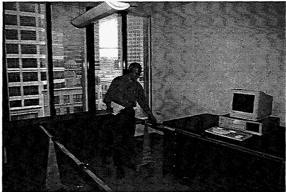
Figure 1. Interior view of the full-scale test room outfitted with the prototype automated venetian blind and an indirect/ direct lighting system. The two rows of workplane illuminance sensors are used for monitoring purposes. The 12 mm (0.5 in) wide blinds are difficult to detect in this photograph.
