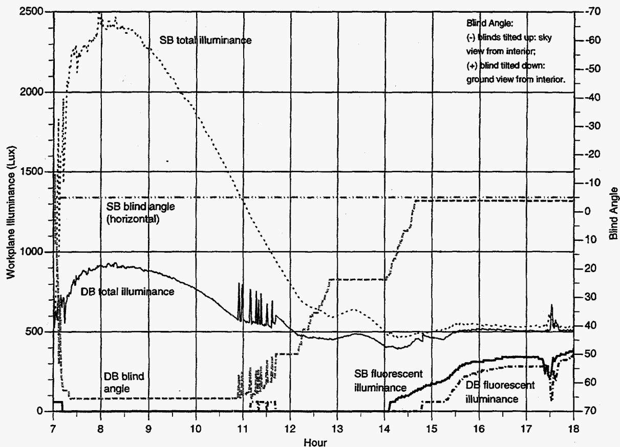
Figure 2. Monitored total workplane illuminance, fluorescent lighting illuminance, and blind angle for the static horizontal blind (SB) and the dynamic venetian blind (DB), both with daylighting controls. Daily cooling load savings were 21%. Peak demand savings were 13%. Daily lighting energy savings were 21%. Data are shown for southeast facing offices in Oakland, California on August 15, 1996.
