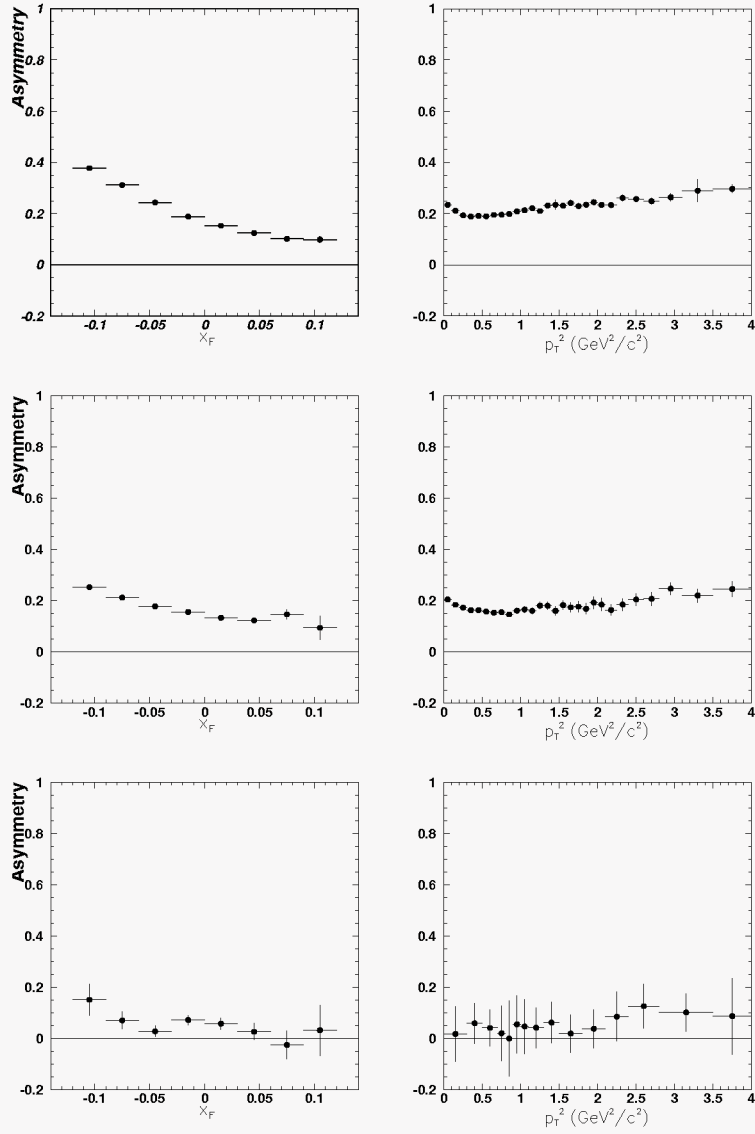
Figure 1: Preliminary results for 6% of the E791 data for \Lambda and 2/3 for \Xi and \Omega . Statistical errors only. \Lambda^0/\bar{\Lambda}^0 (top), \Xi^-/\Xi^+ (middle) and \Omega^-/\Omega^+ (bottom) asymmetries vs. x_F (left) and p_T^2 (right).
