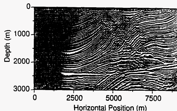
Fig. 2 Image obtained by common-shot prestack depth migration of the IFP Marmousi synthetic data set using the phase-screen method. Frequency components from 10 to 50 Hz were used in the migration.
