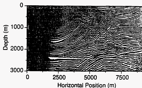
Fig. 3 Same as Fig. 2, except frequency range used in migration is 15 to 35 Hz.
