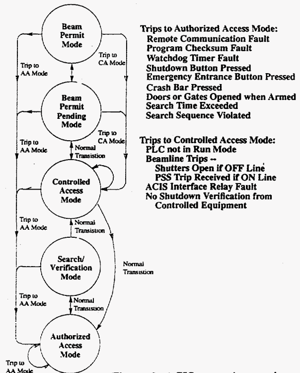
Figure 3: ACIS operating modes.
