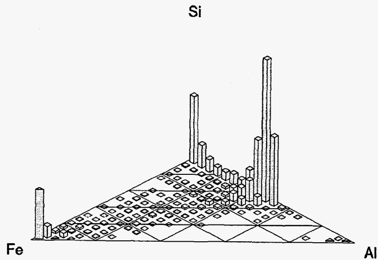
Figure 5-9 Fe-Al-Si ternary histogram of staged combustion Pittsburgh #8 ash (bottom, 75% burnout)
