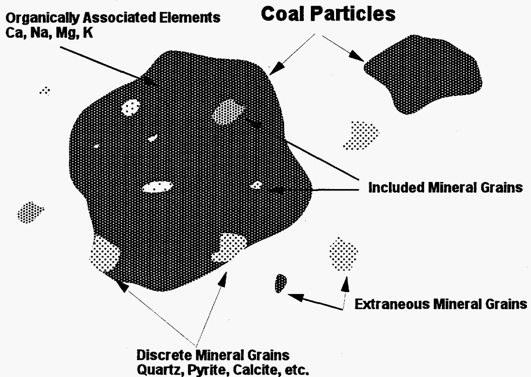
Figure 2-3 Occurrence of mineral matter in coal
