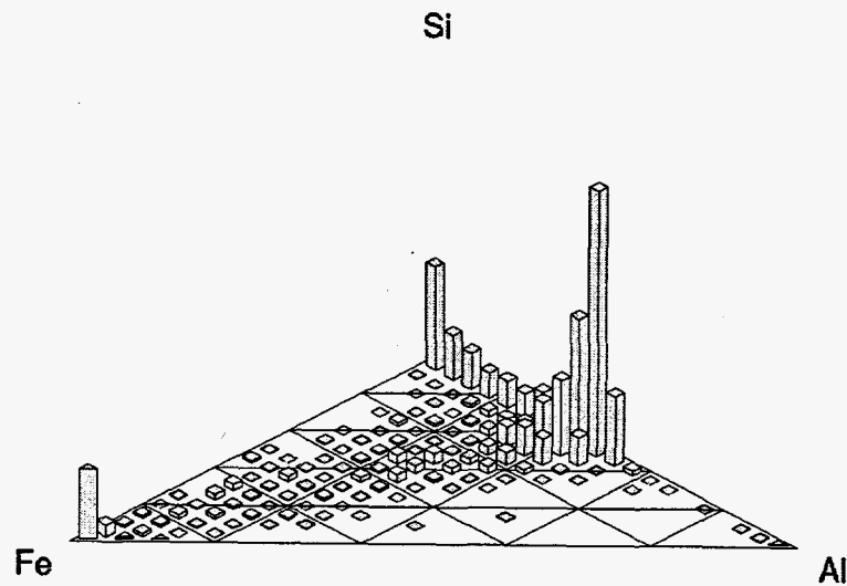
Figure 5-8 Fe-Al-Si ternary histogram of conventional Pittsburgh #8 ash (bottom, 90% burnout)
