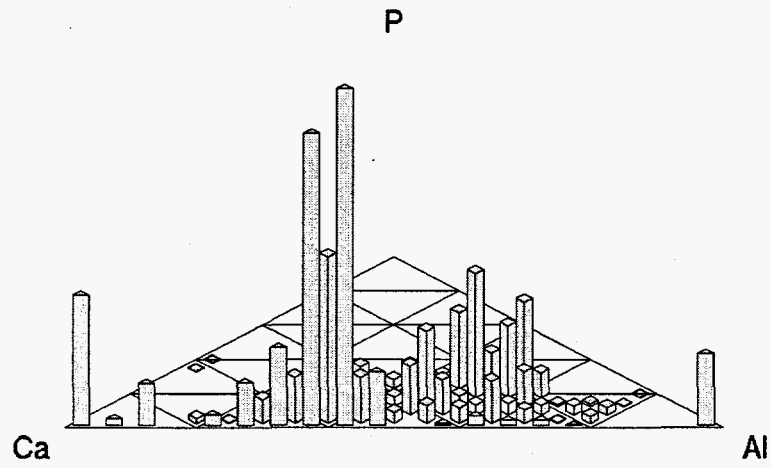
Figure 4-13 Ca-Al-P ternary histogram of conventional ash
