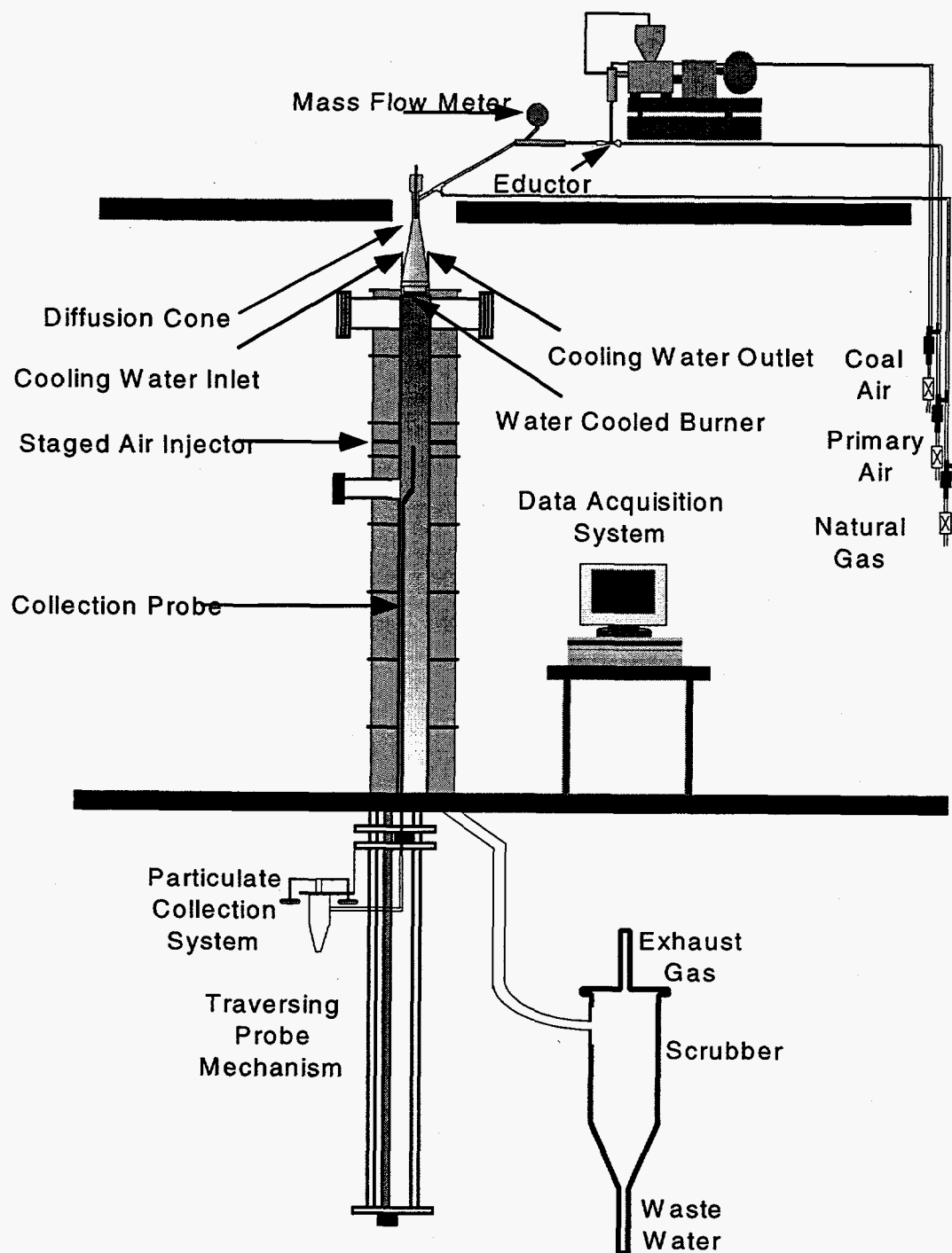
Figure 3-1 Laboratory Combustor
