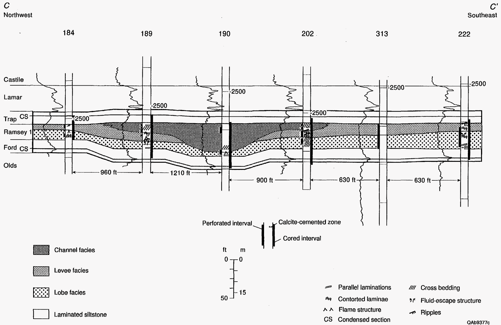
Figure 27. Cross section C-C' through the southern part of Geraldine Ford field, where only the Ramsey 1 sandstone is present. Channel, levee, and lobe facies are similar to those in cross section B-B' (fig. 26). Location of cross section is shown in figure 2.
