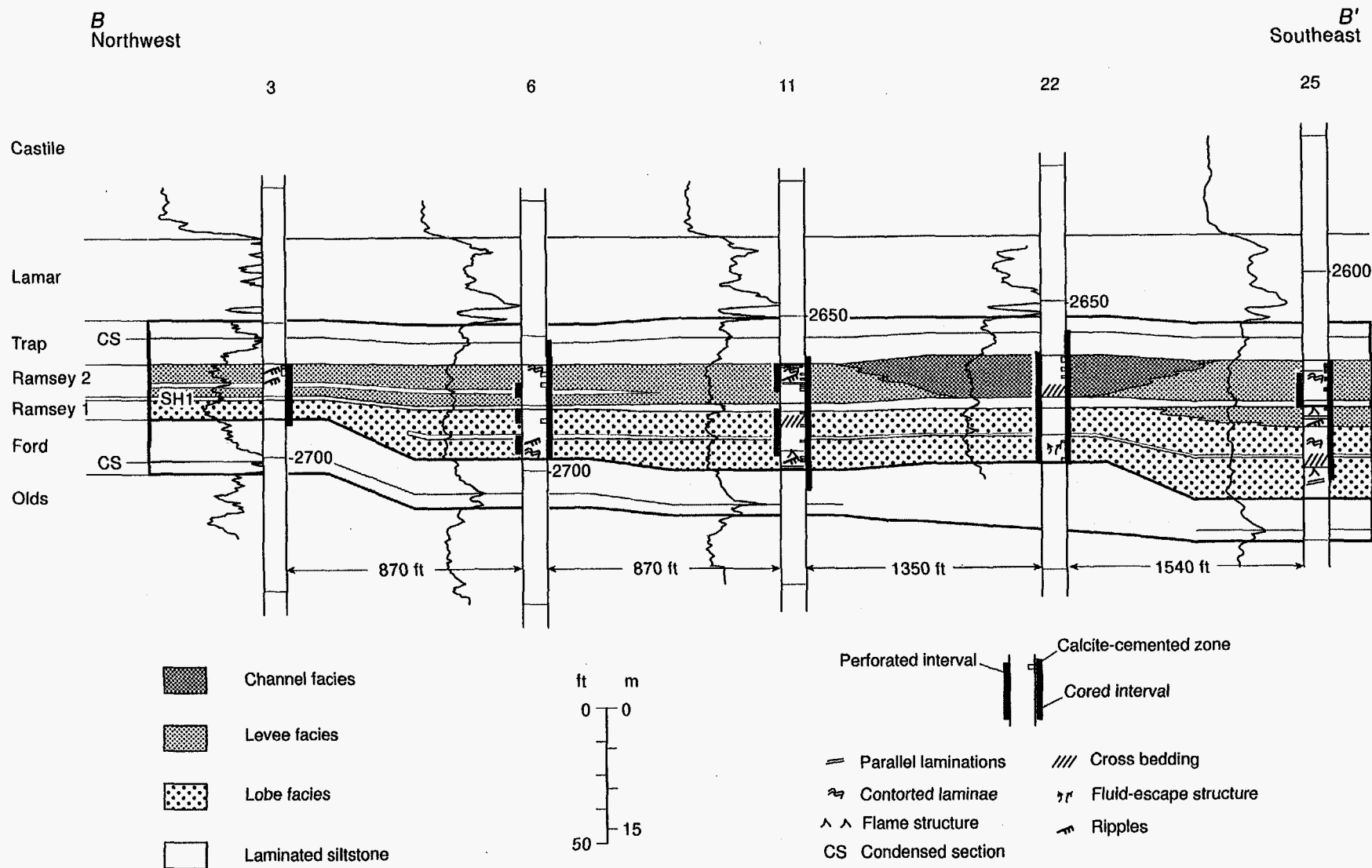
Figure 26. Cross section B-B' through the northern end of Geraldine Ford field, where the SH1 laminated siltstone separates the reservoir into Ramsey 1 and Ramsey 2 sandstones. Deposition of Ramsey sandstones is interpreted to have occurred by sandy high- and low-density turbidity currents that carried a narrow range of sediment size, mostly very fine sand to coarse silt. On the basis of core descriptions and study of the outcrop analog, Ramsey sandstones are interpreted to have been deposited on the basin floor in a sand-rich, channel-levee system with attached lobes. Location of cross section is shown in figure 2.
