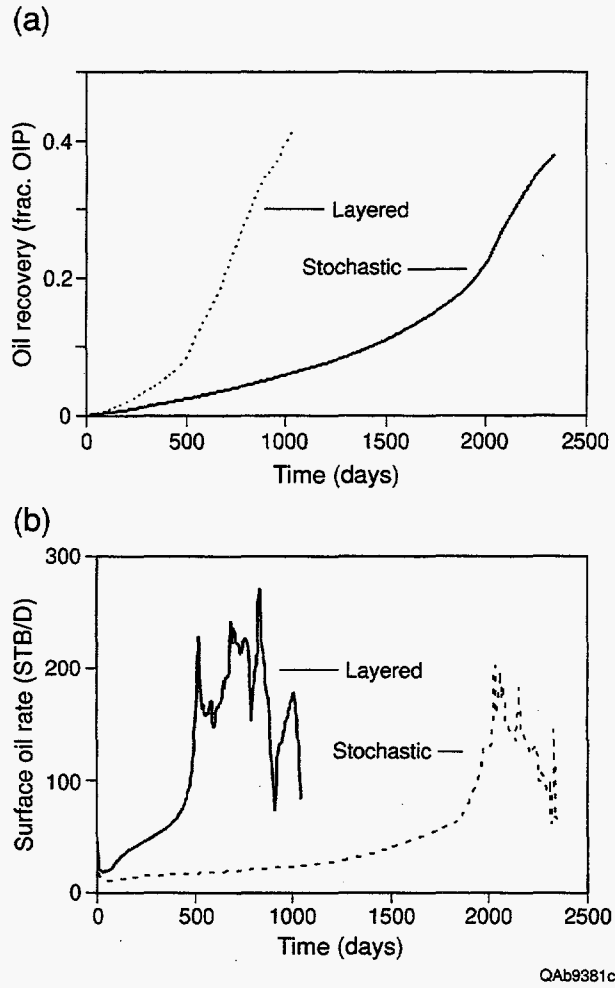
Figure 52. Results of simulation of a CO 2 flood in a quarter five-spot injection pattern in the demonstration area. (a) Oil recovery as a fraction of remaining oil in place. (b) Surface oil production rates.
