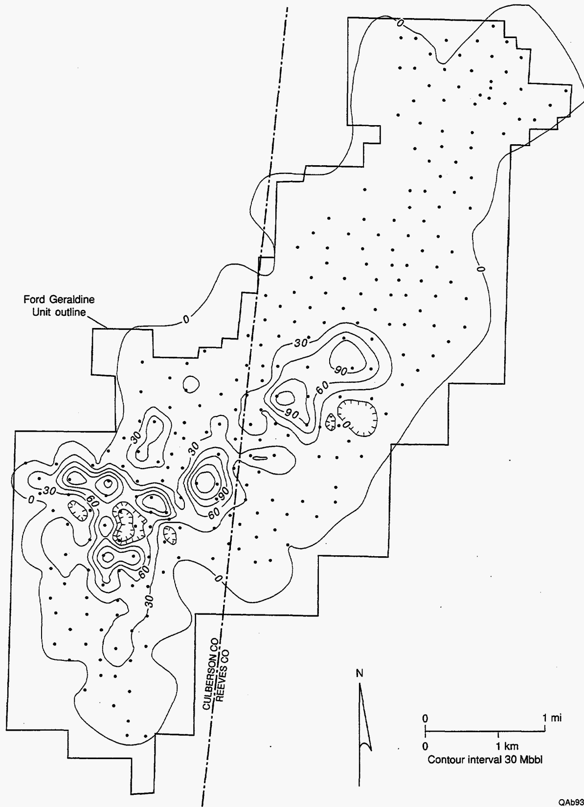
Figure 39. Map of secondary production resulting from the waterflood conducted from 1969 to 1980. Only minor water injection was done in the Stage 5 area (shown in fig. 4) at the northern end of the field.
