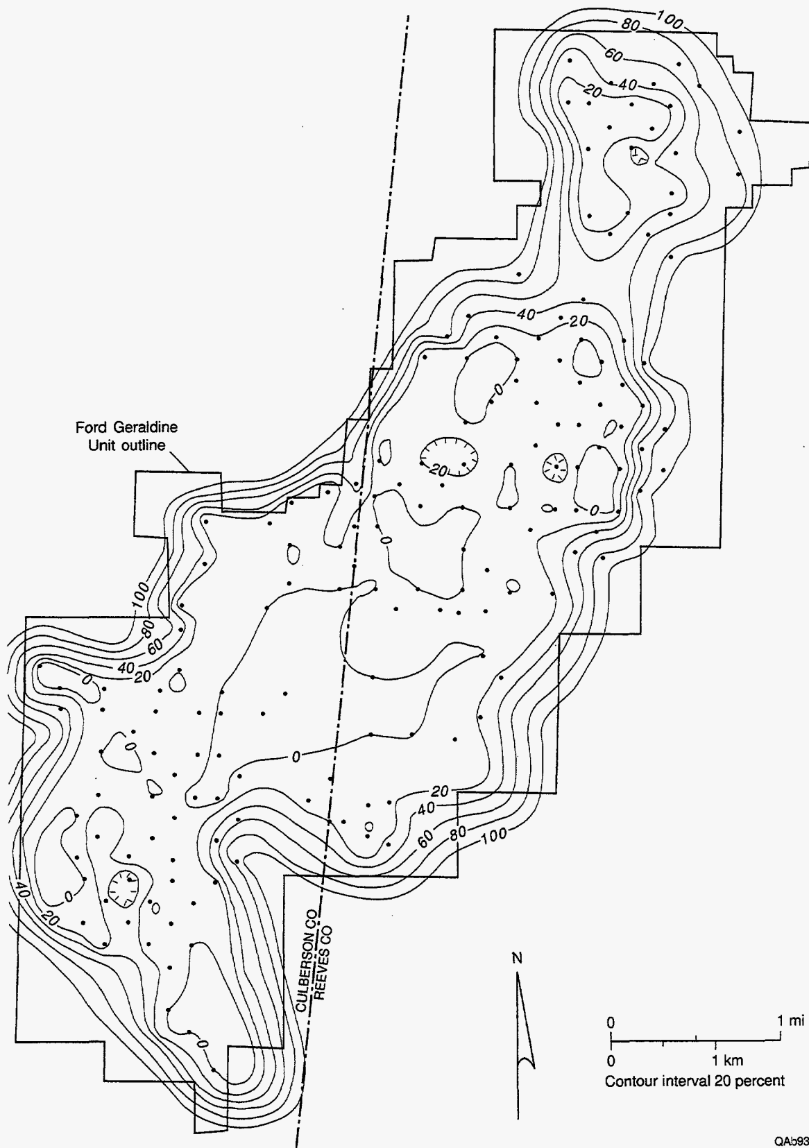
Figure 42. Map of the percentage of water (water cut) produced during initial potential (IP) tests.
