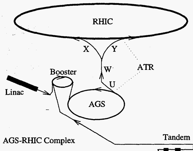
Figure 1: Schematic layout of the AGS-RHIC complex.
