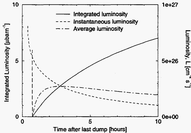
Figure 7: Integrated, instantaneous, and average luminosities during a nominal store of gold ions.
