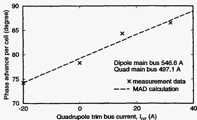
Figure 6: The horizontal phase advance per cell.
