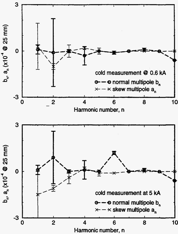
Figure 4: Arc dipole magnetic field multipole harmonics at injection (0.6 kA) and storage (5 kA) currents.
