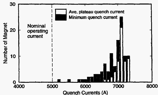
Figure 3: Arc dipole quench current distribution.
