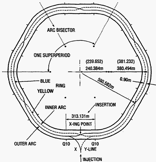
Figure 2: Layout of the collider and the tunnel.
