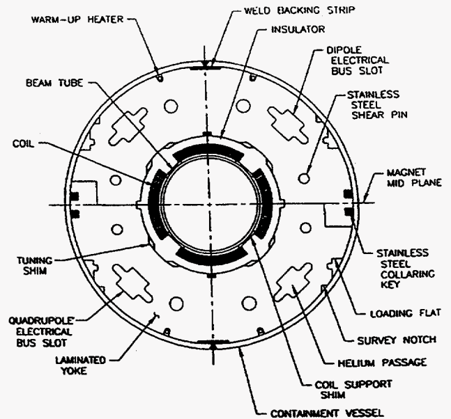
Figure 5: Triplet quadrupole cross-section showing empty slots for tuning shims.
