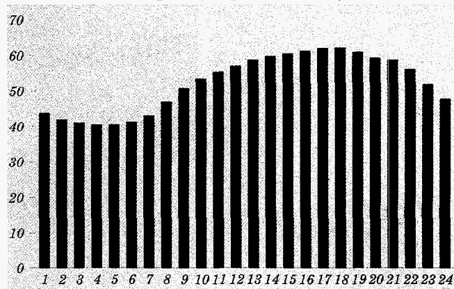
Figure 9. Hourly load curve for the South Atlantic region (megawatthours)
