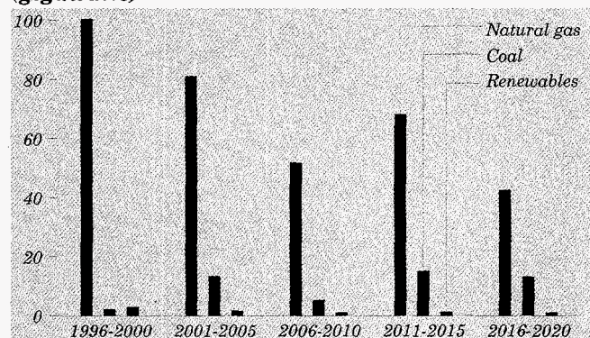
Figure 57. Electricity generation and cogeneration capacity additions by fuel type, 1996-2020 (gigawatts)
