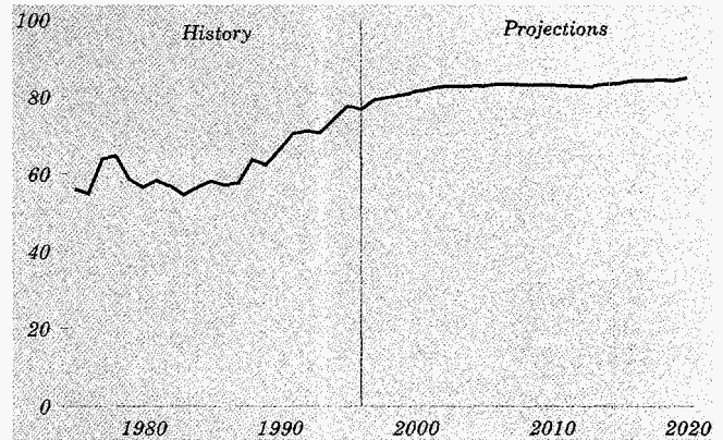
Figure 63. Nuclear power plant capacity factors, 1975-2020 (percent)
