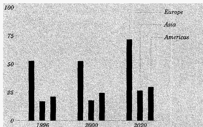
Figure 104. U.S. coal exports by destination, 1996, 2000, and 2020 (million short tons)
