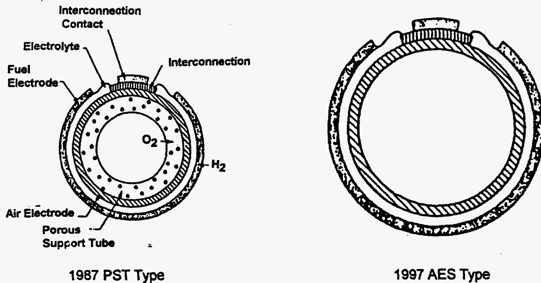
Fig. 1. Tubular SOFC Design Evolution.
