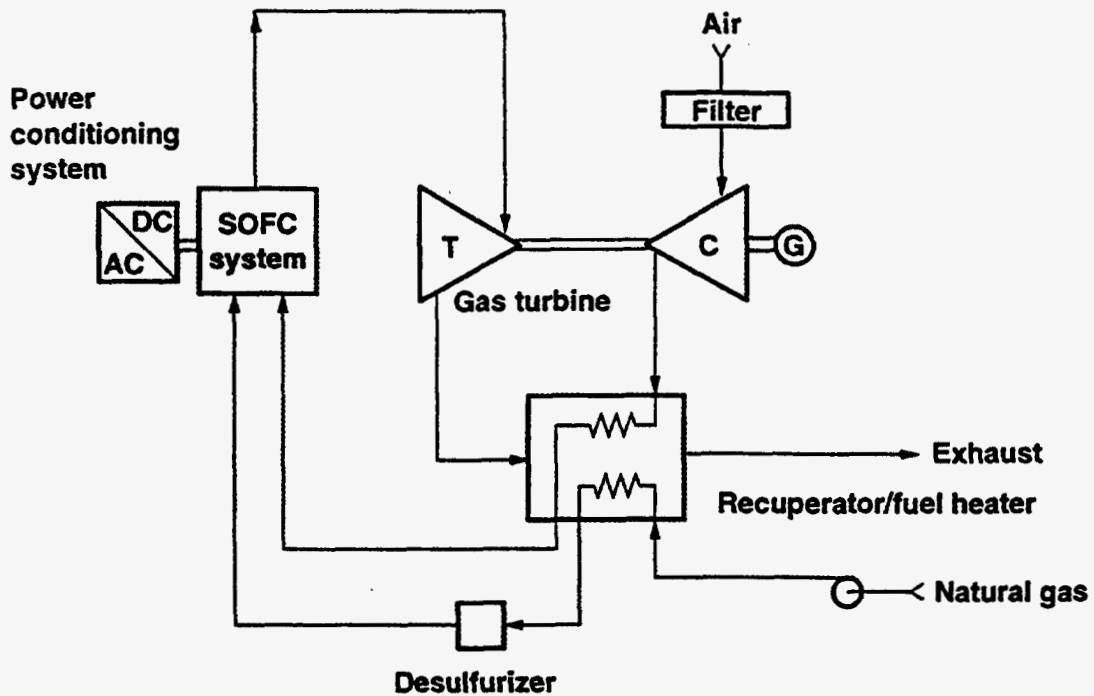
Fig. 2. 3 MWe PSOFC/GT Power System Schematic
