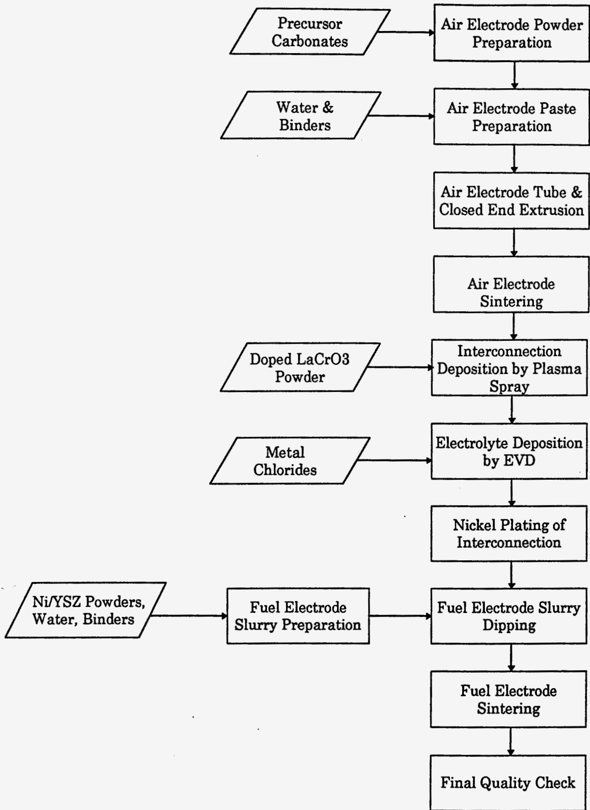
Fig. 3 SOFC Process Flow Diagram.
