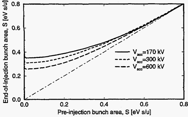
Figure 1: Growth in bunch area of a gold beam due to intra-beam scattering during the initial 2-minute injection period.
