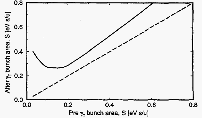
Figure 2: Growth in bunch area of a gold beam at transition in the presence of a \gamma_T jump of \pm 0.4 units in 60 ms. The rf voltage is chosen to be 300 kV, minimizing both chromatic nonlinear effects and beam loading.
