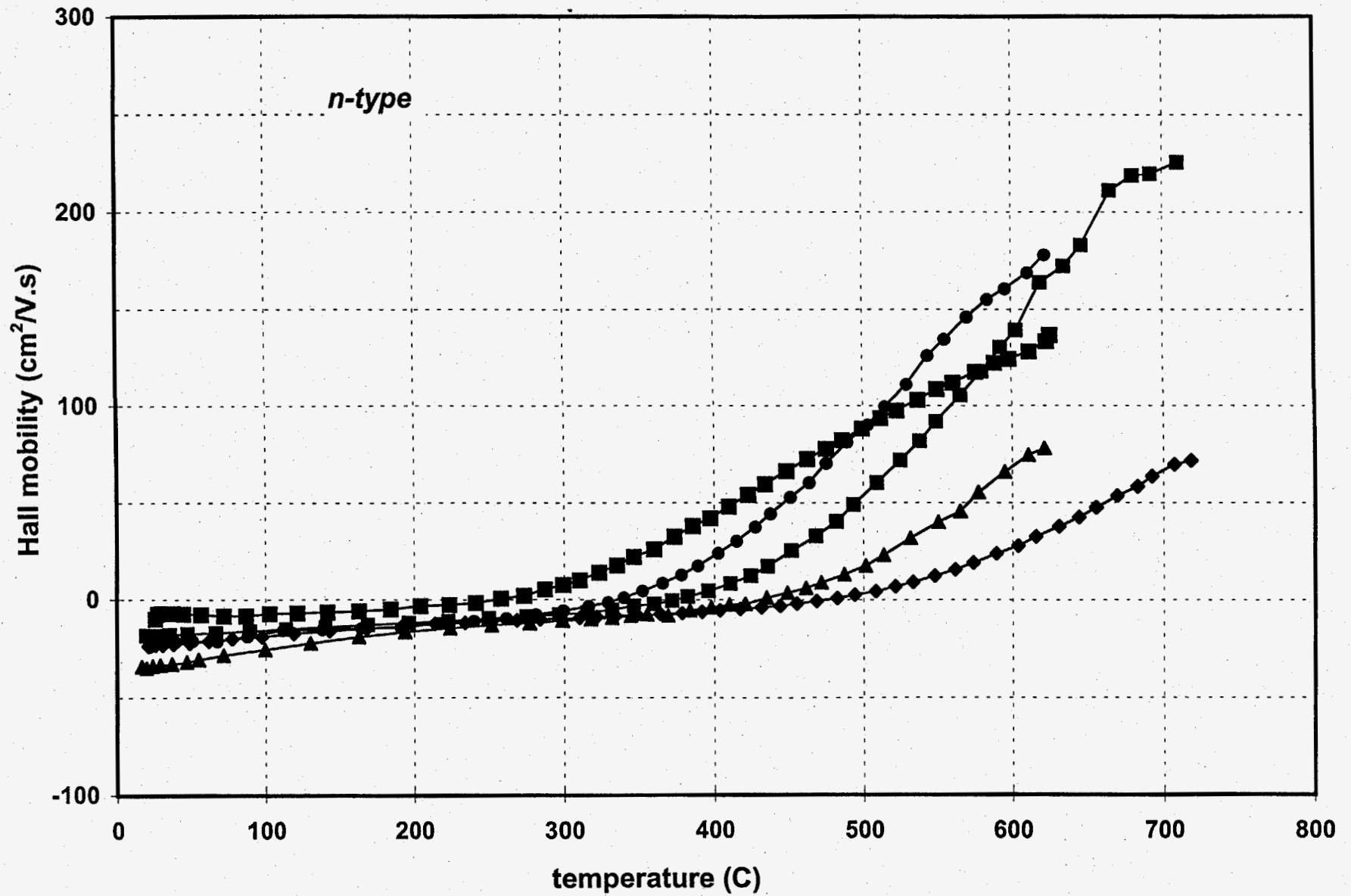
Figure 4: Hall mobility as a function of temperature for n-type IrSb3
