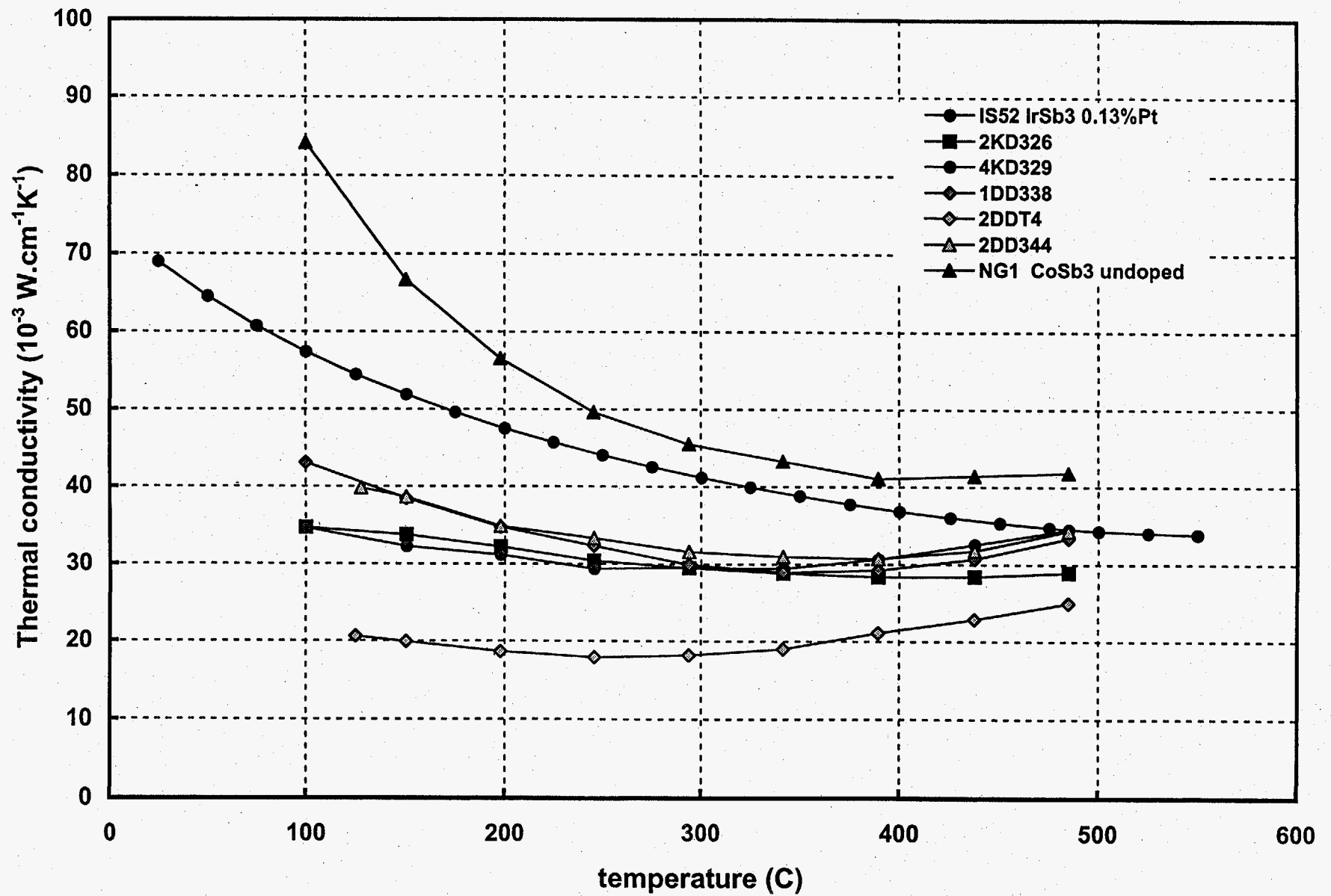
Figure 21: Thermal conductivity as a function of temperature for n-type Cosb3-Irsb3 solid solutions
