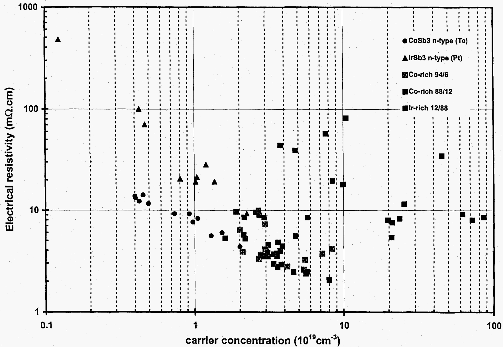
Figure 14: Room temperature electrical resistivity as a function of carrier concentration for n-type CoSb 3 , IrSb 3 and several Co x Ir 1-x Sb 3 solid solutions
