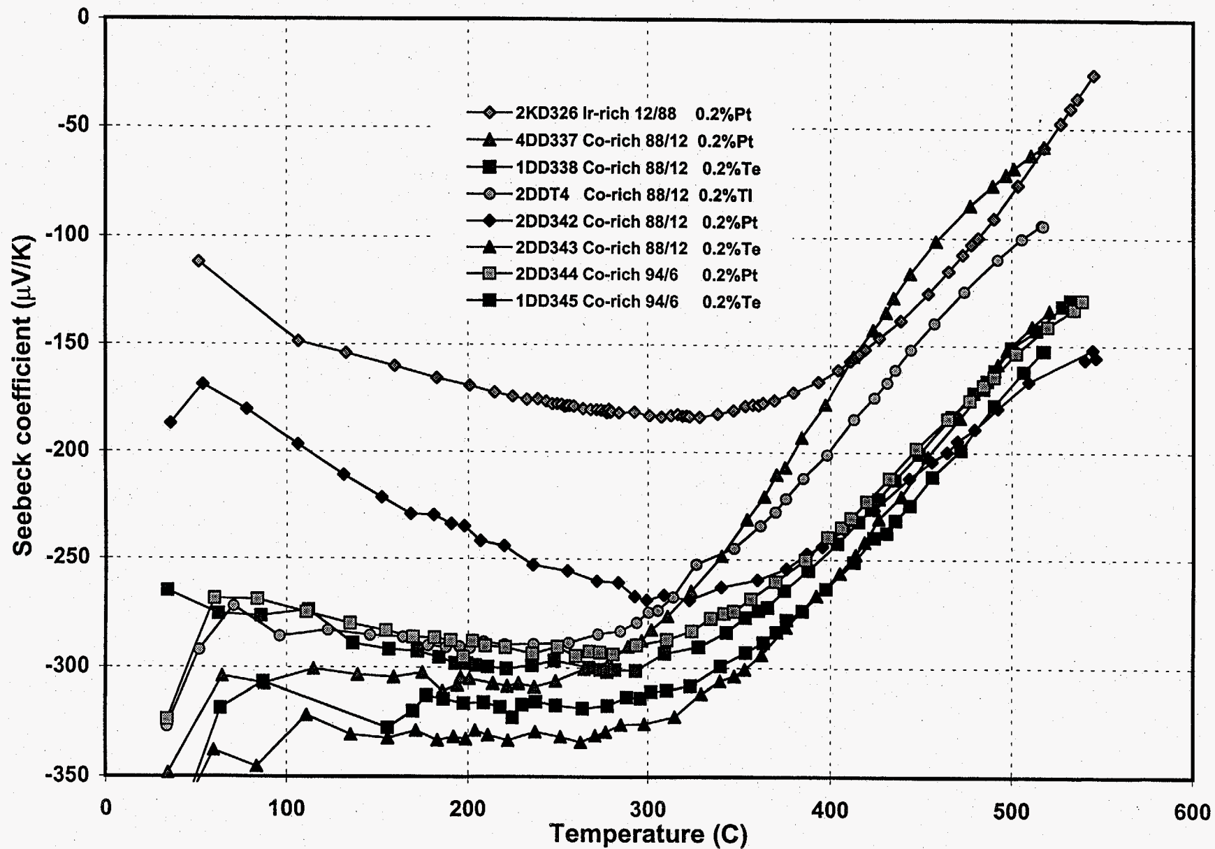
Figure 19: Seebeck coefficient as a function of temperature for several n-type \text{CoSb}_3\text{-IrSb}_3 solid solutions
