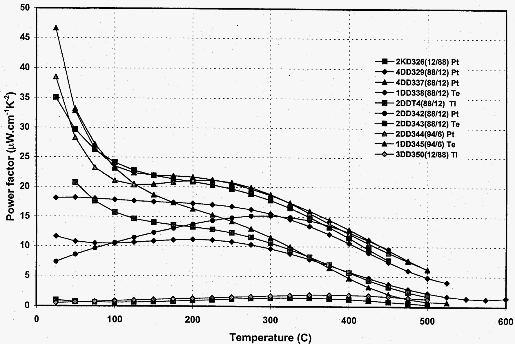
Figure 20: Power factor as a function of temperature for n-type \text{CoSb}_3\text{-IrSb}_3 solid solutions
