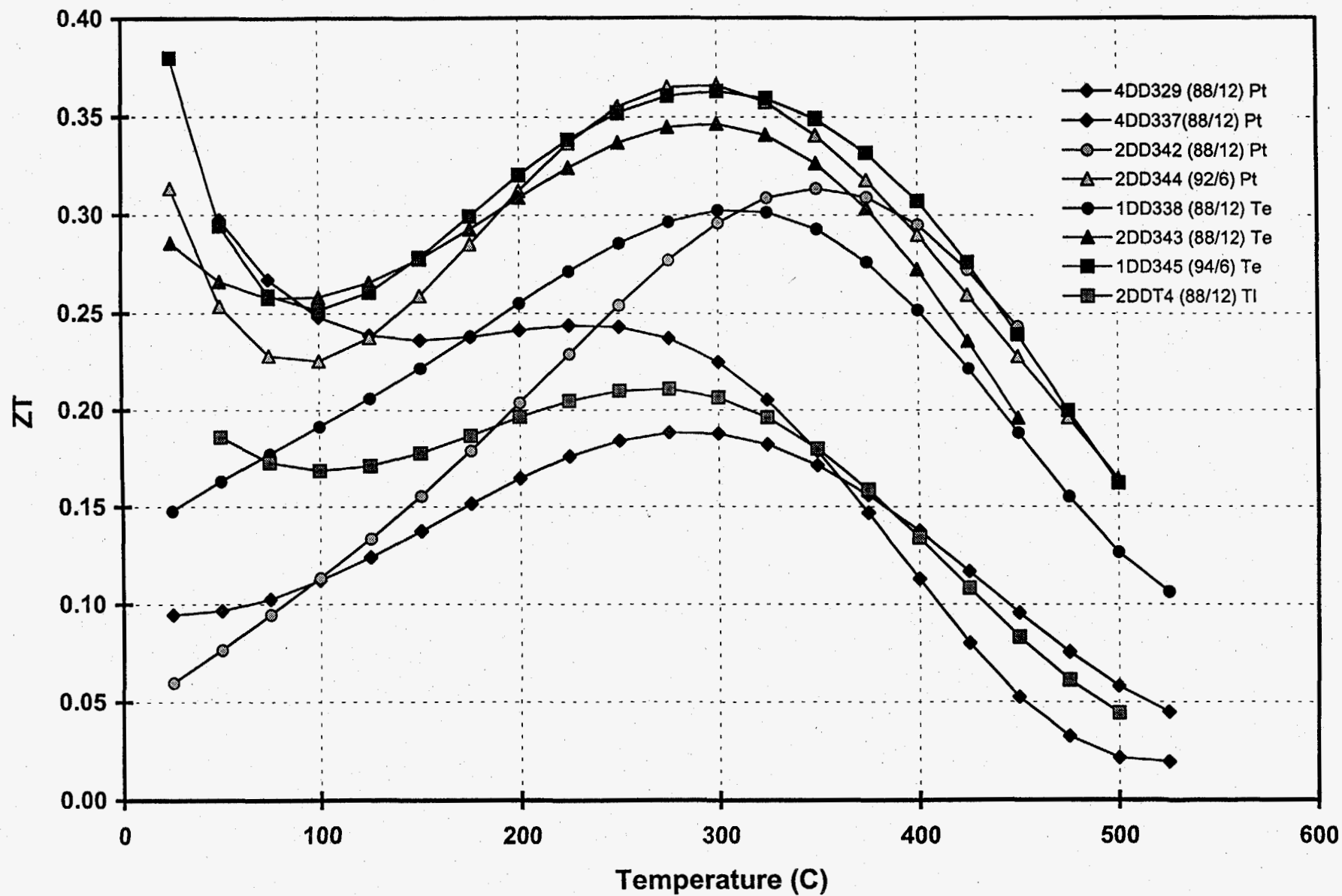
Figure 22: ZT as a function of temperature for n-type CoSb 3 -IrSb 3 solid solutions
