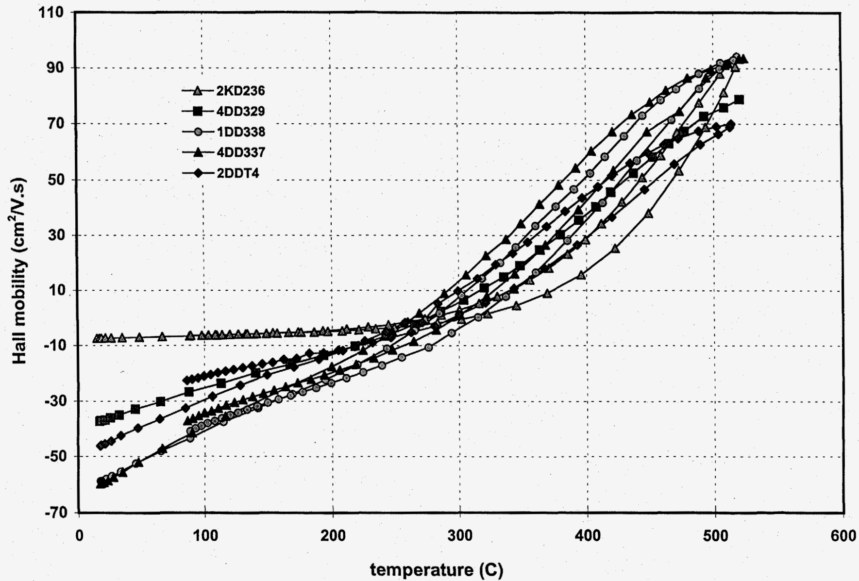
Figure 18: Hall mobility as a function of temperature for n-type \text{Cosb}_3\text{-IrSb}_3 solid solutions
