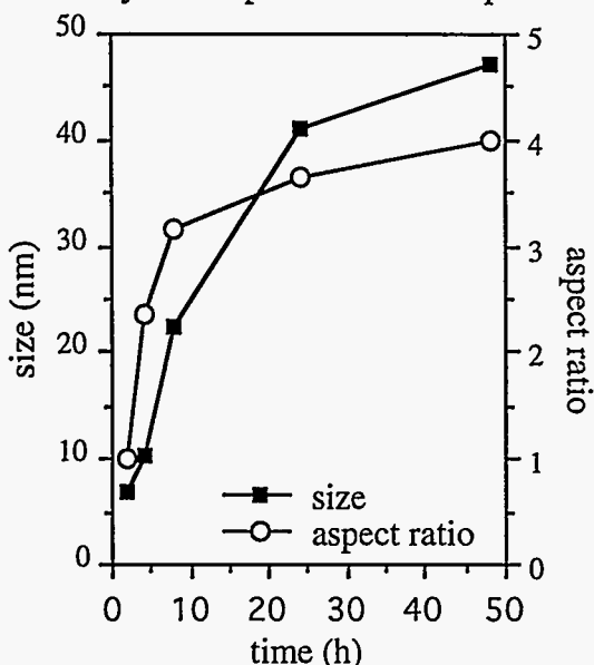
Figure 6: Evolution of particle size and aspect ratio with respect to heat treatment (250°C) time. Particle size data is also included in figure 3. The starting suspensions were 0.05 M Fe^{+3} (from nano-g sol) and 0.05 M Ba(OH)_2 adjusted to a pH of 13.1 using sodium hydroxide. These were then placed into a 250°C furnace for various times.
