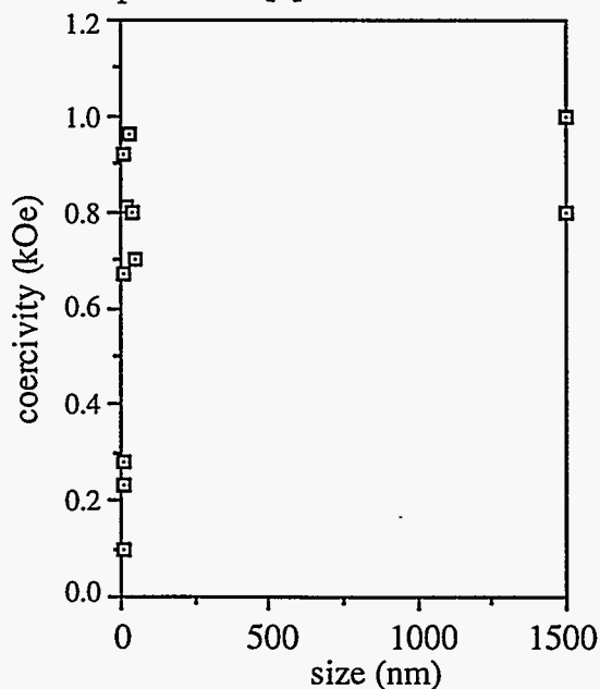
Figure 9: Coercivity versus BHF particle size.
