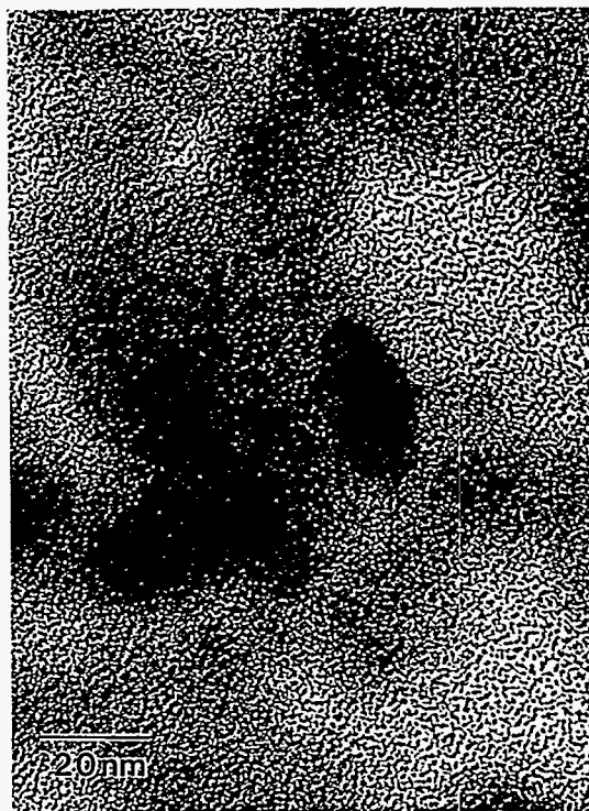
Figure 4: TEM micrograph of nanocrystalline BHF particles (average particle size = 8.6 nm). These particles were produced from a 0.025M \text{Fe}^{+3} (from nano-g precursor) and 0.025 M \text{Ba}(\text{OH})_2 suspension heat treated at 250°C for two hours.
