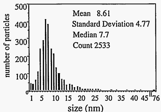
Figure 2: Typical particle size distribution for BHF particles produced in this study. Synthesis conditions for this sample were 0.025 M \text{Fe}^{+3} (from nano-g) and 0.025 M \text{Ba}(\text{OH})_2 suspension heat treated at 250°C for two hours.
