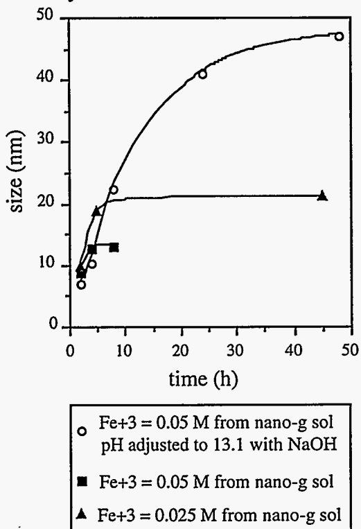
Figure 3: Evolution of particle size with respect to time. Suspensions were prepared and placed in a 250°C furnace for various times. \text{Ba}^{+2} : \text{Fe}^{+3} ratio is equal to one in all cases.
