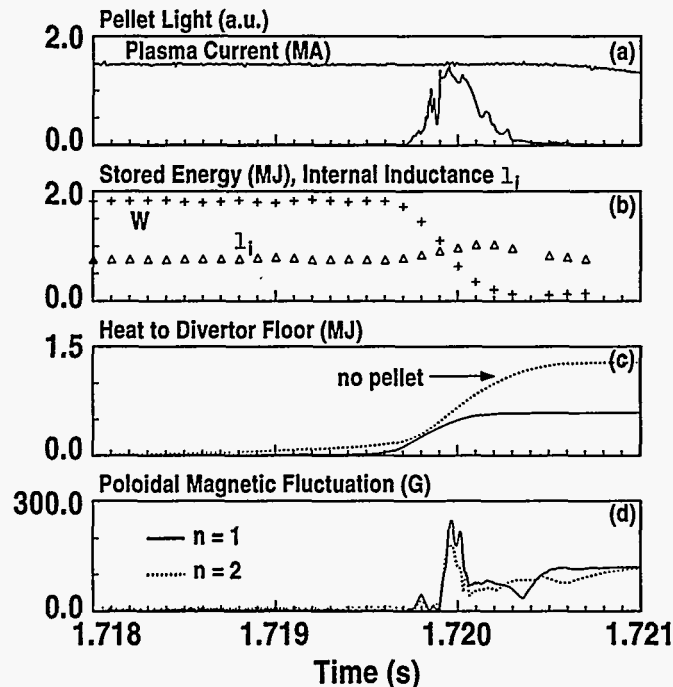
Fig. 3. Argon pellet injection into a VDE ( \beta_n=3.2 , q=3.4 , shot 90206) causes an immediate loss of stored energy and rapidly initiates the current quench. The heat conducted to the floor is reduced by 50% with the injection of a pellet. Large MHD activity develops within 250 \mu s of pellet injection.
