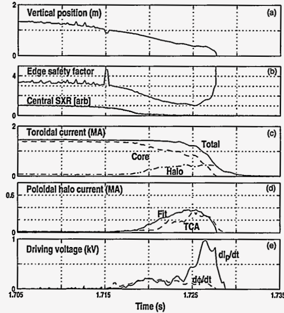
Fig. 1. Time evolution of a VDE ( \beta_n=1.1 , shot 90219). Poloidal halo current reaches 370 kA (23% of the pre-disruption I_p ). The peak poloidal halo current determined by a magnetic fitting code (FIT) agrees well with that measured by the tile current array (TCA).
