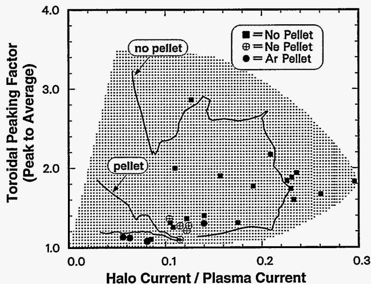
Fig. 2. Toroidal peaking factor and halo current normalized to the pre-disruption plasma current for VDEs. Points show the values at the time of peak halo current. The two solid lines show the trajectory of a pellet and non-pellet discharge with identical pre-disruption equilibria. The shaded region is the boundary of the trajectories of all discharges.
