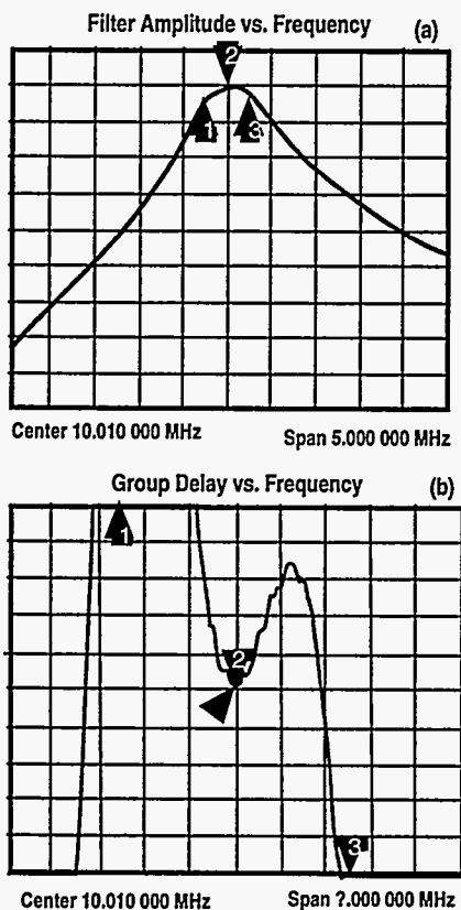
Fig. 3. IF filter amplitude and group delay.
