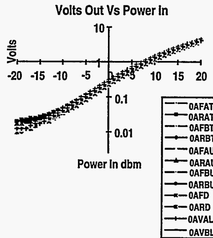
Fig. 4. Amplitude detector voltage out vs. power in.
