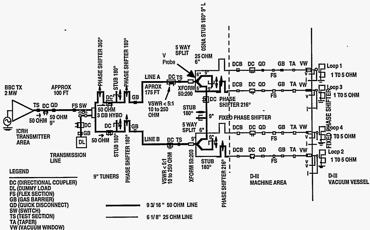
Fig. 1. DIII-D transmission line and antenna tuners
