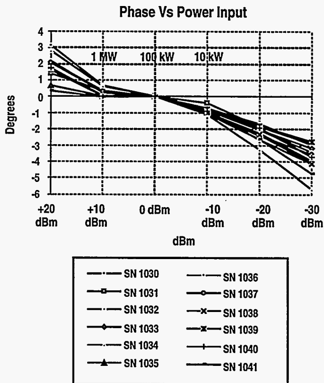
Fig. 5. phase detector accuracy vs input level.
