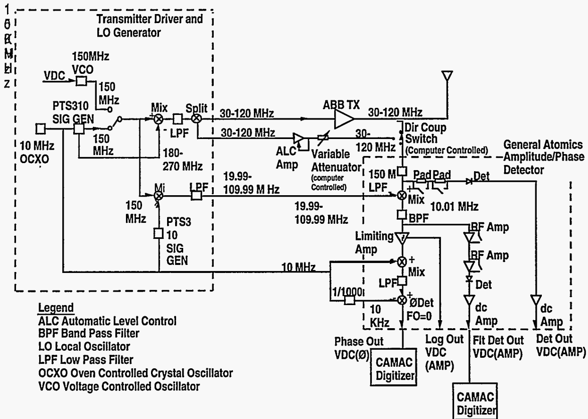
Fig. 2. DIII-D fast wave current drive amplitude and phase detection
