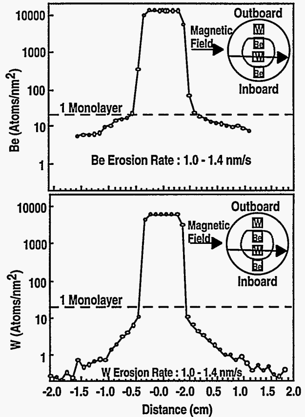
Fig. 7. Areal density profiles for Be and W after exposure to an ELM-free H-mode with a peak heat flux of 0.8 \text{ MW/m}^2 , electron temperature of 70 eV, and magnetic field grazing incidence of 1.5^\circ .
