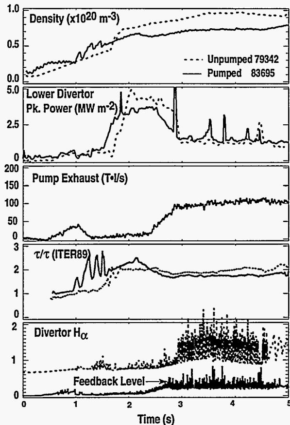
Fig. 4. Effective heat flux reduction to the divertor and particle control have been achieved with D_2 puffing and the use of the cryopump. The pumped (solid) discharge has a lower core density than the unpumped (dash). The gas flow was controlled by the photodiode signal.
