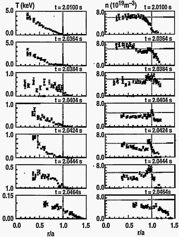
Fig. 6. T_e and n_e profiles versus normalized radius for a disruption induced by argon injection. The plasma edge (separatrix) is shown by the vertical dotted line. The horizontal lines on the density plots are the line average density measured along a midplane radial chord. The thermal quench starts at 2.035 s and ends at 2.045 s. There is a brief reheating period from 2.039 s to 2.044 s.
