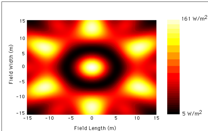
Figure 15. Acoustic Intensity Versus Location Produced 6x10 kW sources that CoherentlySum for a Maximima at the Center of the Array in domain of 30m x 30m; Attenuation Factor for this AER Simulator is 0.2 db/m Comparable to a Ground Water Hydrogeologic Condition
