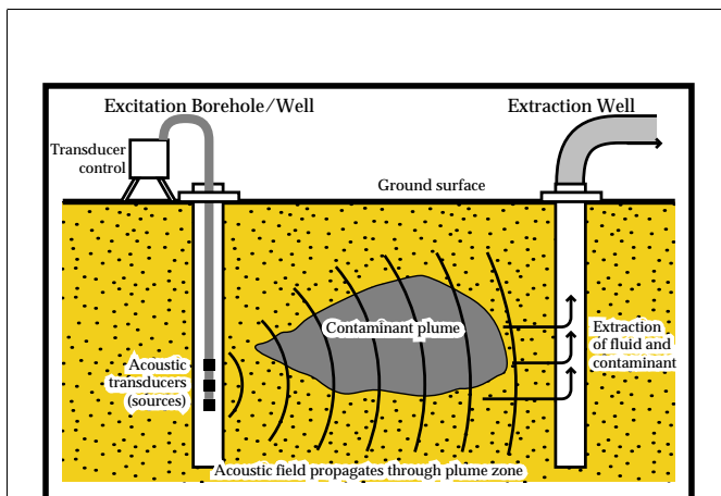
Figure 5. The Acoustically Enhanced Remediation Field Deployment Concept
