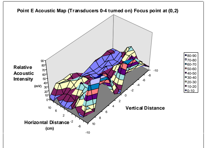
Figure 11. Experiment-1 Relative Acoustic Intensity for Focal Point (0,2); Point E is Approximately 2.4' Below the Injection Point in Figure 9
