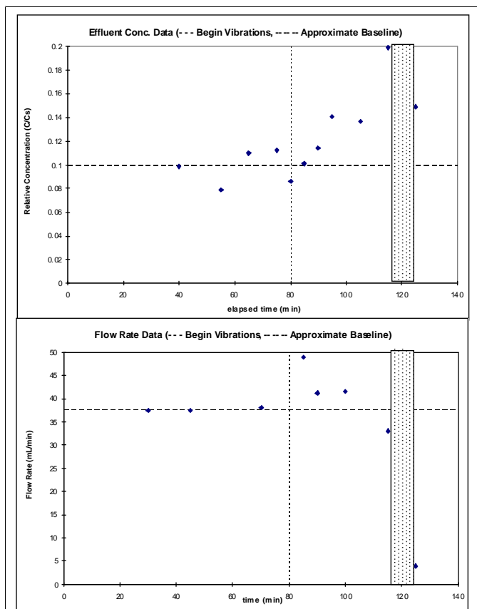
Figure 13. Dissolution Test P-Xylene Concentrations and Test Cell Flow Rates; Shaded Region Indicates Fines Plugging the Flow System Filters
