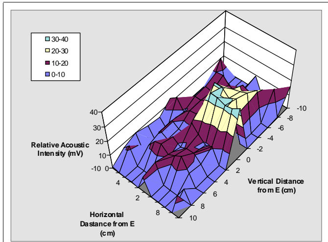
Figure 10. Experiment-1 Relative Acoustic Intensity for Focal Point (0,0); Point E is Approximately 2.4' Below the Injection Point in Figure 9
