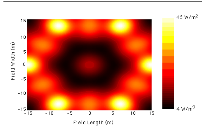
Figure 16. Acoustic Intensity Versus Location Produced 6x10 kW sources that CoherentlySum for a Maximima at the Center of the Array in domain of 30m x 30m; Attenuation Factor for this AER Simulator is 1.0 db/m Comparable to a Ground Water Hydrogeologic Condition
