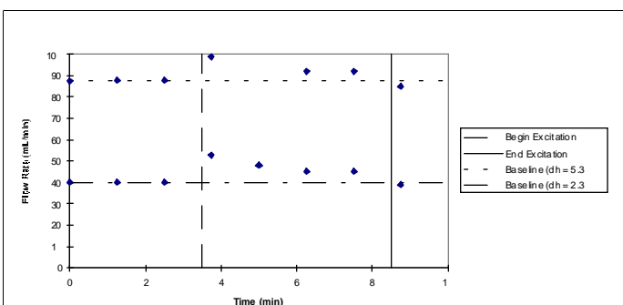
Figure 12. Dissolution Test Cell Hydraulic Conductivity Results
