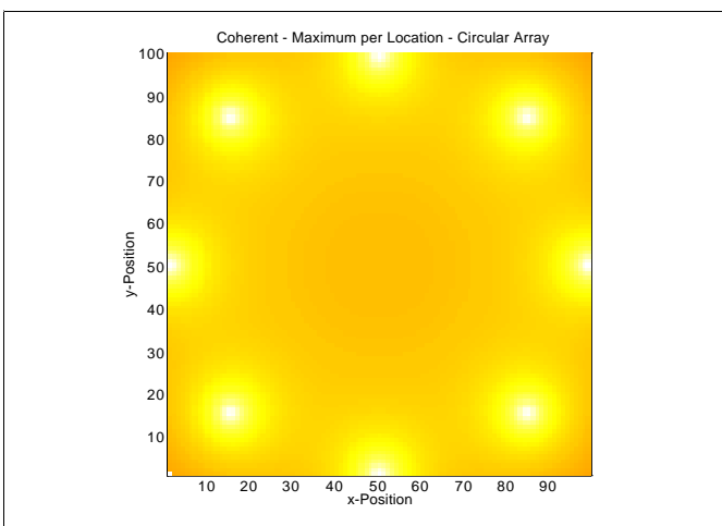
Figure 4. Acoustic Maximum Intensity Versus Location Produced by Sweeping (or Beam Steering) Eight Phase Tuned Sources Across the Volume; domain in meters
