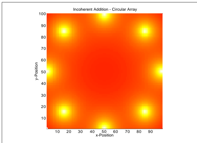
Figure 3. Acoustic Maximum Intensity Versus Location Produced by Eight Sources that Incoherently Sum; domain in meters
