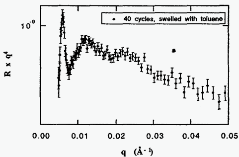
Figure 2b. Reflectivity for sample with 40 cycles, swelled with toluene.
