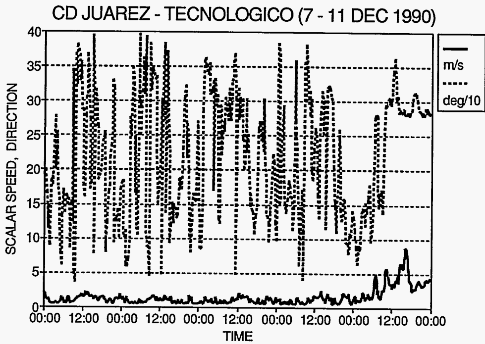
Figure 19 Wind speed and direction for December 7-11 at the Tecnologico site.
