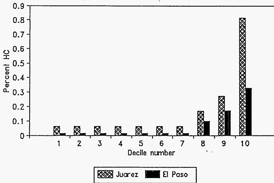
Figure 12 Decile emissions for HC in %propane for vehicles measured in El Paso and Cd. Juarez [from Stedman, 1993B].
