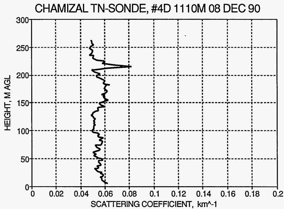
Figure 27 Scattering coefficient profiles during 1045-1110 hours on December 8 at the Chamizal site.
