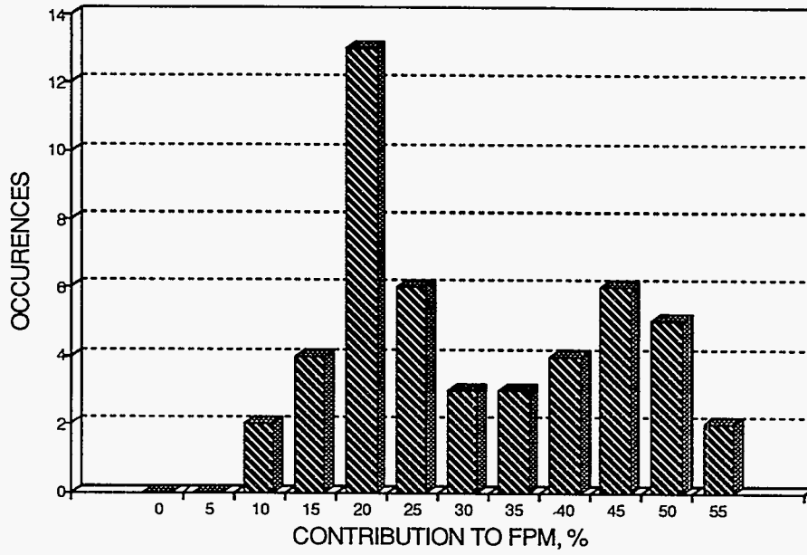
Figure 55 Estimates of vehicular source contribution to FPM for all sites and sampling periods.
