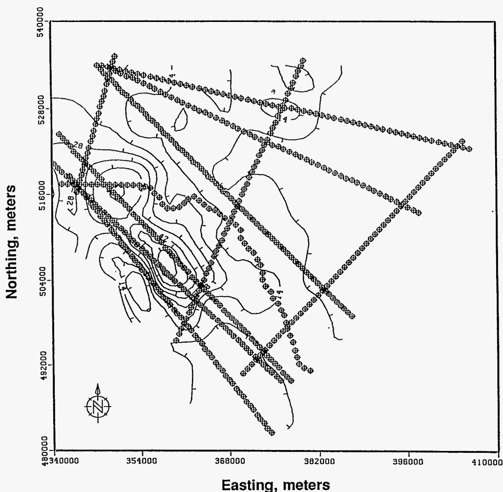
Figure 8 A graph showing airborne flight tracks (circles) on the morning of February 23 with near ground-level aerosol backscatter intensity, interpolated from the lidar data, shown as contour lines [from McElroy, 1990].
