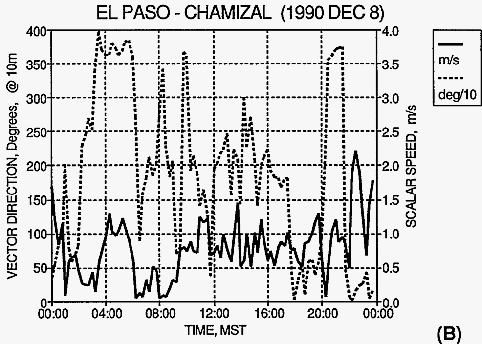
Figure 21 Temperature/humidity (A) and wind speed/wind direction (B) for December 8 at the Chamizal site.
