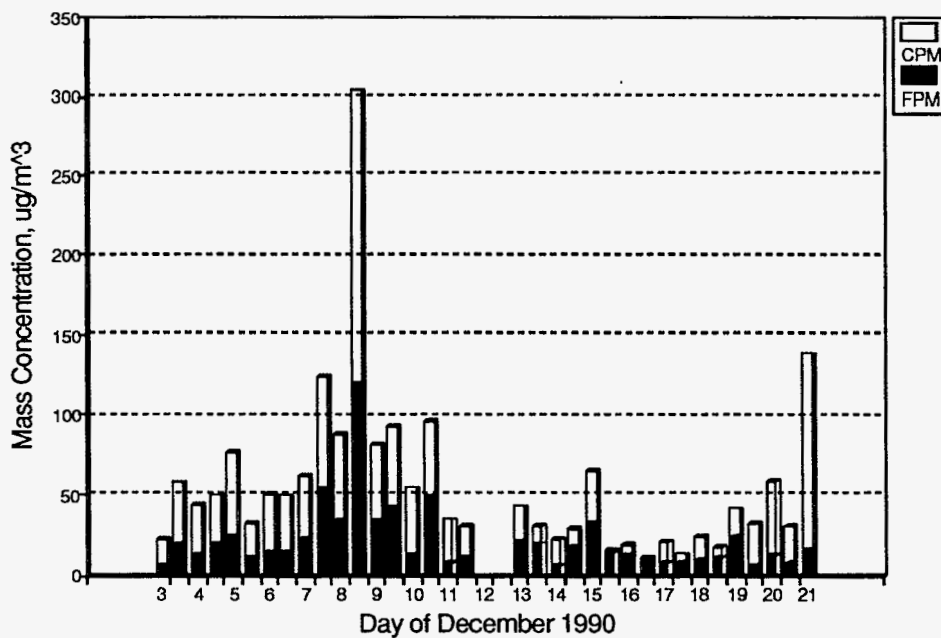
Figure 39 A stacked barplot showing FPM and CPM for all sampling periods at the CAMS6 site [note scale change].
