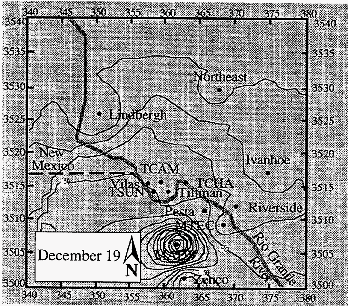
Figure 48 A contour plot showing PM-10 levels interpolated from measurements at 15 sites on December 19 [from Dattner, 1993].
