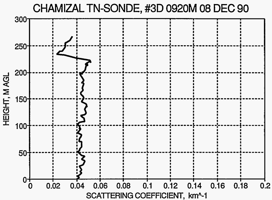
Figure 26 Scattering coefficient profiles during 0805-0920 hours on December 8 at the Chamizal site.
