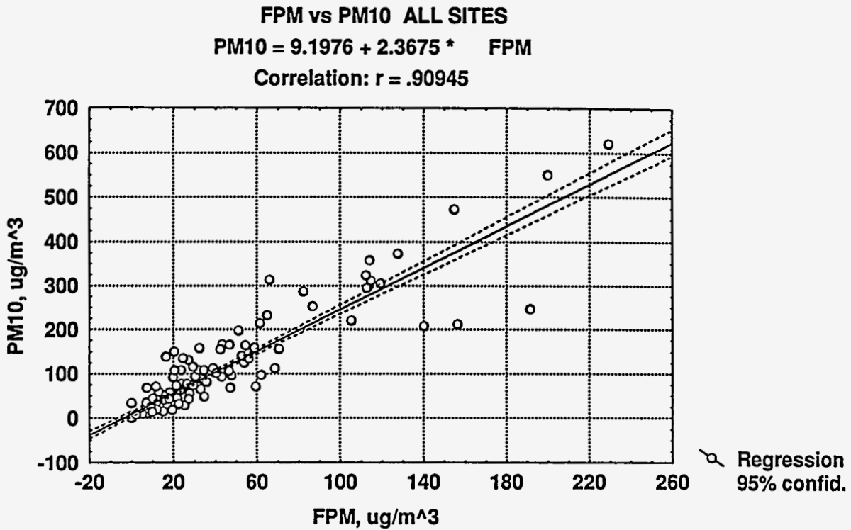
Figure 43 A scatterplot of FPM and PM-10 for all sampling sites and periods.
