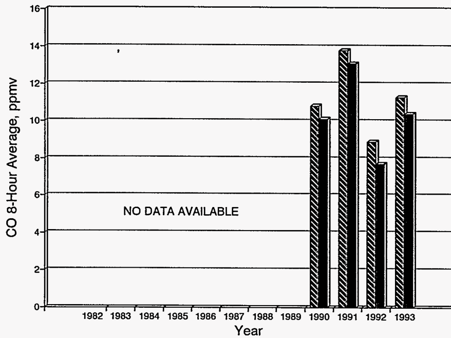
Figure 6 The two highest 8-hour CO averages measured annually at the Cd. Juarez Advance Transformer and Tecnologico sites from 1990 through 1993.
