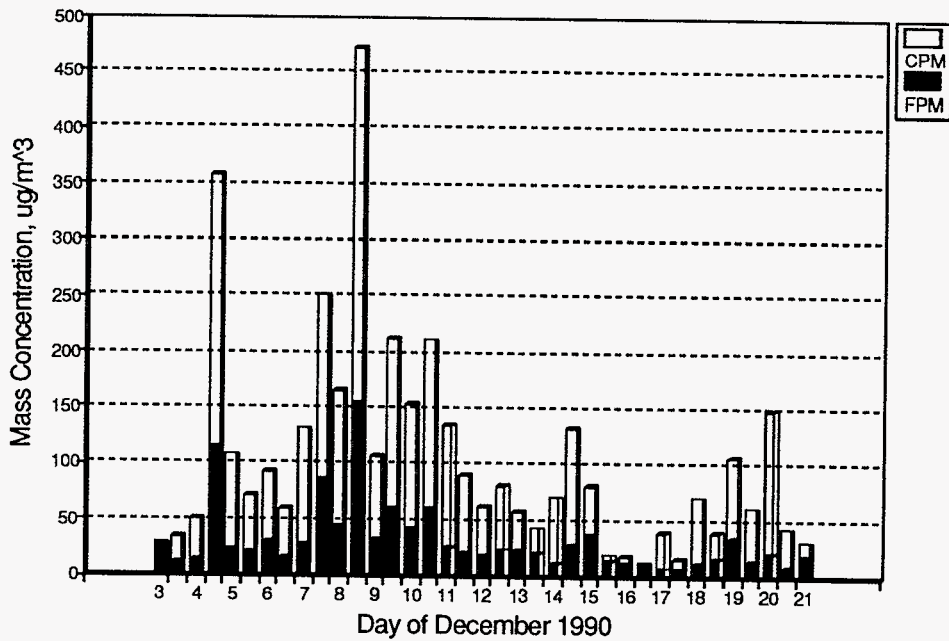
Figure 40 A stacked bar plot showing FPM and CPM for all sampling periods at the Chamizal site.
