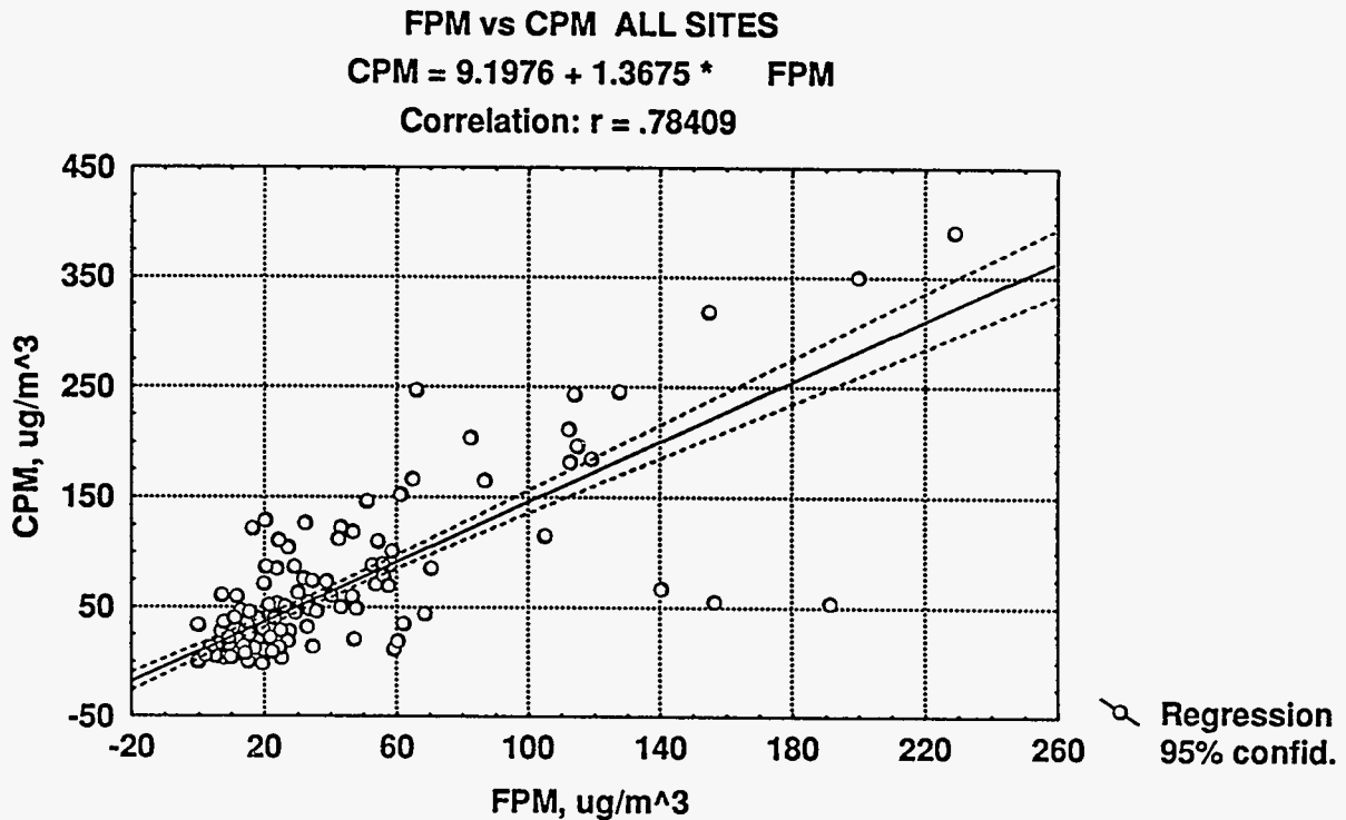
Figure 45 A scatterplot of FPM and CPM for all sampling sites and periods.
