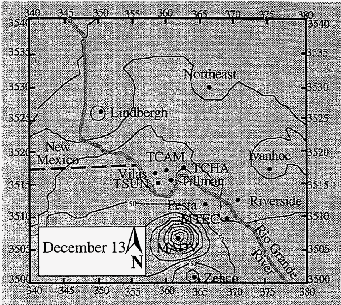
Figure 47 A contour plot showing PM-10 levels interpolated from measurements at 15 sites on December 13 [from Dattner, 1993].
