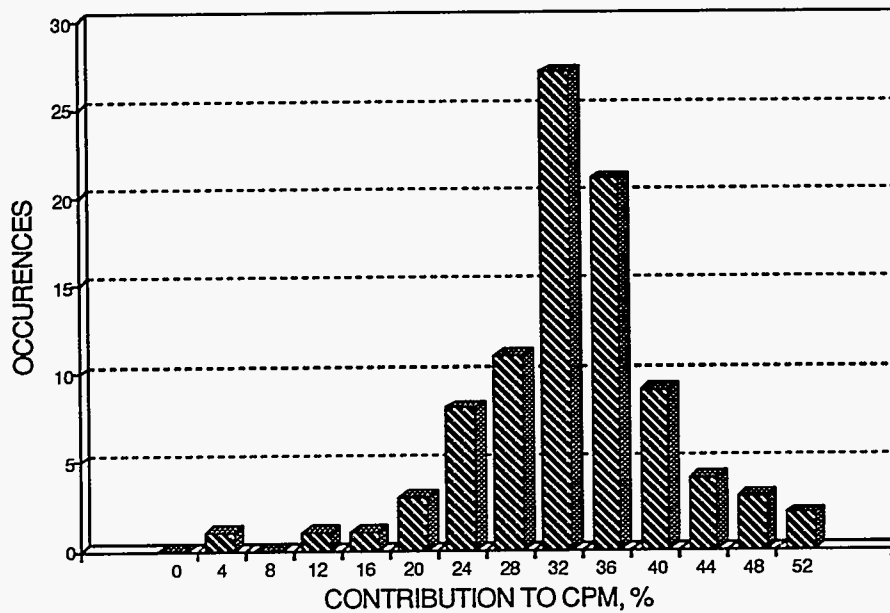
Figure 58 Estimates of biomass combustion source contribution to CPM for all sampling sites and periods.
