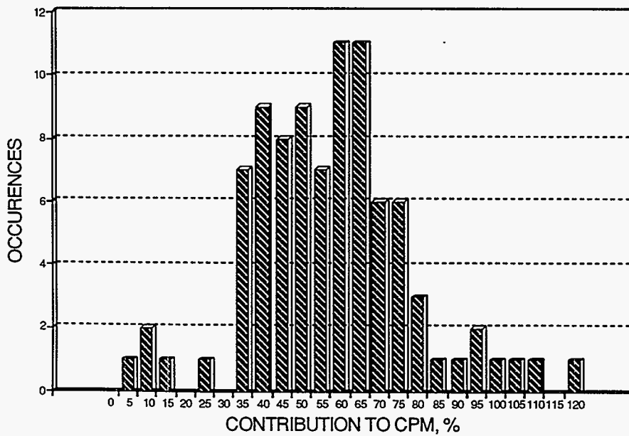
Figure 52 Estimates of crustal source contribution to CPM for all sites and sampling periods.
