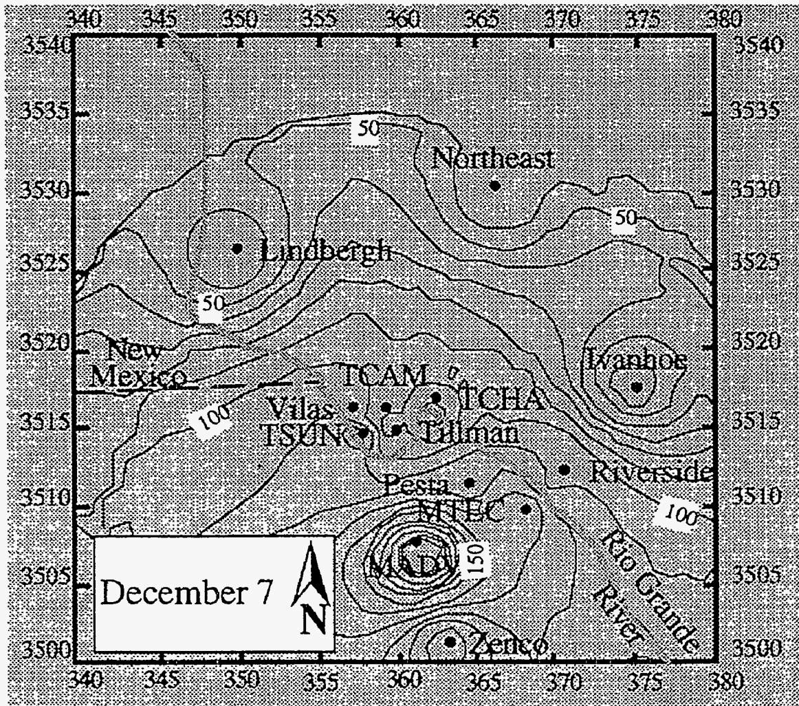
Figure 46 A contour plot of PM-10 levels interpolated from measurements at 15 sites on December 7 [from Dattner, 1993].
