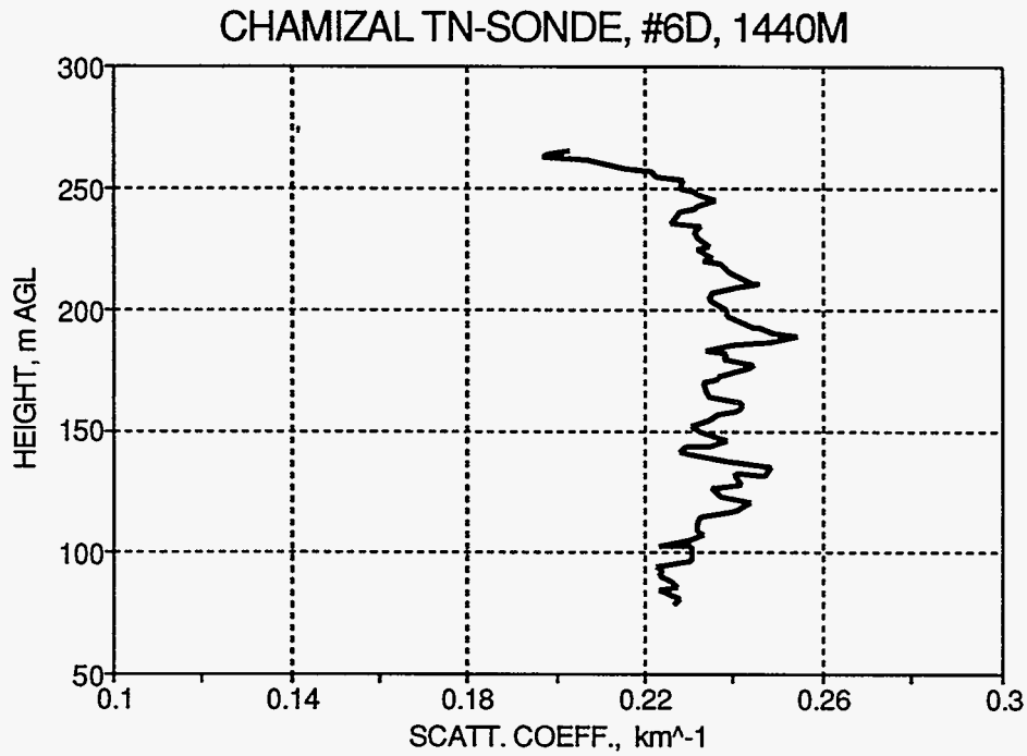
Figure 29 Scattering coefficient profiles during 1408-1440 hours on December 8 at the Chamizal site.
