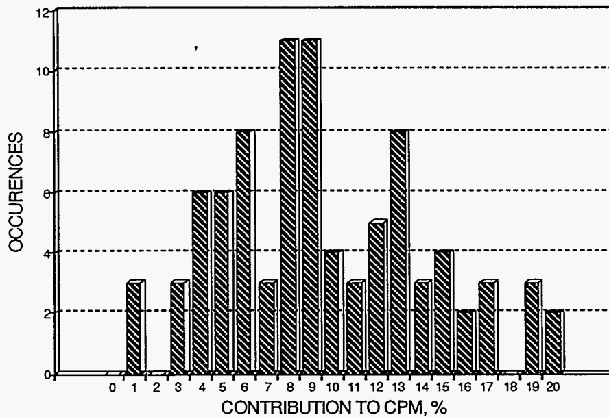
Figure 56 Estimates of the vehicular source contribution to CPM for all sampling sites and periods.
