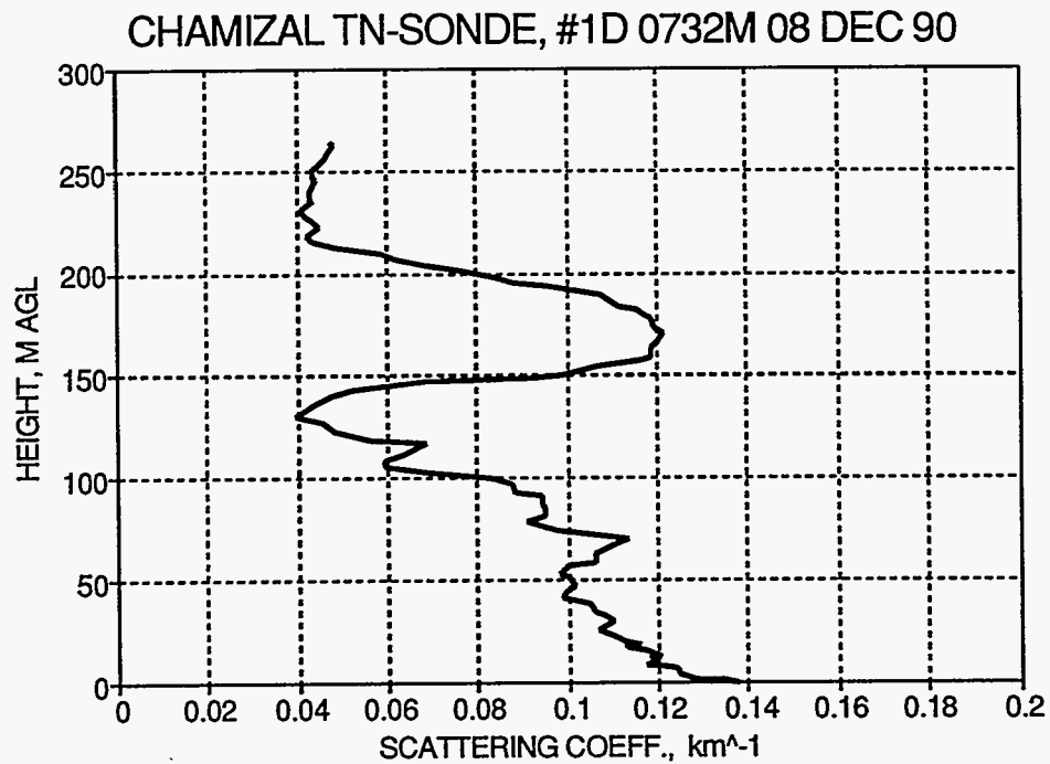
Figure 24 Scattering coefficient profiles during balloon-nephelometer ascent (upper) and descent (lower) during 0708-0732 hours on December 8 at the Chamizal site.
