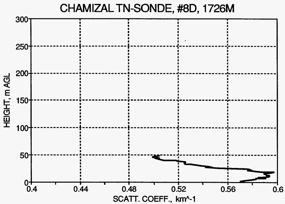
Figure 31 Scattering coefficient profiles during 1718-1726 hours on December 8 at the Chamizal site.
