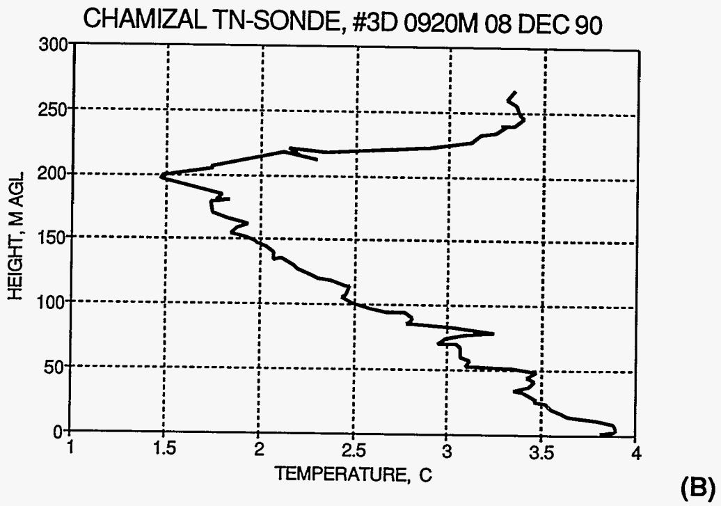
Figure 23 Chamizal temperature sounding data from the morning of December 8 from radiosonde (A) and tethersonde (B).
