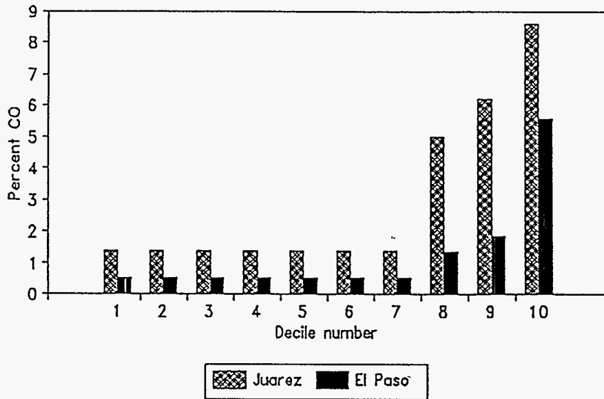
Figure 11 Decile emissions in %CO for vehicles measured in El Paso and Cd. Juarez [from Stedman, 1993B].
