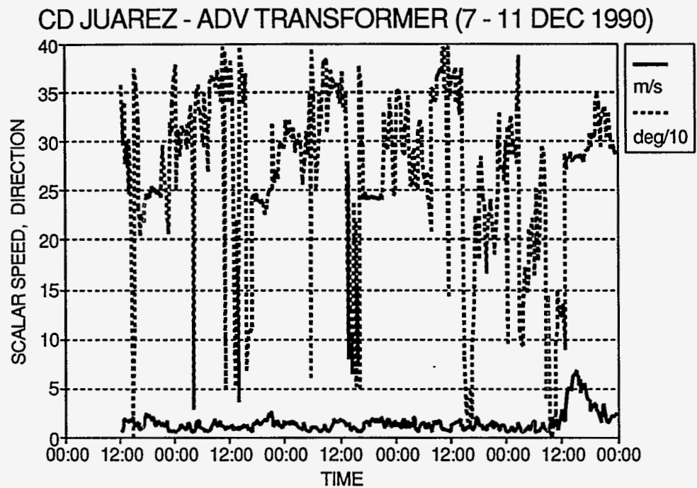
Figure 20 Wind speed and direction for December 7-11 at the Advance Transformer site.
