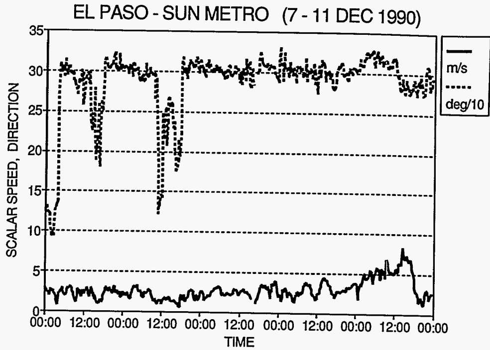
Figure 18 Wind speed and direction for December 7-11 at the Sun Metro site.
