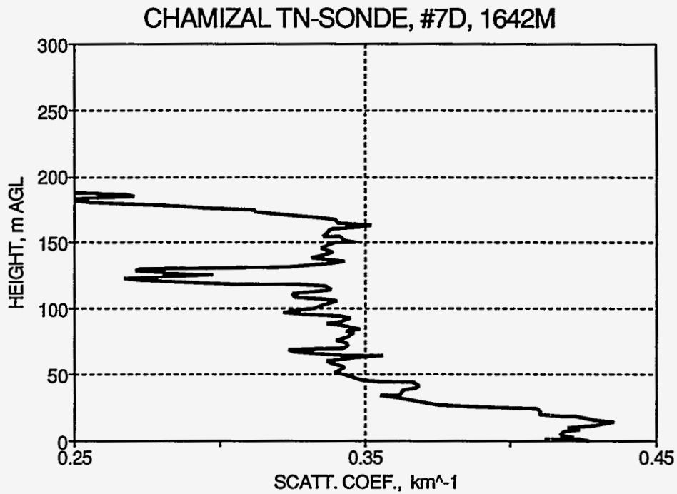
Figure 30 Scattering coefficient profiles during 1615-1642 hours on December 8 at the Chamizal site.
