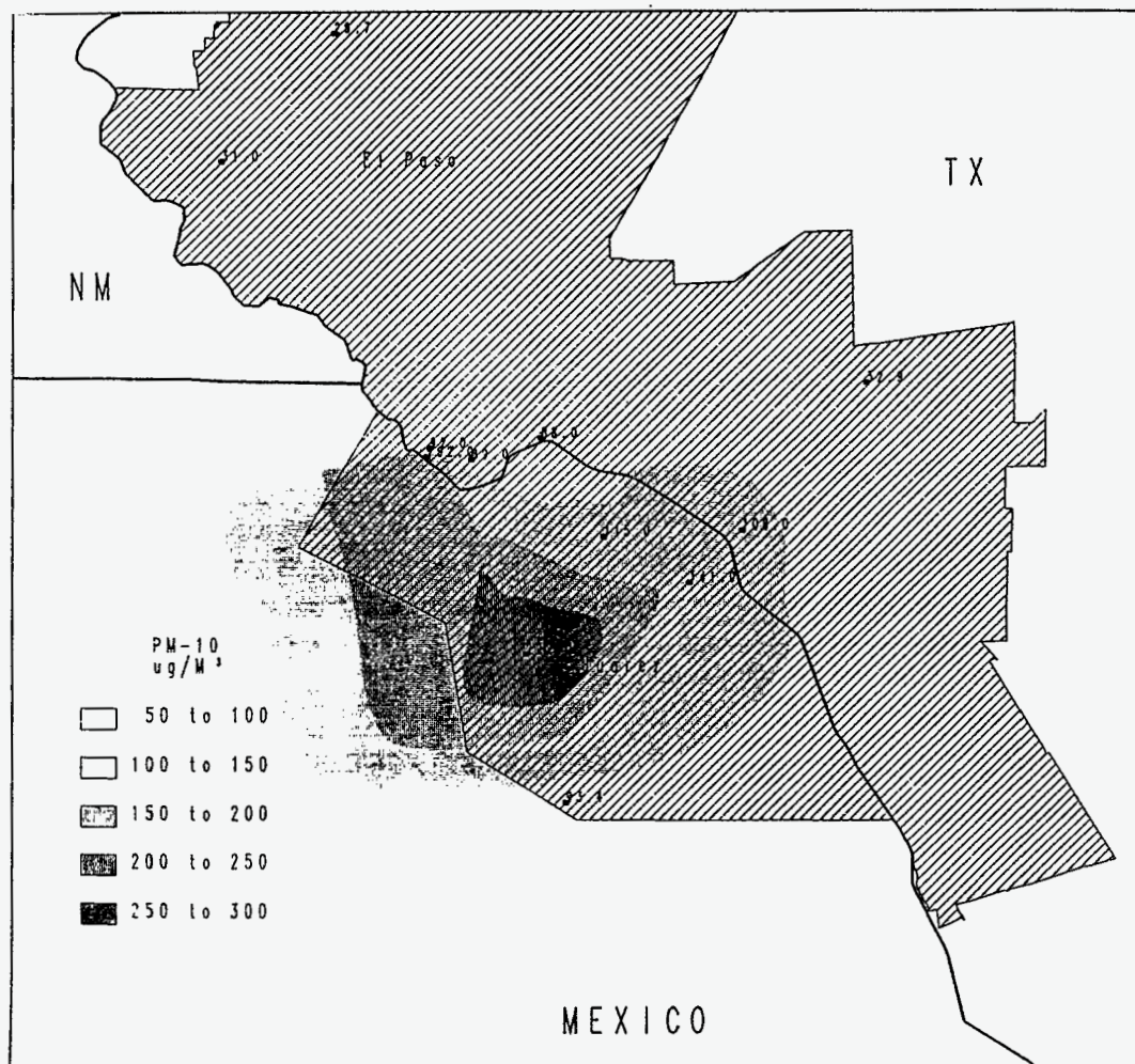
Figure 9 A contour plot showing PM_{10} values interpolated from measurements on December 11, 1989 during the Saturation PM_{10} Study [from Kemp, 1990].
