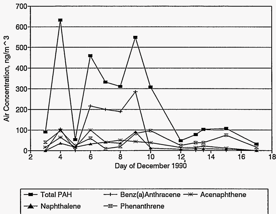
Figure 49 Total polycyclic aromatic hydrocarbon and selected species concentrations measured at the CAMS6 site during a portion of the study interval [from Dattner, 1993].
