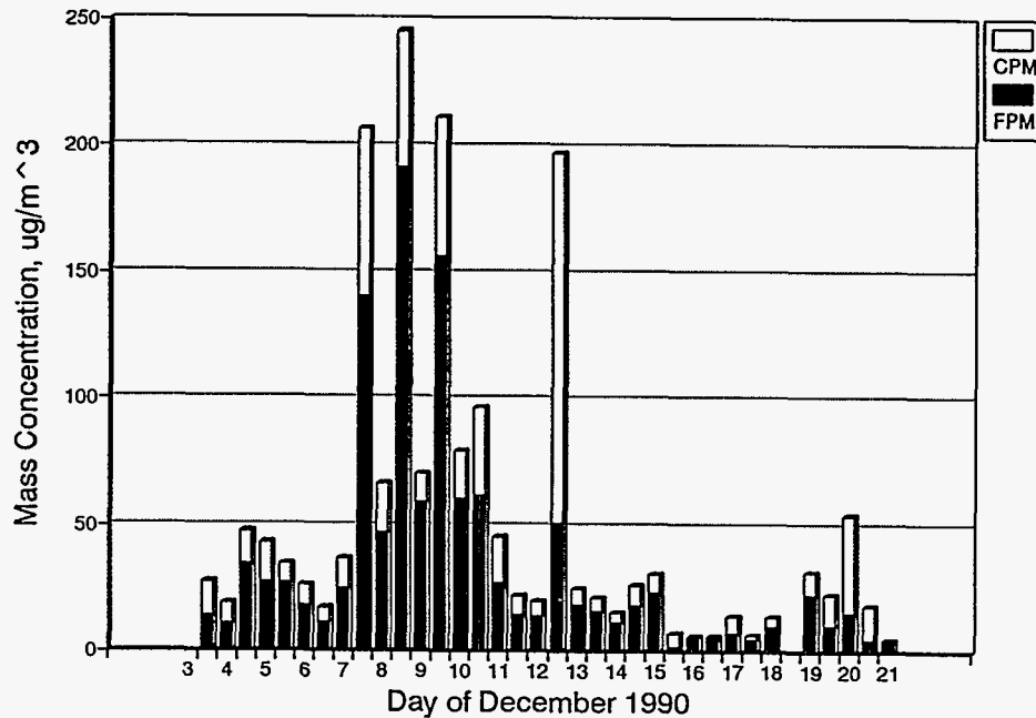
Figure 42 A stacked barplot showing FPM and CPM for all sampling periods at the Tecnologico site.
