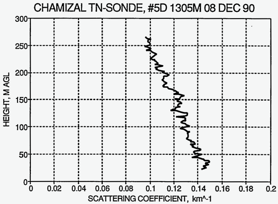
Figure 28 Scattering coefficient profiles during 1235-1305 hours on December 8 at the Chamizal site.
