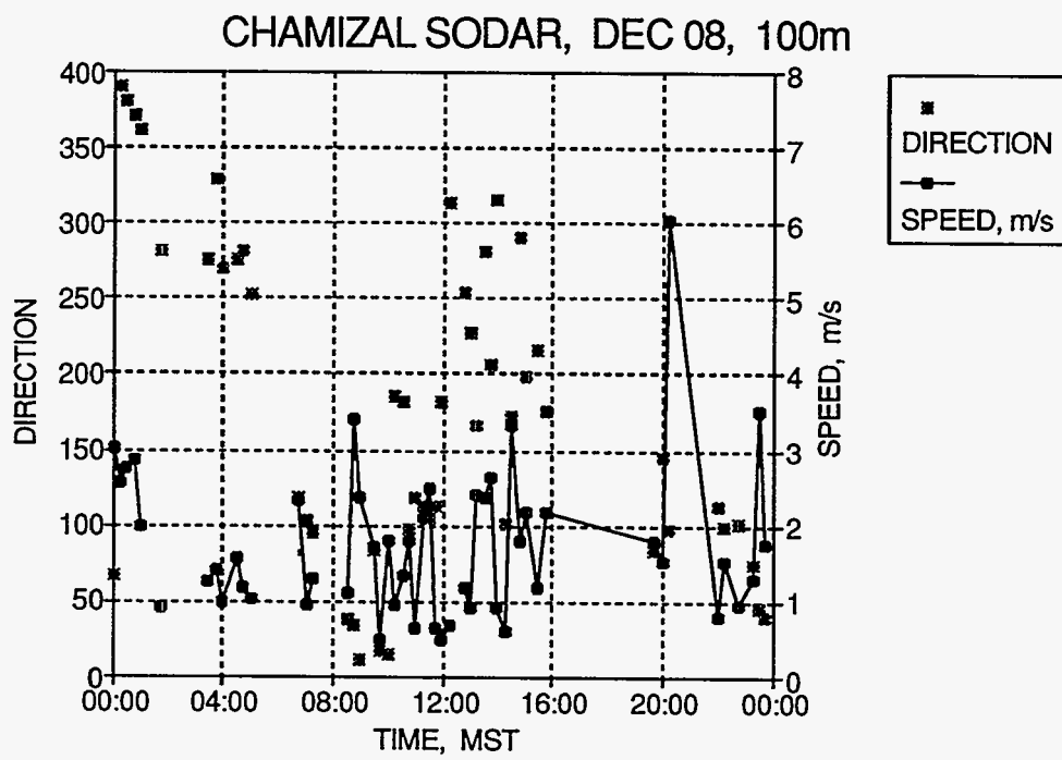
Figure 22 Sodar measured winds on December 8 at the Chamizal site.
