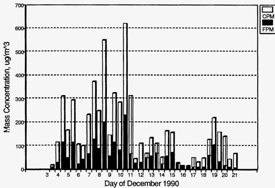
Figure 38 A stacked barplot showing FPM and CPM for all sampling periods at the Advance Transformer site.
