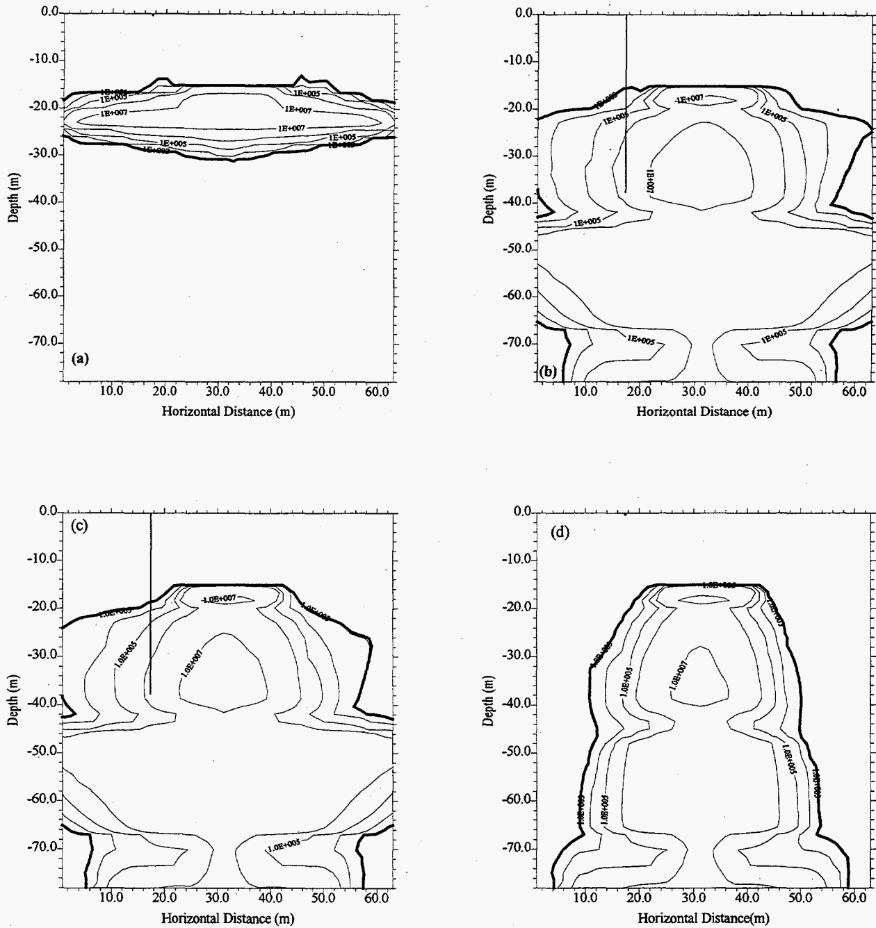
Figure 20. Simulated ^{99}\text{Tc} Concentration ( \text{pCi L}^{-1} ) in 1983 Showing the Impact of Recharge Rate, J_w , on Plume Migration (a) Case 4, J_w = 0.5 \text{ mm yr}^{-1} , (b) Case 6, J_w = 10 \text{ mm yr}^{-1} , (c) Case 3, Variable Recharge, and (d) Case 7, J_w = 100 \text{ mm yr}^{-1} . The Vertical Line at 17.6 m on the X-Axis Represents the Borehole. The Bold Isopleth is 900 \text{ pCi L}^{-1} .
