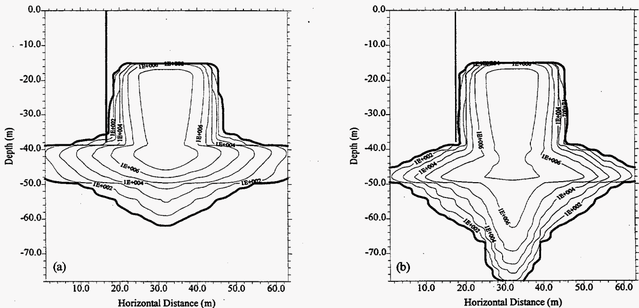
Figure 11. Simulated ^{137}\text{Cs} Concentration ( \text{pCi g}^{-1} ) in 1973 Showing the Impact of Specific Gravity on Plume Migration With a Simplified Stratigraphy Under a Variable Recharge and K_d = 0 \text{ mL g}^{-1} (a) Case 1, Pure Water, and (b) Case 3, Specific Gravity = 1.4. The Vertical Line at 17.6 m on the X-axis Represents the Borehole. The Bold Isopleth is 10 \text{ pCi g}^{-1} .
