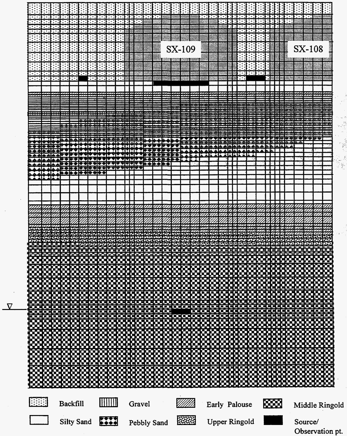
Figure 5. Schematic of the Two-dimensional Simulation Domain Showing the Major Stratigraphic Units Considered and the Location of the Source and Observation Points.
