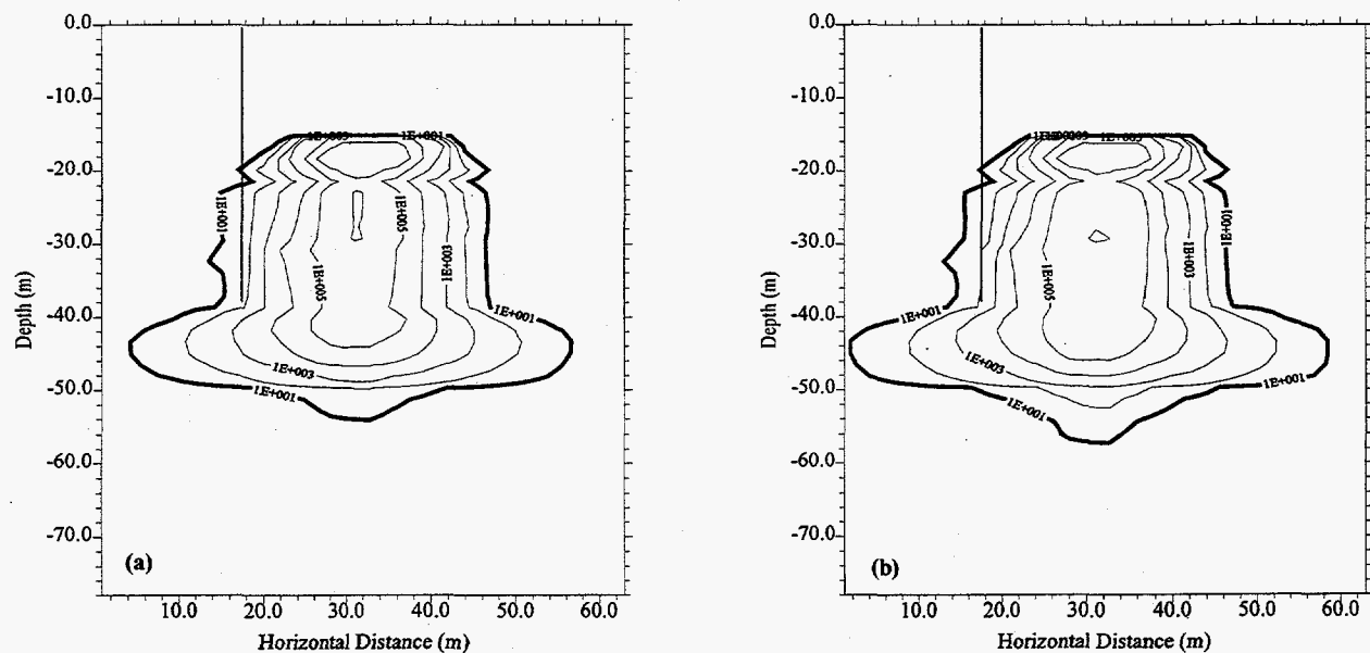
Figure 15. Simulated ^{137}\text{Cs} Concentration ( \text{pCi g}^{-1} ) in 1996 Showing the impact of a Change in Release history. A Total of 15 \text{ m}^3 was Leaked over 15 yr (a) Case 12, Specific Gravity = 1.0, and (b) Case 13, Specific Gravity = 1.4. A Variable Recharge Rate and a K_d = 0 \text{ mL g}^{-1} were Assumed. The Borehole is Shown at 17.6 m on the X-axis. The Bold isopleth is 10 \text{ pCi g}^{-1} .
