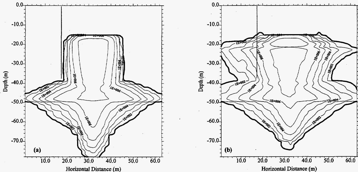
Figure 12. Simulated 137 Cs Concentration (pCi g -1 ) in 1973 Showing the Impact of Stratigraphic Detail on Plume Migration Under a Variable Flux and K_d = 0 \text{ mL g}^{-1} , (a) Case 2, Simple Stratigraphy, and (b) Case 3, Complex Stratigraphy. The Borehole is Shown at 17.6 m on the X-axis. The Bold Isopleth is 10 pCi g -1 .
