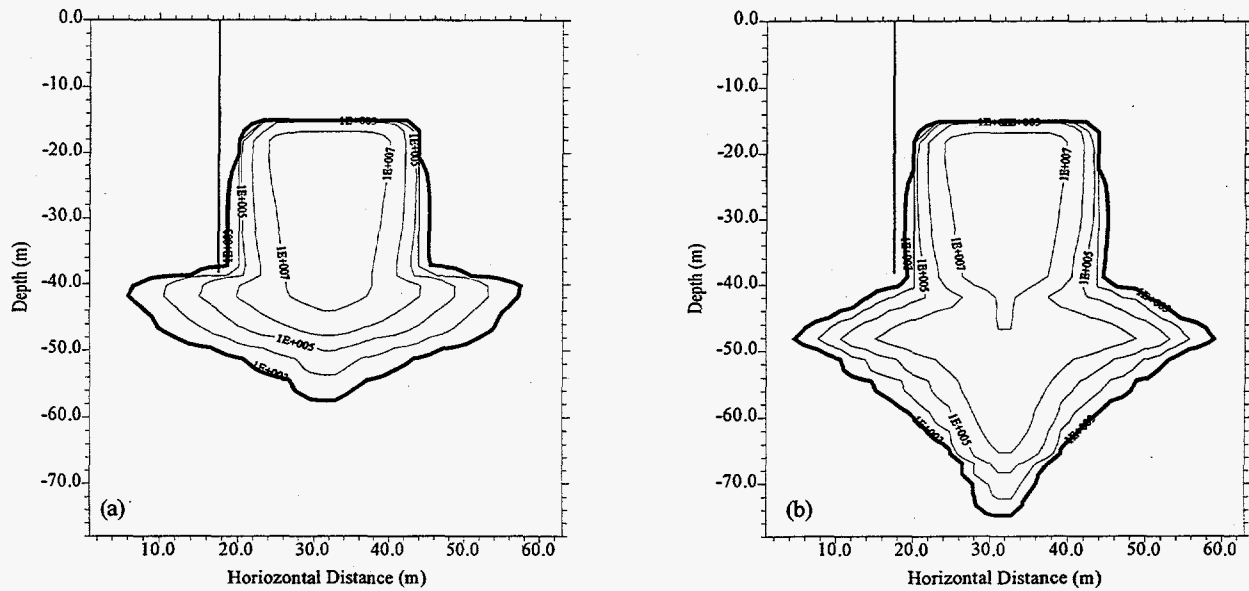
Figure 18. Simulated ^{99}\text{Tc} Concentration ( \text{pCi L}^{-1} ) in 1973 Showing the Impact of Specific Gravity on Plume Migration with a Simplified Stratigraphy Under a Variable Recharge (a) Case 1, Pure Water, and (b) Case 3, Specific Gravity = 1.4. The vertical line at 17.6 m on the x-axis represents the borehole. The bold isopleth is 900 \text{ pCi L}^{-1} .
