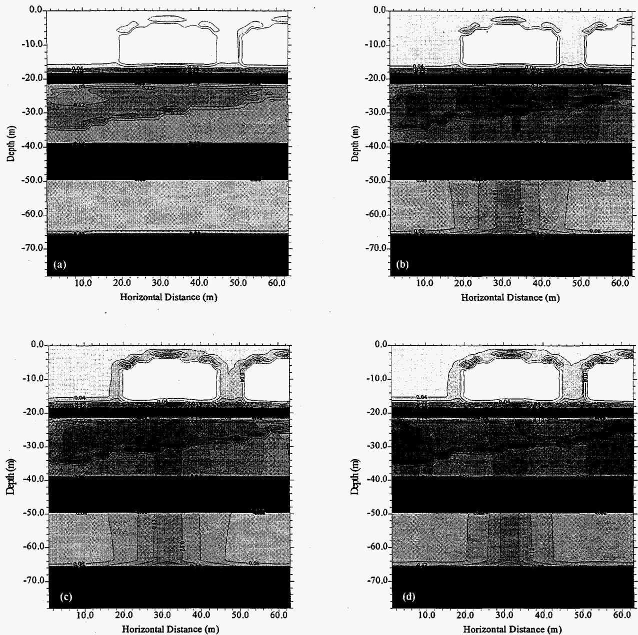
Figure 9. Simulated Volumetric Water Content ( \text{m}^3 \text{m}^{-3} ) in 1973 Showing the Impact of Recharge Rate, J_w , on Moisture Distribution in a Profile with Complex Stratigraphy (a) Case 4, 0.5 \text{ mm yr}^{-1} , (b) Case 6, 10 \text{ mm yr}^{-1} , (c) Case 3, J_w Variable, and (d) 100 \text{ mm yr}^{-1} .
