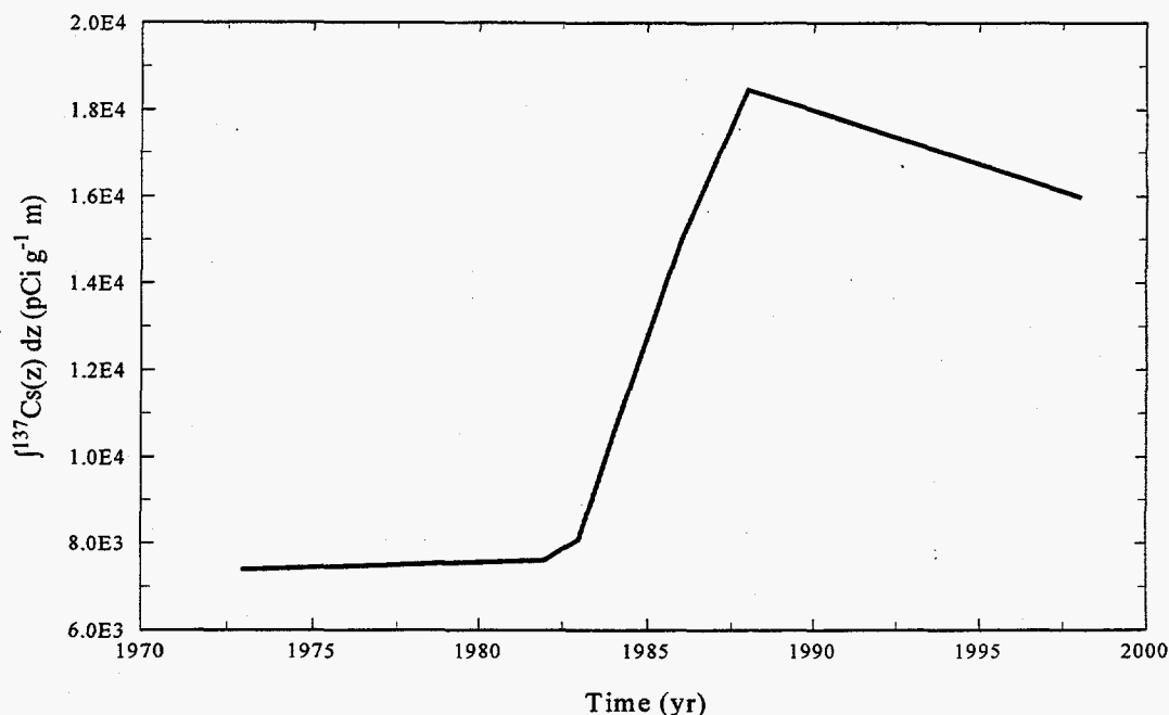
Figure 17. Simulated Accumulation of 137 Cs at the Borehole in Response to the Leak History Depicted in Figure 6 and the Conditions Assumed in Case 12 (Figure 16d). Both the Recharge Rate and K_d were Assumed to be Variable.
