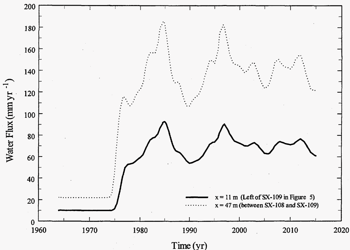
Figure 10. Comparison of Water Flux Between Two Tanks and Away From a Tank at a Depth of 16 m, Showing the Umbrella Effect (Case 3). Recharge Between the Tanks Ranged From 1.8 to 4.6 Times Higher Than the Imposed Recharge Rate.
