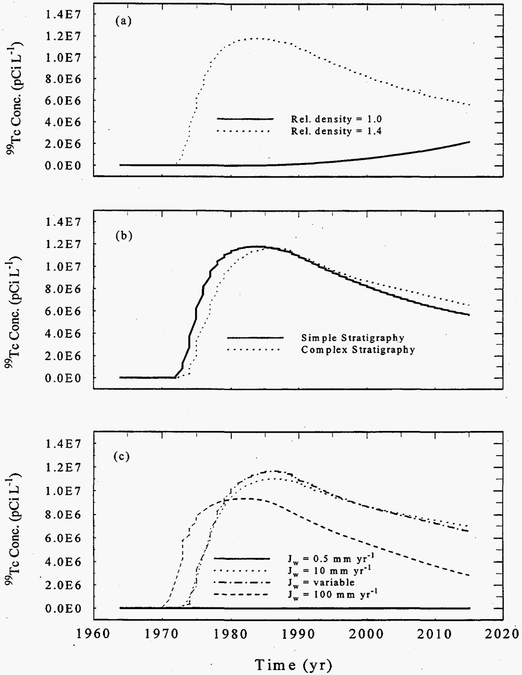
Figure 21. Time Series Plot of Simulated ^{99}\text{Tc} Concentration (pCi L ^{-1} ) at the Water Table Below SX-109 Showing the Impact of (a) Specific Gravity, (b) Stratigraphy, and (c) Recharge rate, J_w . In all Cases, a Leak of 500 m ^3 (132,000 gal) was Assumed and the Simulations Were Run For 50 yr, Starting in 1964.
