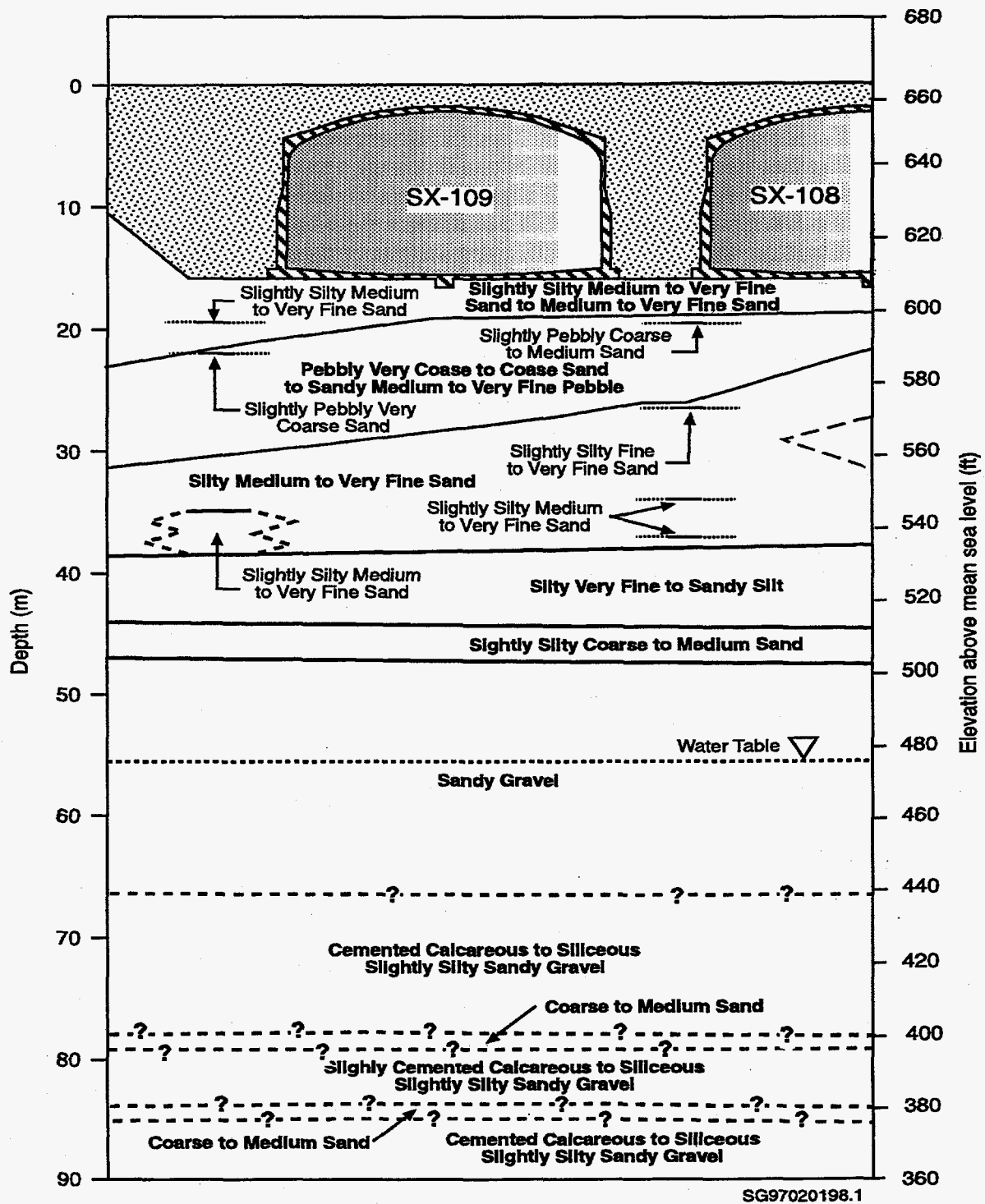
Figure 3. Geologic Characterization of SX Farm. The Cross Section Was Taken Through Tanks SX-108 and SX-109 (after Price and Fecht 1976).
