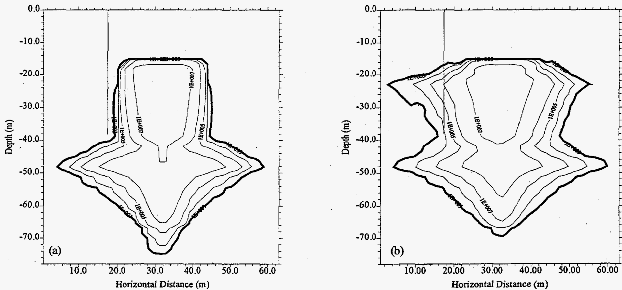
Figure 19. Simulated ^{99}\text{Tc} Concentration ( \text{pCi L}^{-1} ) in 1973 Showing the Impact of Stratigraphic Detail on Plume Migration Under a Variable Recharge (a) Case 2, Simple Stratigraphy, and (b) Case 3, Complex. The vertical line at 17.6 m on the x-axis represents the borehole. The bold isopleth is 900 \text{ pCi L}^{-1} .
