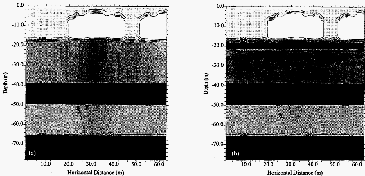
Figure 8. Simulated Volumetric Water Content ( \text{m}^3 \text{m}^{-3} ) in 1973 Showing the Impact of Stratigraphic Detail on Moisture Distribution in a Profile with Simplified Stratigraphy (a) Case 2, Simple Stratigraphy, and (b) Case 3, Complex Stratigraphy, Including Lenses <0.6 m Thick.
