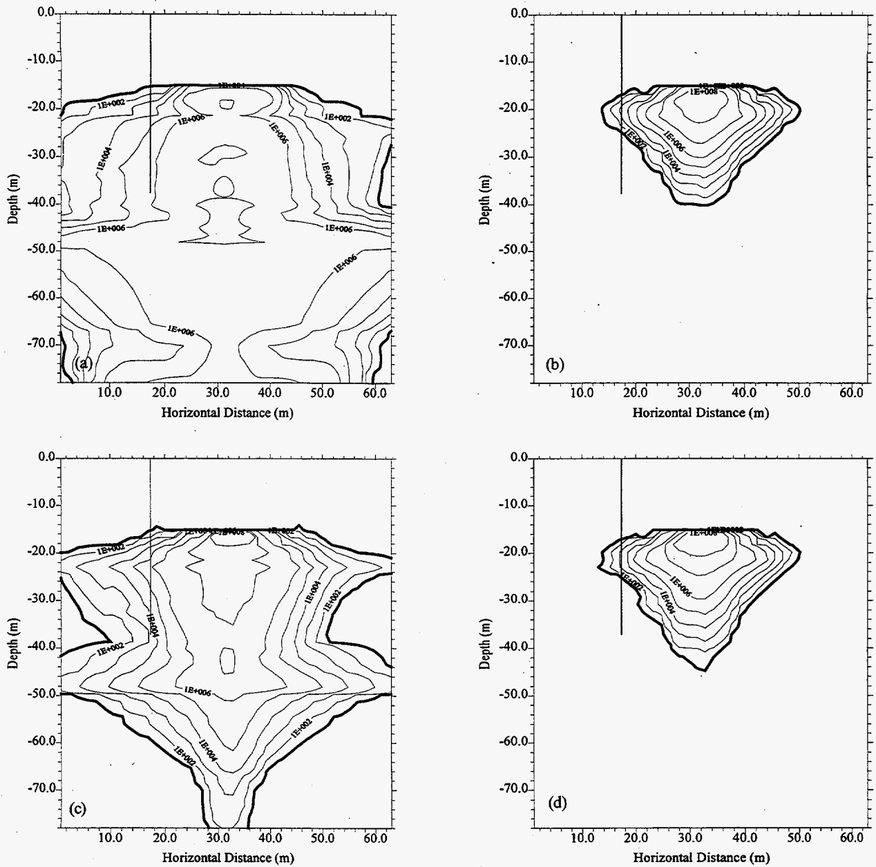
Figure 14. Simulated ^{137}\text{Cs} Concentration ( \text{pCi g}^{-1} ) in 1983 Showing the Impact of K_d on Plume Migration Under a Variable Recharge Rate (a) Case 3, K_d = 0 \text{ mL g}^{-1} , (a) Case 8, K_d = 3.0 \text{ mL g}^{-1} , \text{mm yr}^{-1} , (b) Case 11, K_d = 0.5 and 3.0 \text{ mL g}^{-1} , and (d) Case 12, K_d = 0/0.5/3.0/37/3.0/37.0 \text{ mL g}^{-1} (see Table 5). The Borehole is shown at 17.6 m on the X-axis. The Bold isopleth is 10 \text{ pCi g}^{-1} .
