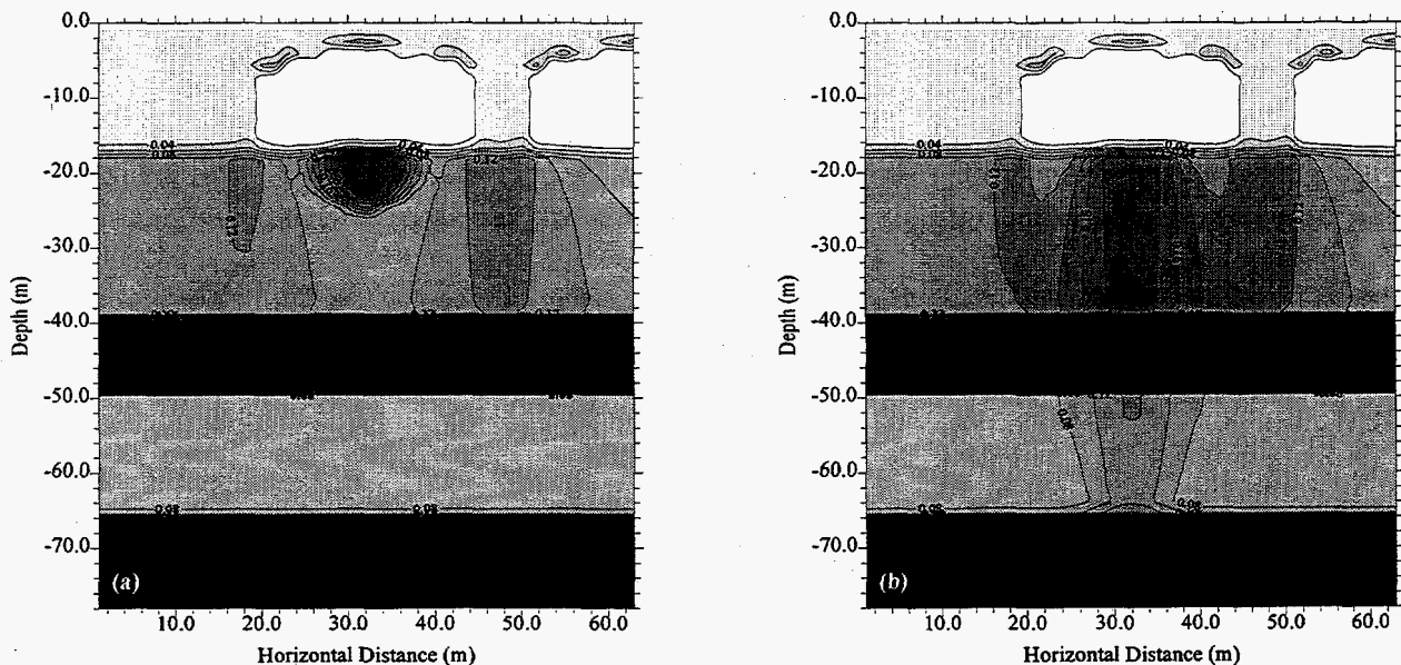
Figure 7. Simulated Volumetric Water Content ( \text{m}^3 \text{m}^{-3} ) in 1973 Showing the Impact of Specific Gravity of the Leaked Fluid on Moisture Distribution in a Profile with Simplified Stratigraphy (a) Case 1, Specific Gravity = 1.0; (b) Case 2, Specific Gravity = 1.4.
