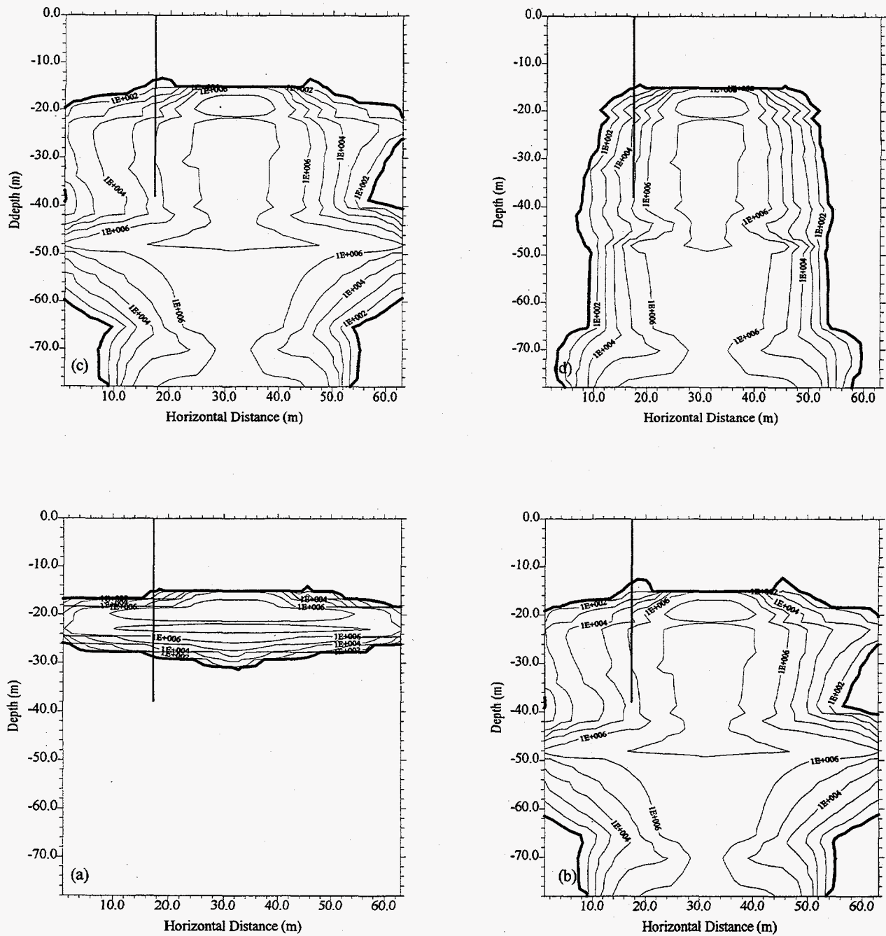
Figure 13. Simulated ^{137}\text{Cs} Concentration ( \text{pCi g}^{-1} ) in 1983 Showing the Impact of Recharge Rate, J_w , on Plume Migration With a K_d = 0 \text{ mL g}^{-1} , (a) Case 4, J_w = 0.5 \text{ mm yr}^{-1} , (b) Case 6, J_w = 10 \text{ mm yr}^{-1} , (c) Case 3, Variable Recharge, and (d) Case 7, J_w = 100 \text{ mm yr}^{-1} . The Borehole is Shown at 17.6 m on the X-axis. The Bold Isopleth is 10 \text{ pCi g}^{-1} .
