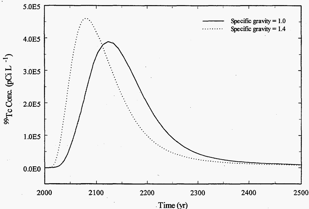
Figure 22. Time Series Plot of Simulated ^{99}\text{Tc} Concentration ( \text{pCi L}^{-1} ) at the Water Table Below Tank SX-109 Showing the Impact of Specific Gravity on Plume Migration After a Leak of 15 \text{ m}^3 ( 4000 ) Over a 15-yr Period.
