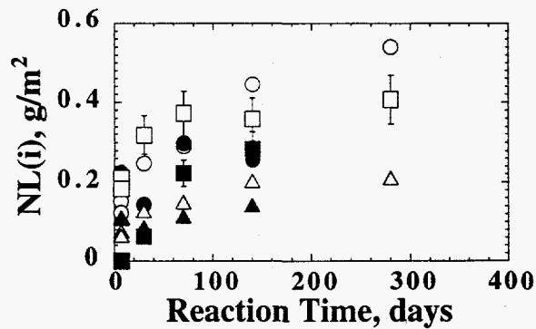
Fig. 2. Normalized Mass Loss vs. Reaction Time for PCTs in EJ-13 at (a) 2000 \text{ m}^{-1} and (b) 20,000 \text{ m}^{-1} : NL(B) (● and ○), NL(Na) (■ and □), and NL(Si) (▲ and Δ); filled symbols for tests with 51R glass; open symbols for tests with 51S glass.
