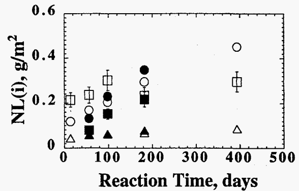
Fig. 2. Normalized Mass Loss vs. Reaction Time for PCTs in EJ-13 at (a) 2000 \text{ m}^{-1} and (b) 20,000 \text{ m}^{-1} : NL(B) (● and ○), NL(Na) (■ and □), and NL(Si) (▲ and Δ); filled symbols for tests with 51R glass; open symbols for tests with 51S glass.
