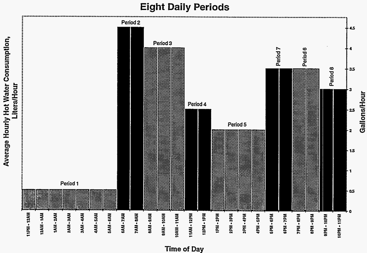
Figure 1. Average Hot Water Consumption for Summer Weekdays
