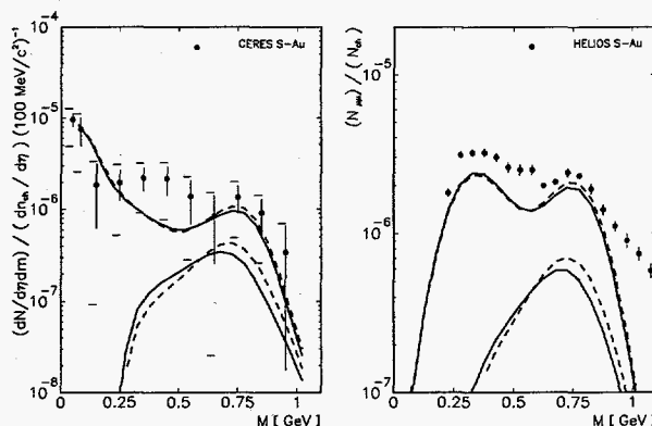
Figure 2: Dilepton invariant mass spectrum with (full line) and without (dashed line) in-medium corrected pion annihilation in comparison with CERES (left) and HELIOS [4] (right) data.
