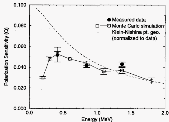
Figure 1: The experimental results for Q are compared to theoretical energy dependences.
