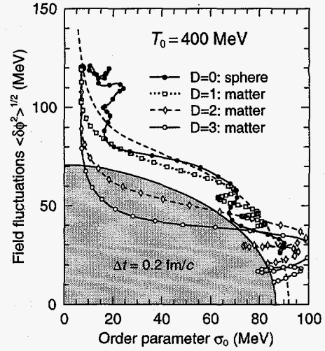
Figure 1: The combined dynamical evolution of the order parameter and the field fluctuations. The dashed curve connects the equilibria and the shaded region is the unstable region within which \mu_\pi^2 < 0 . The systems start in equilibrium at T_0 = 400 MeV. The irregular solid trajectory ( D=0 ) has been obtained by solving the standard equations of motion for a spherical source with R=5 fm. The other three trajectories have been obtained by adding a cooling term emulating expansion in D=1,2,3 dimensions.
