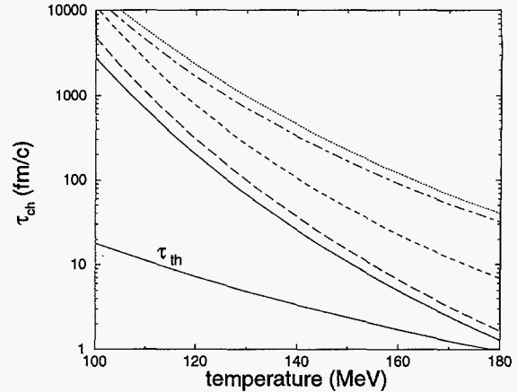
Figure 1: Chemical relaxation time of pions in hot hadronic matter. The reactions \rho\rho \leftrightarrow \pi\pi (long dashed curve), \pi\omega \leftrightarrow \pi\pi (dashed-dot curve), \pi a_1 \leftrightarrow \pi\pi (dashed curve) and \pi\pi\pi\pi \leftrightarrow \pi\pi (dotted curve) are considered. The solid curve represents the total relaxation time. These results are compared with the thermal relaxation time, \tau_{th} .
