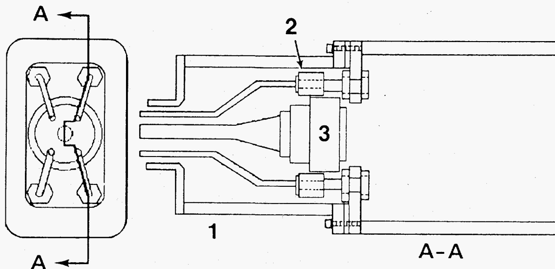
Fig. 5.1. Separation of capsule from umbilical cable. Identified components are: (1) gasketed cable connector cover, (2) gas line Swagelock fitting, and (3) instrumentation Amphenol connector.
