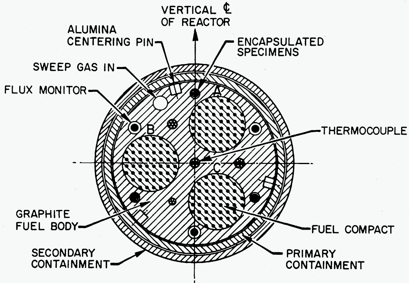
Fig. 2.1. Horizontal section through capsule HRB-21.
