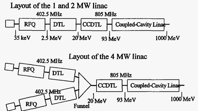
Figure 1. Layout of the accelerator structures for the 1, 2, and 4 MW NSNS linacs.
