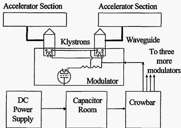
Figure 2. Schematic of the RF system with the dual-klystron modulator.
