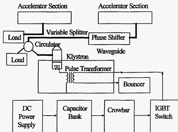
Figure 3. The solid-state modulator with a 5 MW klystron and waveguide splitter system.
