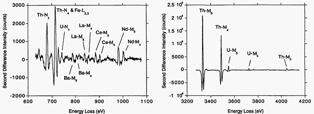
Fig. 6. The EELS spectra from the brockite indicate nearly identical distributions of REEs and actinides as that observed in brockite particles from tests terminated at times of one year or less [12].
