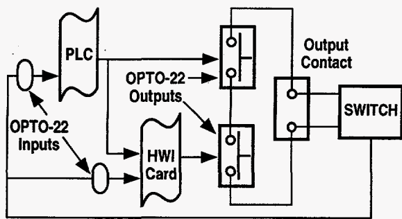
Fig. 3. Typical series redundant circuitry.
