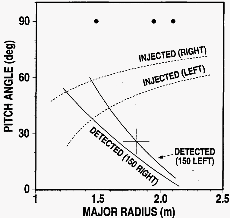
Fig. 3. Pitch angle \chi , where \cos\chi = v_{\phi\ominus}/v , versus major radius R . The dashed lines show the pitch angles of ions born near R . The solid lines show the pitch angles accessible to the horizontal analyzer when using the 150^\circ beams for active charge-exchange measurements; the error bar shows the total spread in major radius and pitch angle associated with the beam footprint. (The 1/e intensity points are approximately half as large.) The sightlines of the vertical analyzers (circles) are also indicated.
