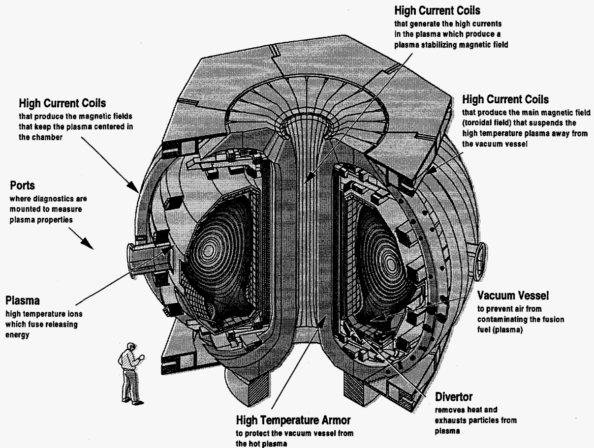
Fig. 3. A cross-sectional view of DIII-D showing the major features of a tokamak device, including the various coils for producing the confining magnetic fields and shaping the plasma.
