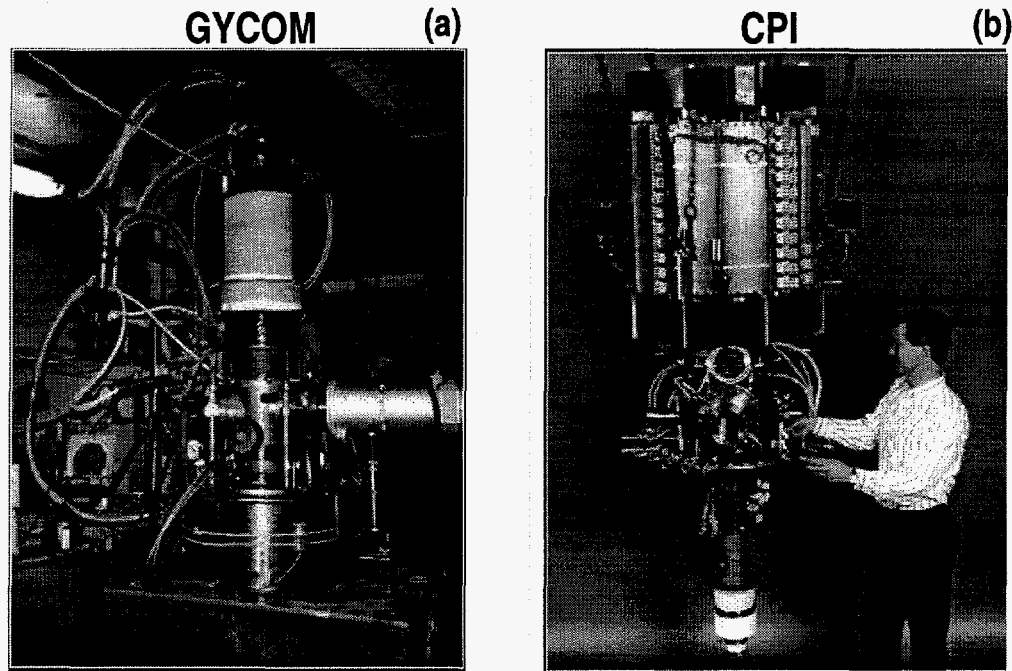
Fig. 5. MW-level, 110 GHz gyrotrons with internal mode converters: (a) Gycom; (b) CPI. The microwave outputs are from windows on the side and the unspent beam is collected at the top.
