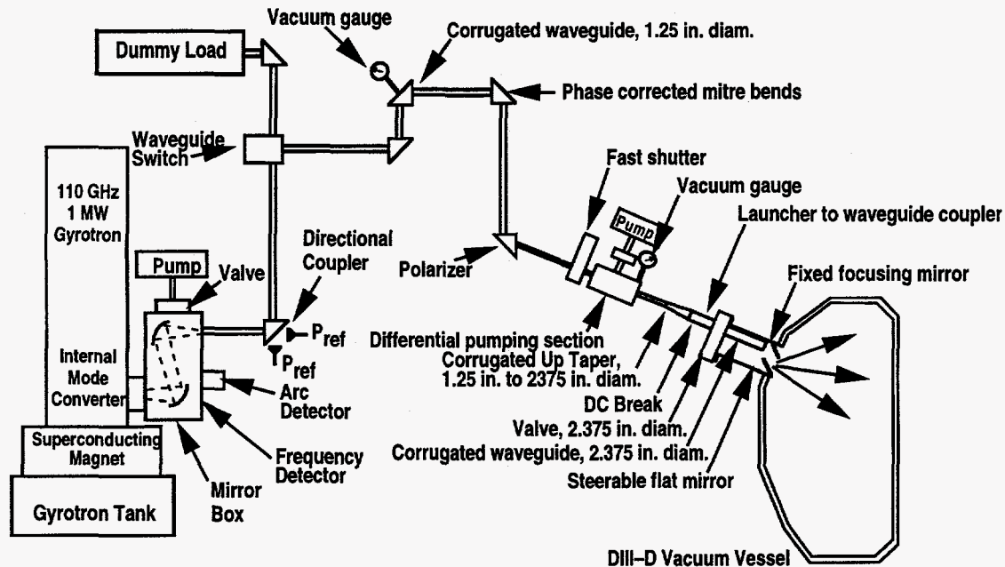
Fig. 6. DIII-D 1 MW, 110 GHz gyrotron system (not to scale).
