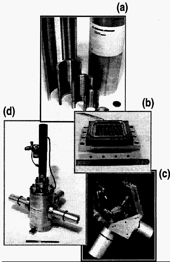
Fig. 7. General Atomics high power millimeter wave transmission line components. Clockwise from top: (a) corrugated waveguides; (b) distributed window; (c) directional coupler; and (d) waveguide switch.
