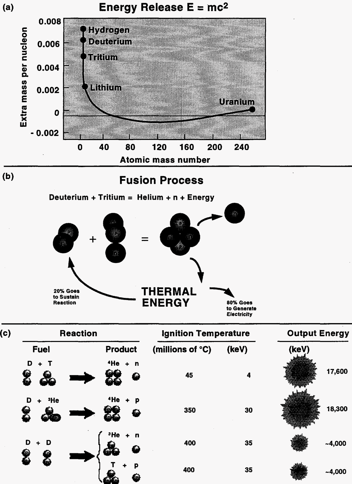
Fig. 1. (a) Excess energy per nucleon shows "fusion" of low mass nuclei liberates energy as does "fission" of high mass nuclei; (b) most energetically favorable fusion reaction is deuterium with tritium, which releases helium and an energetic neutron; and (c) other fusion reactions.
