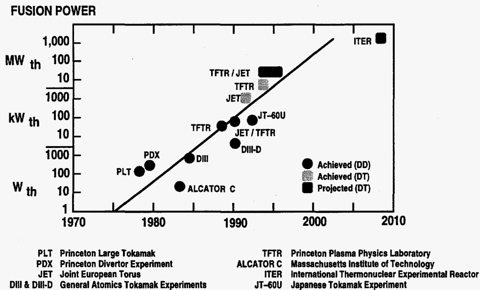
Fig. 2. Fusion power produced in worldwide experimental devices as function of time showing six orders of magnitude increase over the past twenty years.
