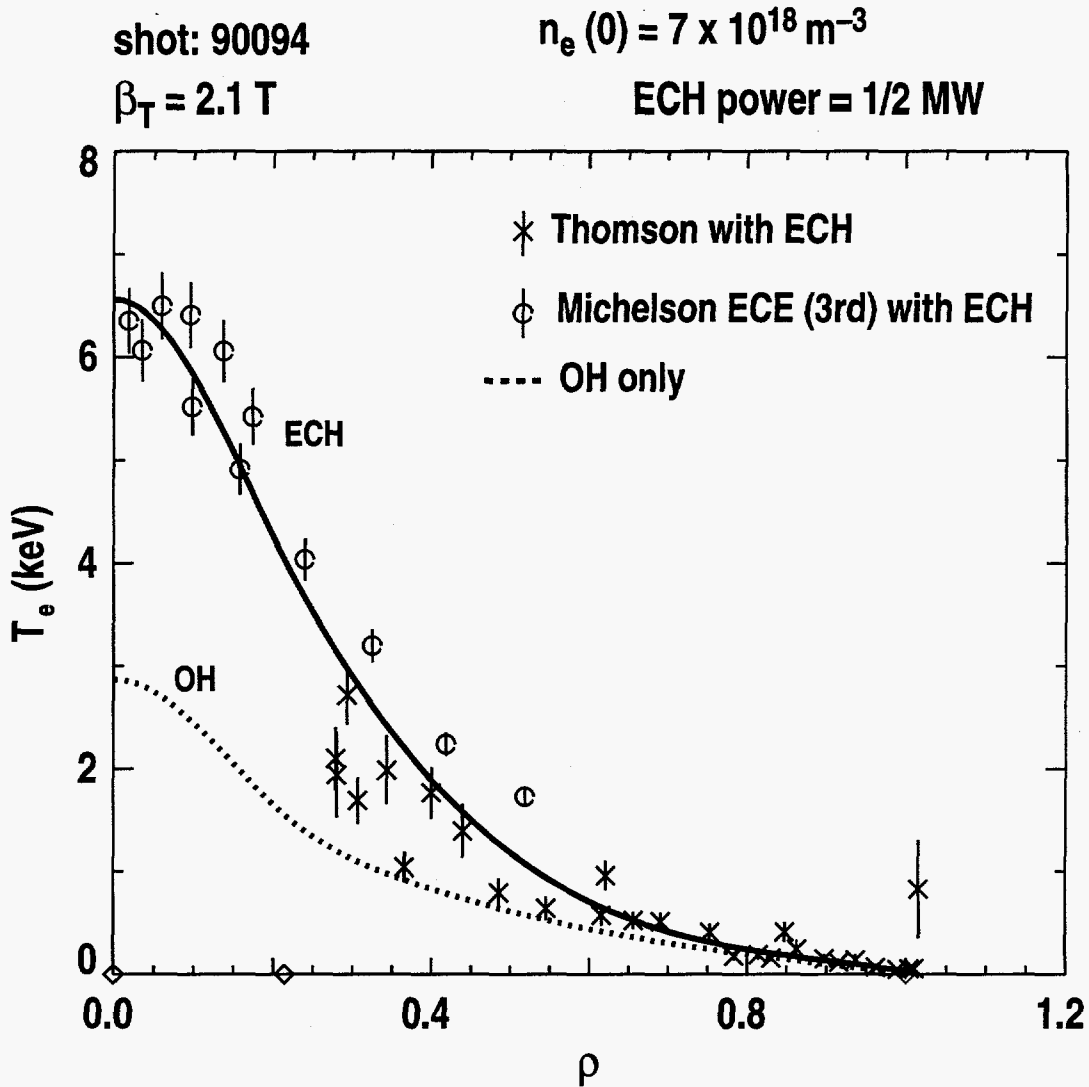
Fig. 4. Electron temperature as a function of normalized minor radius with ohmic heating alone (OH) and with 0.5 MW of millimeter wave power added.
