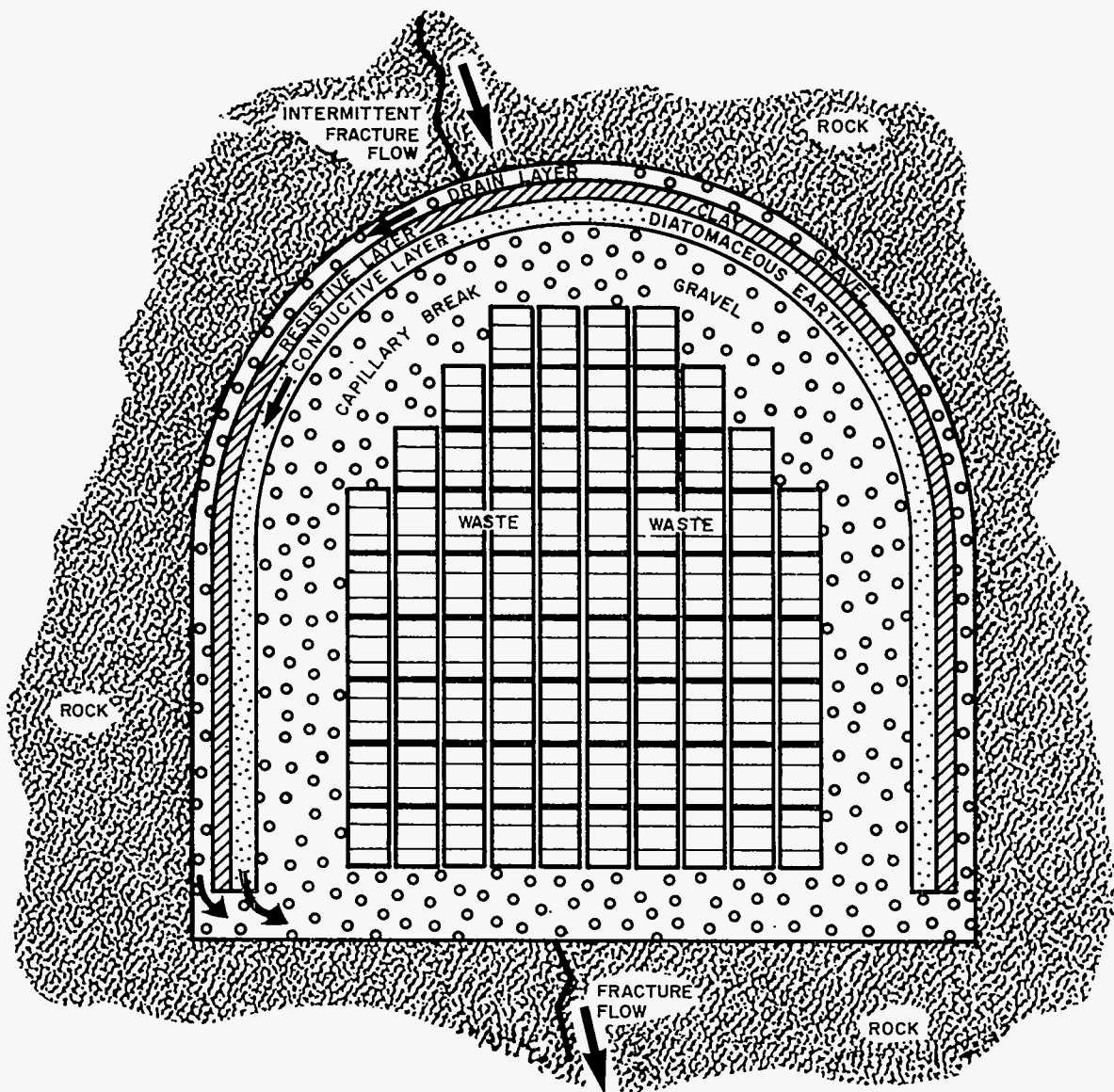
Fig. 28. Artist's concept of resistive and conductive layer barriers to protect high-level waste from water flowing through rock fracture. Resistive (clay) layer diverts almost all fracture flow water. Conductive layer (very fine sand or diatomaceous earth) scavenges small quantities of water that pass through clay layer. Conductive layer transports scavenged water, under tension, around waste.
