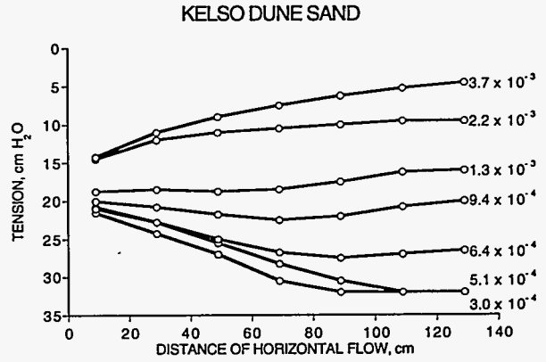
SOIL WATER TENSION AT VARIOUS FLOW RATES, (cm/sec) TENSION vs HORIZONTAL DISTANCE FROM DISCHARGE POINT
