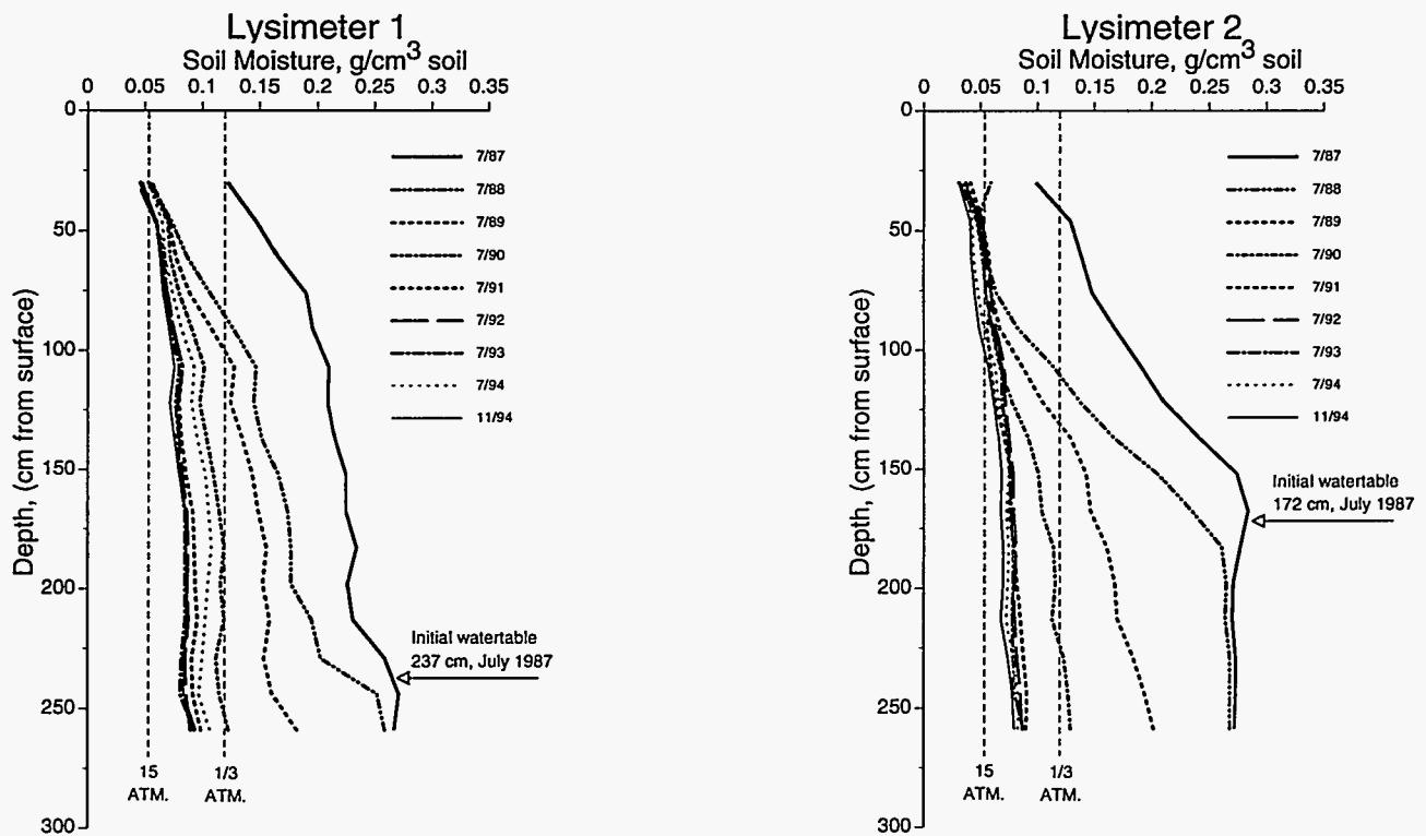
Fig. 11. Bioengineered covers. Volumetric soil moisture content plotted as a function of soil depth at nine different dates. By July, 1989, water table was eliminated from soil profiles. As of November, 1994, entire soil profiles, although relatively dry, still showed slightly increasing moisture content with depth.
