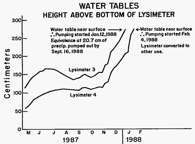
Fig. 7. Water table vs. time in reference lysimeters. Crowned surface is planted with fescue grass. Water table increased with time until pumping was necessary to keep trench from running over. Surface run-off was 8% of precipitation.
