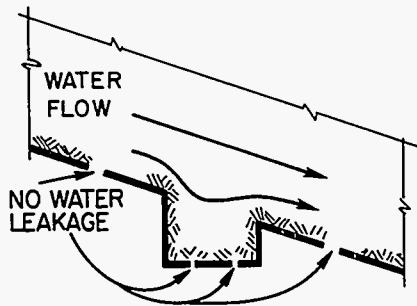
Fig. 19. Imperfectly constructed conductive layer with "pocket" extending down into rock (or capillary break) layer. No leakage if conditions required to maintain tension are met.
