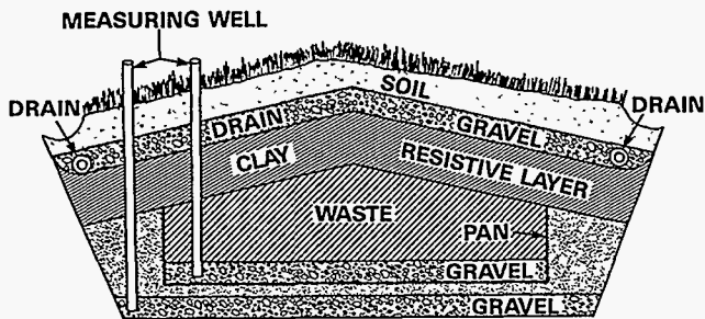
Fig. 15. Resistive-layer barrier with grass cover. Similar to UMTRA cover but has soil and vegetation in place of rip-rap. See Fig. 14.
