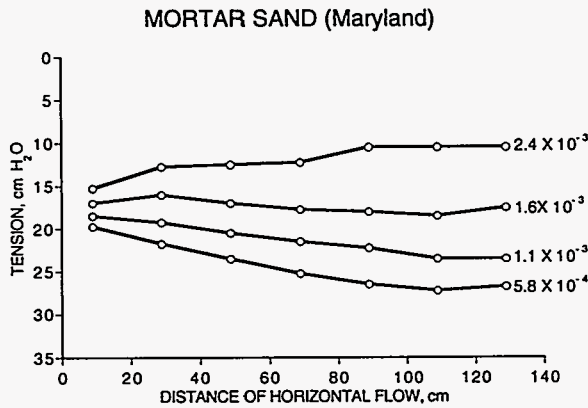
SOIL WATER TENSION AT VARIOUS FLOW RATES, (cm/sec) TENSION vs HORIZONTAL DISTANCE FROM DISCHARGE POINT
