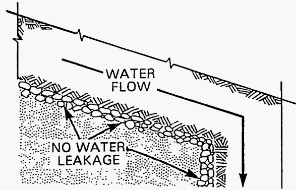
Fig. 18. Substitution of rock layer for holes shown in Fig. 17. Voids between rocks act exactly like holes shown in Fig. 17. They form a capillary discontinuity, preventing leakage downward under the influence of gravity.
