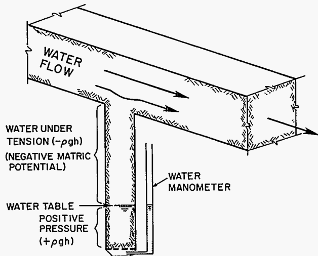
Fig. 20. Schematic of laboratory apparatus for measurement of water tension using different materials and varying flow rates.
