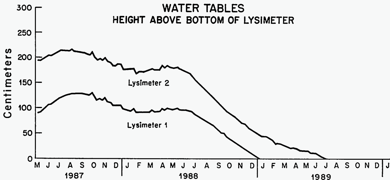
Fig. 8. Water table vs. time in bioengineered lysimeters. Decline of water-table levels with time shows bioengineered covers effectively prevented water percolation. Elimination of water table shows that this procedure could be used for remedial action ("drying out") of existing water-logged burial sites. Compare with Fig. 7.
