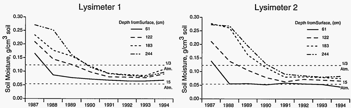
Fig. 12. Bioengineered covers. Volumetric soil moisture content at four depths in the soil profile at the end of each seasonal year. In lysimeter 1 and at the 244 cm (8 ft) level the moisture content continued to drop through the end of seasonal 1992-1993. However, a rise in moisture content is evident in lysimeter 1 at the end of seasonal 1993-1994. No rise in moisture content is evident in lysimeter 2. The two percent rise of moisture in lysimeter 1, in itself, is not important if the rise does not increase with further passage of time.
