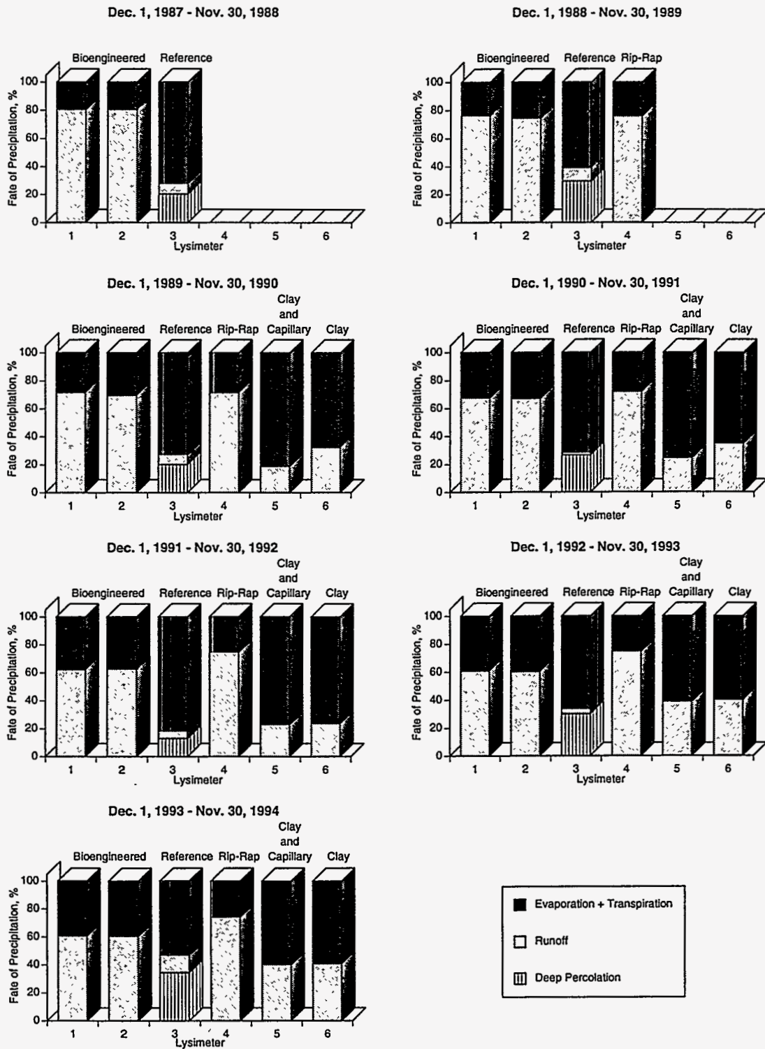
Fig. 9. Fate of precipitation in bioengineered, reference (soil with grass), UMTRA (clay with riprap), clay (clay with grass), and clay + capillary (clay and capillary layers with grass), lysimeters. Deep percolation is present in reference lysimeter. No deep percolation has occurred to date in any other cover system with the exception of 0.13 cm (0.05 in) in lysimeter 5 in 1993-1994.
