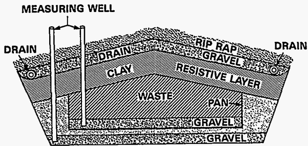
Fig. 14. Resistive-layer barrier with rock cover; no vegetation. Possible UMTRA cover. Possible advantages over vegetated, resistive-layer barrier: (1) Clay layer remains wet and more efficient barrier to escape of radon. (2) Initially, superior erosion protection. (3) No root penetration of waste. Major disadvantage: no plant transpiration, therefore requiring clay barrier of extremely low hydraulic conductivity. For clarity, most instrumentation and some details not shown. Plot (lysimeter) is 21.34 m (70 ft) long by 13.72 m (45 ft) wide; bottom is 3.05 m (10 ft) below grade. Clay layer is 46-61 cm (1½-2 ft) thick. Slope is 1:5.
