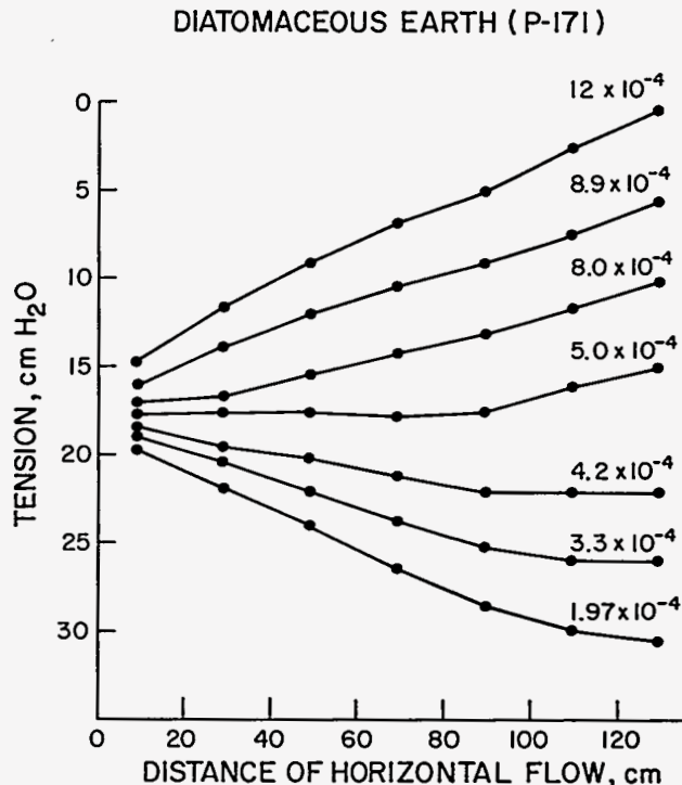
Fig. 22. Soil water tension at various flow rates, measured in miniature soil beam shown in Fig. 21. Tension vs. horizontal distance from discharge point. Results suggest that, at 4.2 \times 10^{-4} cm/sec or less, water would remain under tension at any beam length. Slope of beam is 1:5.
