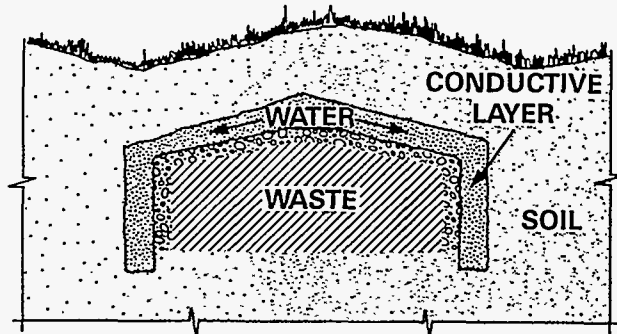
Fig. 2. Conductive layer barrier.
