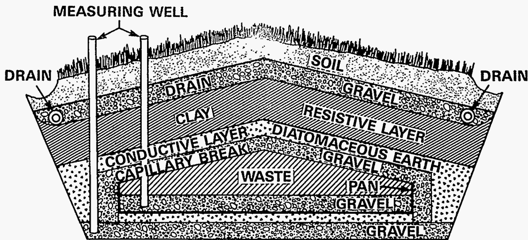
Fig. 25. Combination resistive-layer barrier over a conductive layer barrier. Clay-barrier (resistive layer barrier) needs only to protect to approximately 10^{-6} cm/sec. Conductive-layer barrier of diatomaceous earth readily transports percolating water around waste.
