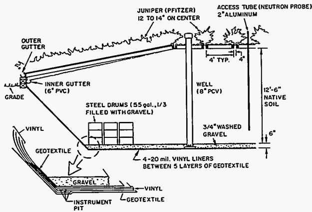
Fig. 6. Side view of bioengineered lysimeter. Surface run-off is collected from both engineered surface and soil surface. Soil moisture content measured with neutron probe. Water table is measured in well.
