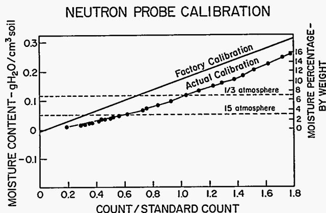
Fig. 10. Calibration of neutron probe using soil of bioengineered lysimeters. Calibration was carried out in weighing lysimeter over a 7-yr period. Factory calibration was supplied by manufacturer of neutron probe and made against sand rather than soil.
