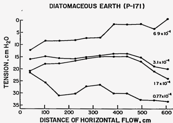
Fig. 24. Soil water tension at various flow rates, measured in large soil beam shown in Fig. 23. That beam is 6.4 m (21 ft) long and has slope of 1:5. At -15 to -20 cm, matric potential water flow rate is approximately 3 \times 10^{-4} cm/sec. At this rate, unsaturated flow can be maintained over an infinite distance, confirming results of soil beam measurements (Fig. 22).
