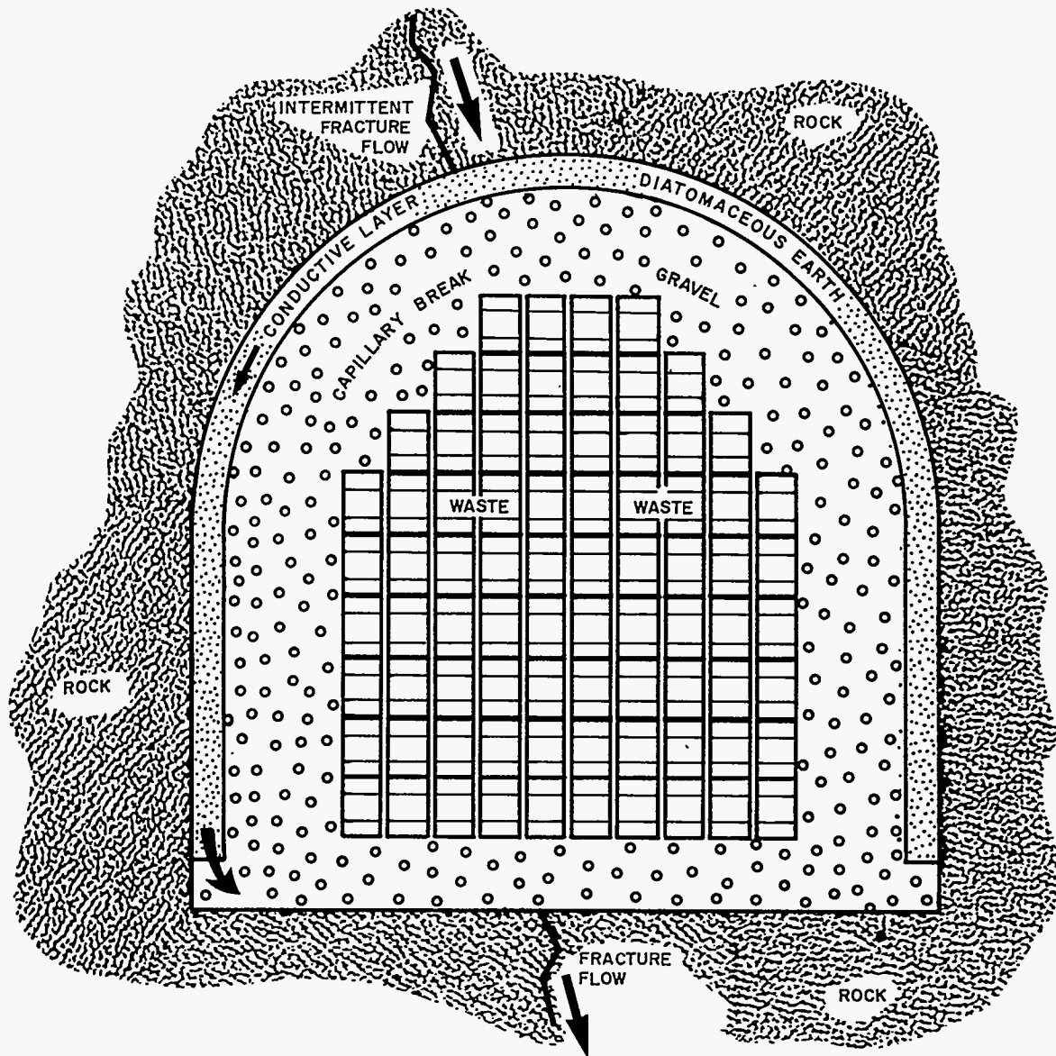
Fig. 29. Simplified case of Fig. 28. If fracture flow is slow conductive layer transports all water around waste; clay layer is then not needed.
