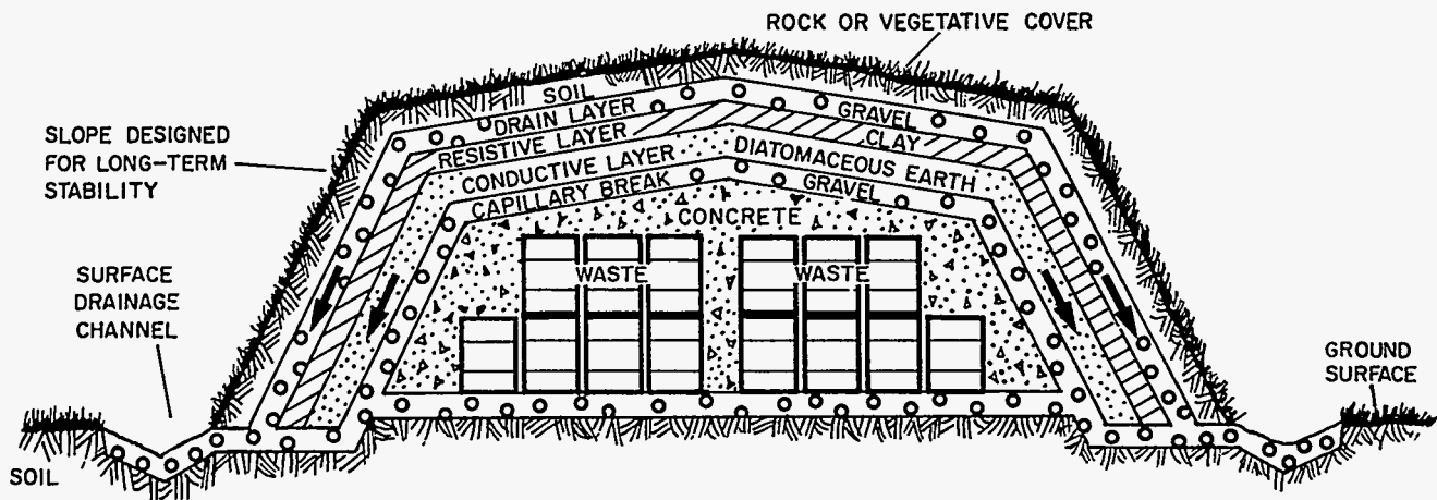
Fig. 27. Resistive-layer barrier overlaying a conductive-layer barrier as might be used with an earth-mounded concrete bunker. Resistive (clay) layer is primary barrier to water passage downward. Conductive layer (diatomaceous earth) scavenges and conducts any water percolating through clay layer around concrete structure to drains. Diatomaceous/gravel interface is capillary break. Concrete is exposed only to a stagnant, alkaline film of water, greatly retarding degradation of concrete over time. Only geological materials already over 1 million yr old are used in construction, other than concrete, so life of cover will far exceed that of concrete, even though this cover system can be expected to significantly increase structural life of concrete.
