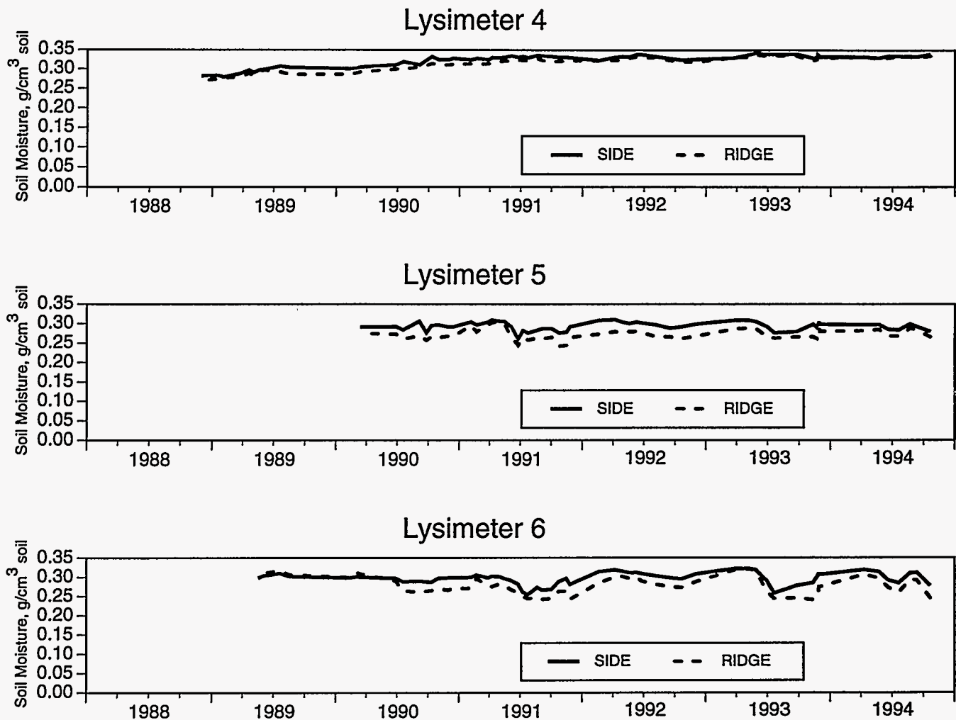
Fig. 16. Moisture content of clay layers with time. Lysimeter 4 cover system is a clay layer covered with gravel and rip-rap. No vegetation is present, and clay shows a very slight increase of water content with time. Lysimeter 5 has a capillary (conductive-scavenging) layer underneath clay layer; plot is planted with grass. During five-year life of plot, largest variations in moisture content were during summer. Lysimeter 6 has clay layer with a grass cover. As in lysimeter 5, largest moisture excursions were in summer.
