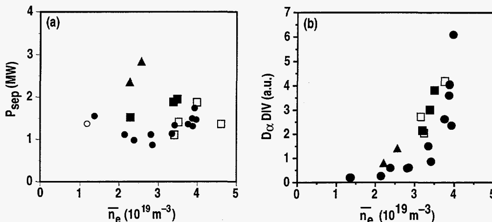
Fig. 1. (a) P_{\text{lh}} ( P_{\text{sep}} ) required to produce H-mode vs. line averaged density n_e . ( I_p = 1.35 MA, B_T = 2.1 T) Data from 1994 with (open circle) and without (solid circles) error field correction coil show that P_{\text{lh}} is minimum for n_e in range of 2\text{--}3 \times 10^{19} \text{ m}^{-3} and increases for lower and higher values of n_e . Data from neutrals experiment shown for positive density ramp (open squares), no gas puff (solid squares) and negative density ramp (diamonds). (b) Divertor D_{\alpha} emission, assumed to be an indicator for neutral density, as a function of n_e . 1994 n_e scan (circles) shows that D_{\alpha} increases nonlinearly with n_e . D_{\alpha} values obtained from experiment which attempted to break correlation of neutral density and n_e are comparable to values from 1994 scan, evidence that neutral density is strongly correlated with n_e . Symbols have same meaning as in (a).
