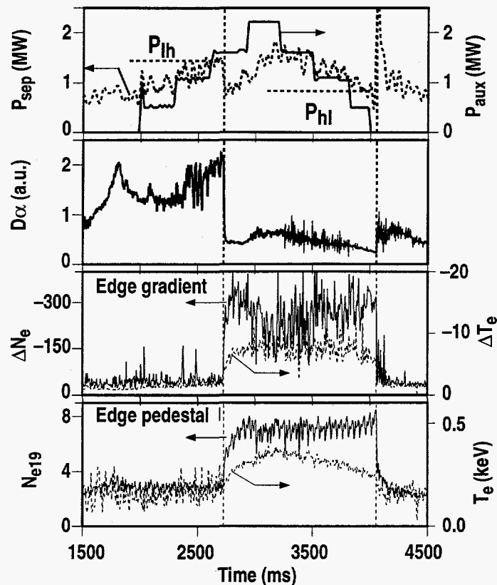
Fig. 2. (a) Solid line shows injected neutral beam power P_{aux} which was ramped up and then ramped down in stairstep fashion. Dashed line shows P_{sep} . H-L transition occurred after beam power was turned off. Nevertheless, H-mode was sustained with P_{sep} of about 60% of P_{lh} . ( I_p = 1.35 MA, B_T = 2.1 T) (b) D_\alpha as a function of time. Dashed vertical lines mark time of L-H transition (about 2700 ms) and H-L transition (4100 ms). (c) Gradients of T_e (keV/m) and n_e ( 10^{19} \text{ m}^{-4} ) in the transport barrier show similar time behavior. They rise rapidly after L-H transition and drop abruptly at H-L transition. (d) Pedestal values of T_e and n_e , determined from hyperbolic tangent fit, show that T_e starts to decrease as P_{sep} is decreased. In contrast, n_e remains unchanged until back transition.
