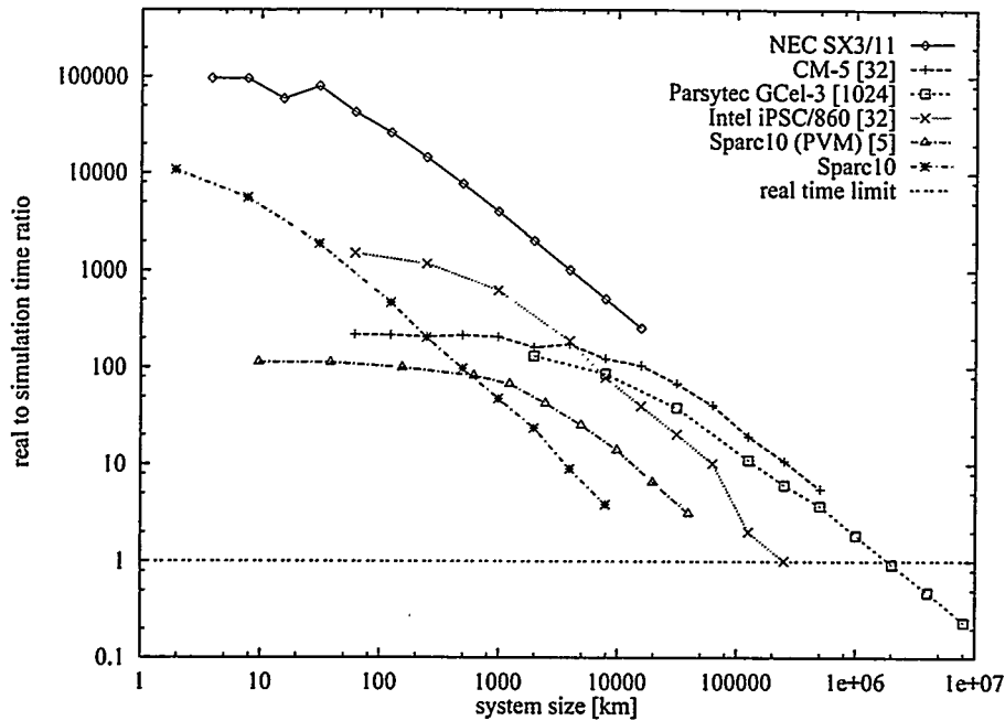
Fig. 3. Comparison between real time and computer time for different system sizes, i.e. the factor \tau the computer model runs faster than reality. The system sizes where the curves cross \tau = 1 are the so-called real time limits.
