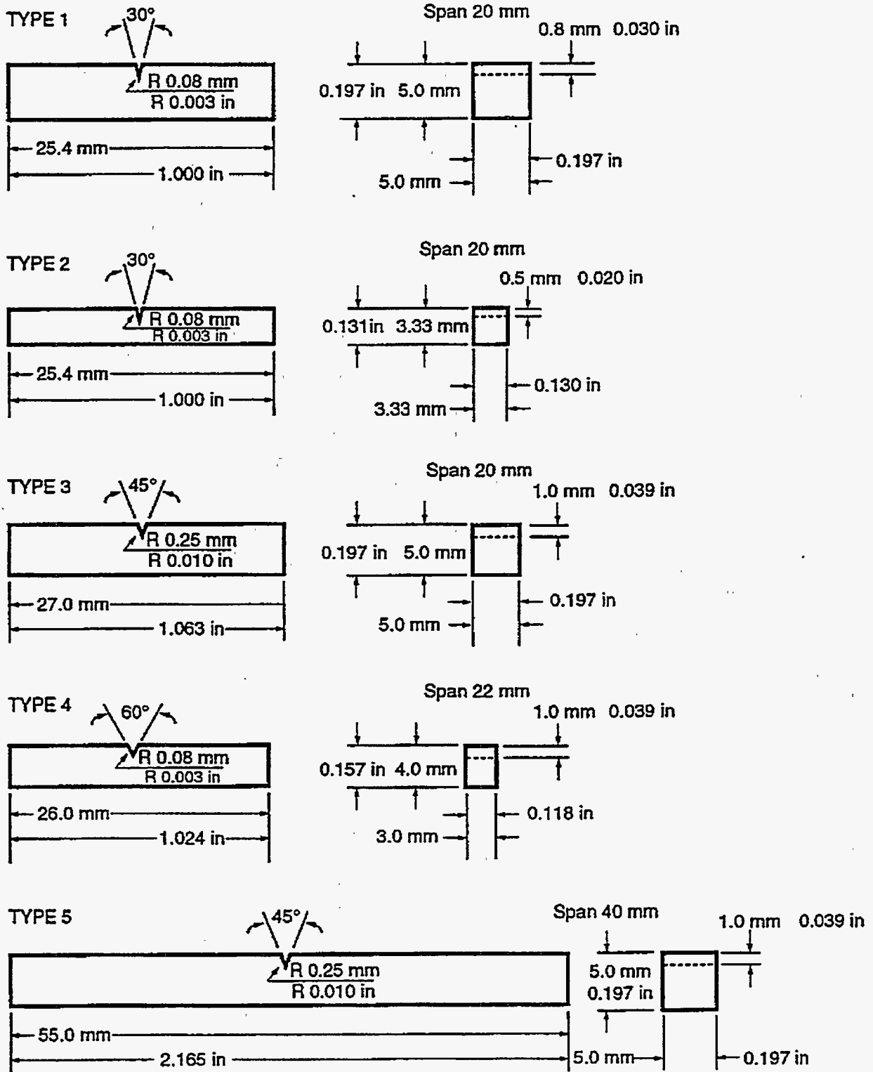
Figure 1. Dimensions of subspecimens used in this study.
