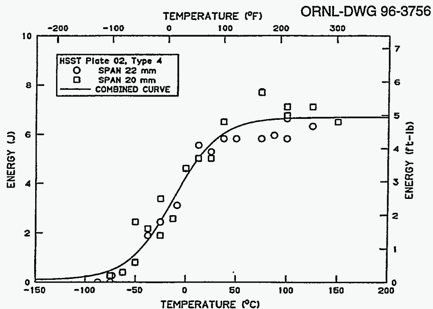
Figure 7. Absorbed energy versus test temperature for type 4 subsized specimens from HSST Plate 02, quarter-thickness location, tested at 22- and 20-mm span.
