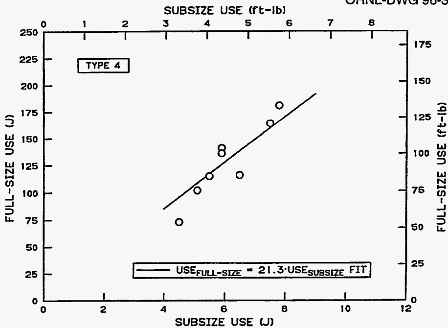
Figure 16. Correlation of upper-shelf energies of full-size and type 4 subsize specimens.
