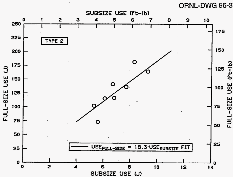
Figure 14. Correlation of upper-shelf energies of full-size and type 2 subsize specimens.
