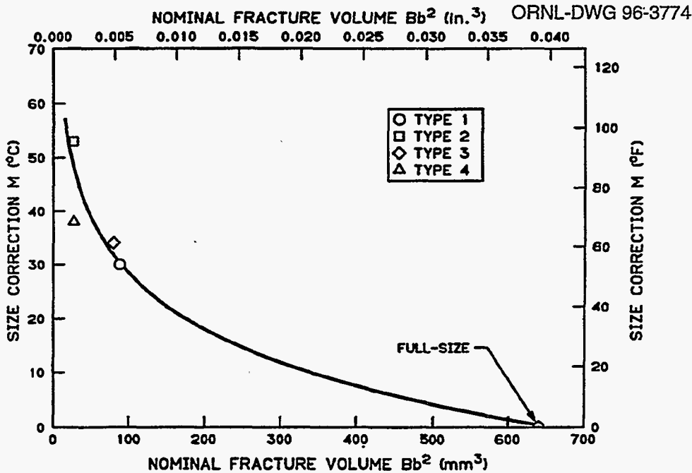
Figure 27. Temperature correction for subsize specimens as a function of nominal fracture volume.
