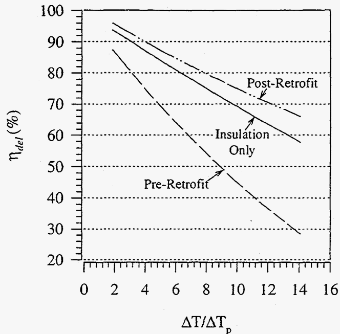
FIGURE 13. Different Parts of the Retrofit on \eta_{del}
