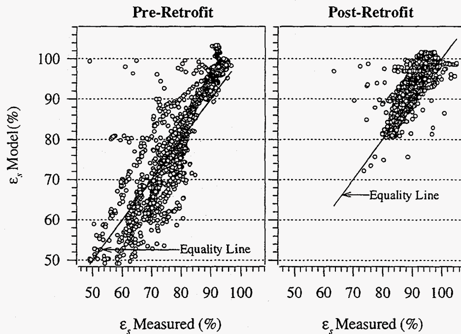
FIGURE 9. Modeled vs. measured supply effectiveness ( \epsilon_s )
