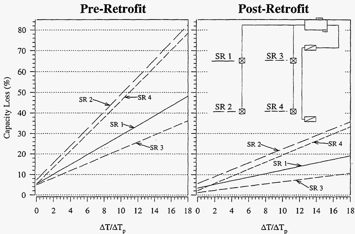
FIGURE 15. Capacity loss at registers
