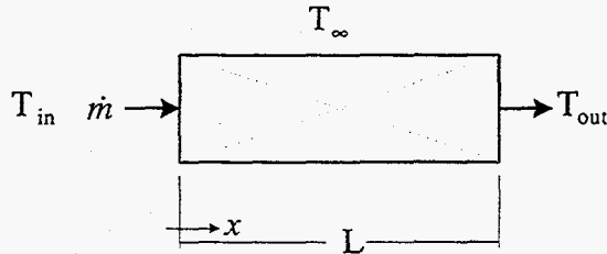
FIGURE 19. Duct segment
