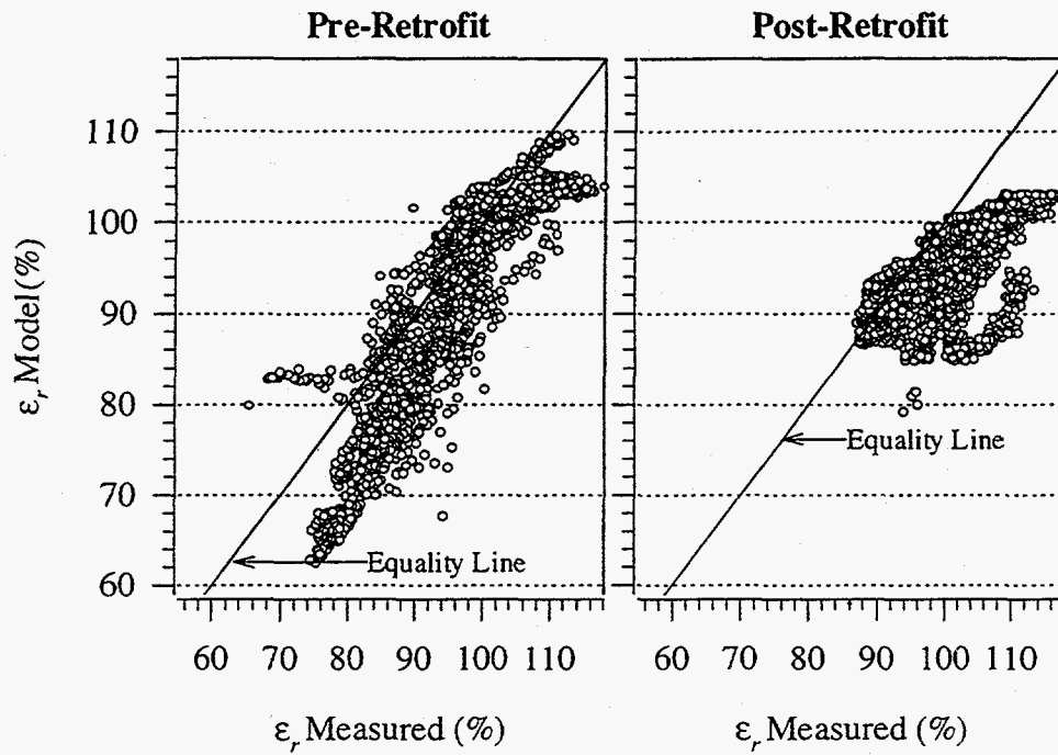
FIGURE 10. Modeled vs. measured return effectiveness ( \epsilon_r )
