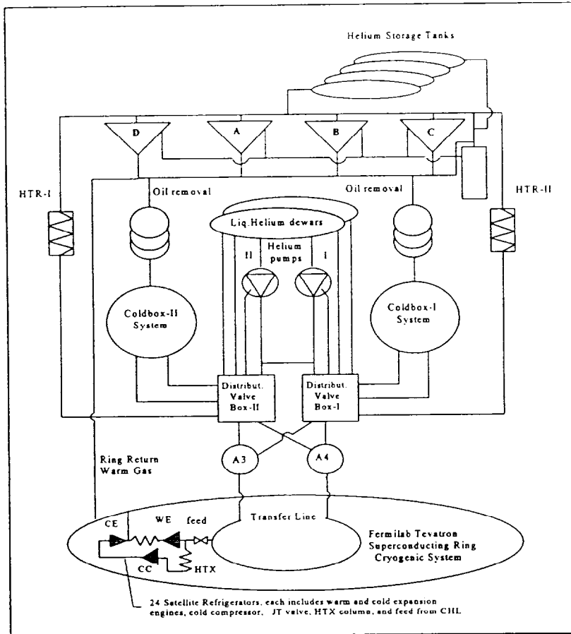
Figure 1. CHL Layout
