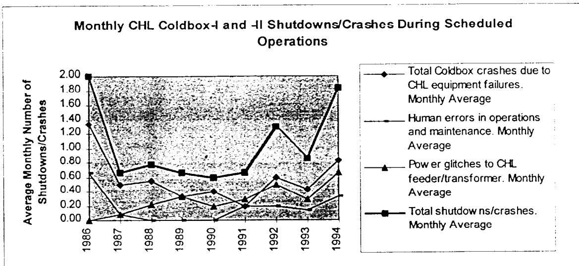
Figure 4. Monthly Average of CHL Coldboxes Shutdowns During Scheduled Operations [Monthly average downtime = (the annual number of downtime hours) / (number of months a year with scheduled operations)]
