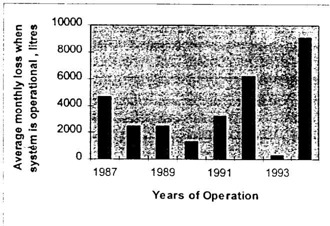
Figure 7. Monthly helium losses due to power outages
