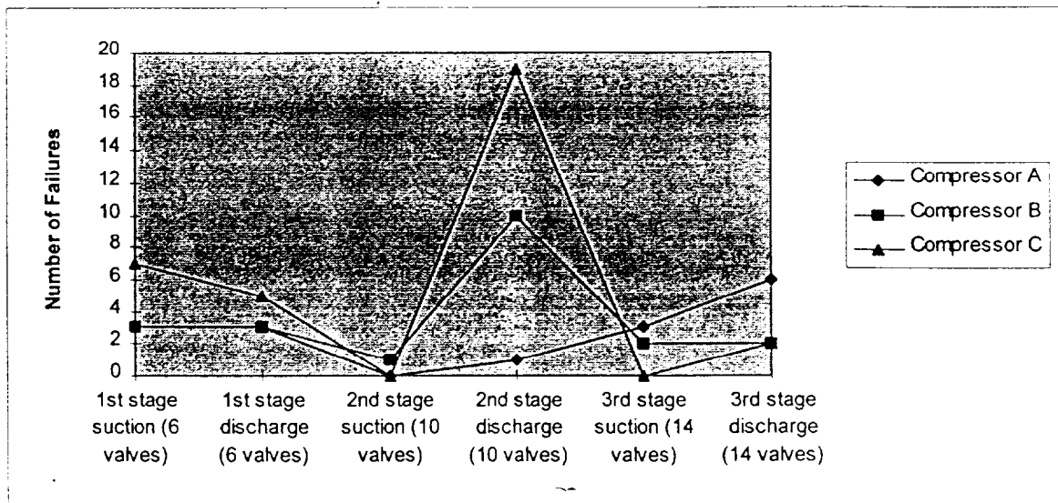
Figure 5. CHL Reciprocating Helium Compressors Valves Failures. 84 - 94.
