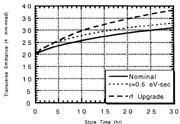
Figure 6. The time dependence of the transverse emittance of the stores described in the text.
