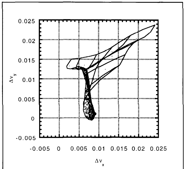
Figure 18. Tune grid and distribution of particle tunes for all 180 crossing points of the last antiproton bunch. The tune distribution is calculated for 2000 particles whose amplitudes were randomly generated from a gaussian beam distribution. The tune shift of the zero amplitude particle is shown by the large dot.
