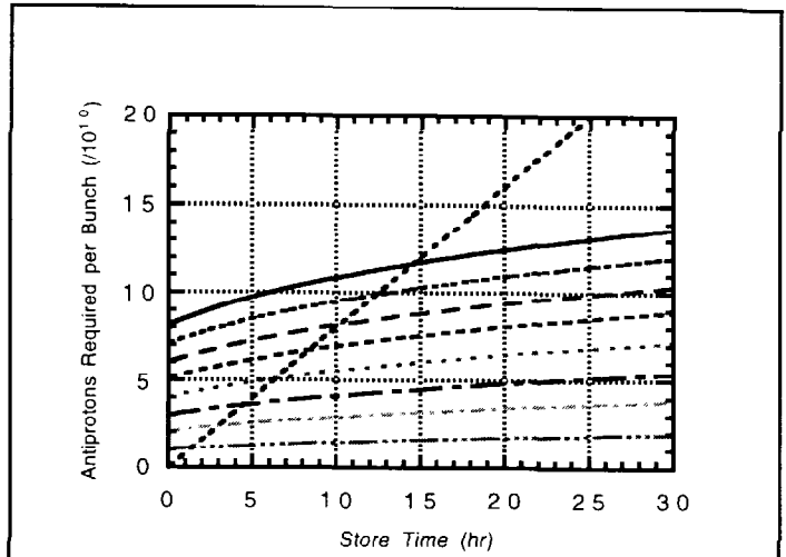
Figure 2. Number of antiprotons per bunch required versus store time for the initial parameters given in Table I but with varying antiproton intensities. The straight line from the origin shows the number of antiprotons produced per colliding bunch as a function of time assuming a stacking rate times transfer efficiency of 0.8 \times 10^{12}/\text{hr} . The initial antiproton intensities are the same as shown in the legend in Figure 1.
