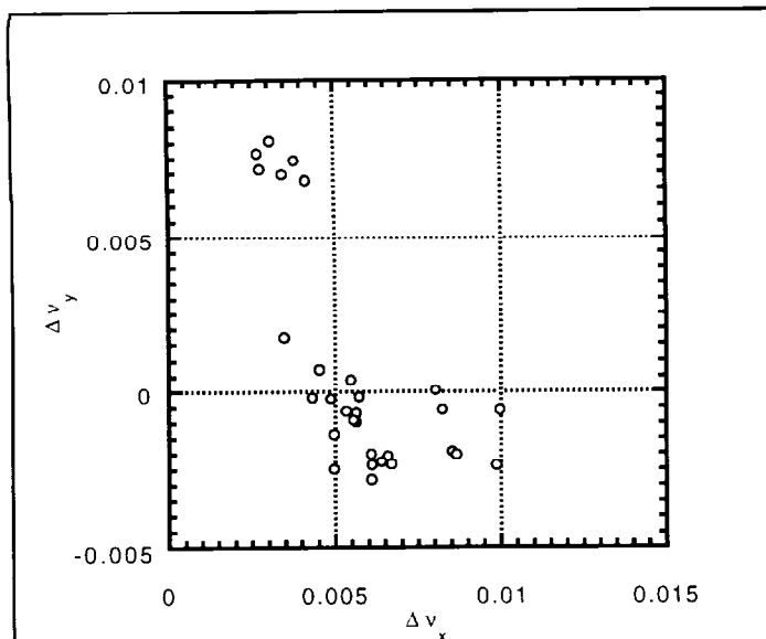
Figure 12. The horizontal and vertical tune shifts for a zero amplitude antiproton in each of the 30 bunches in a group. The tune shift includes the 2 interaction points and the 178 long-range interactions.
