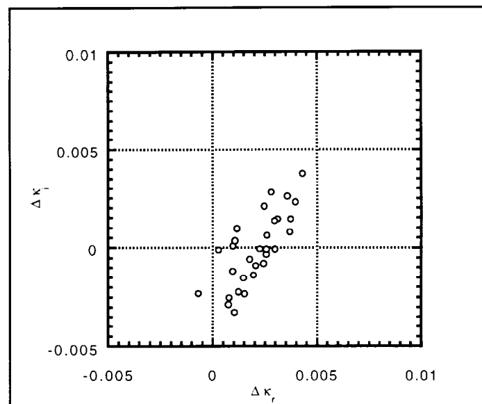
Figure 13. The complex coupling shifts for a zero amplitude antiproton in each of the 30 bunches in a group. The coupling shift includes the 2 interaction points and the 178 long-range interactions.
