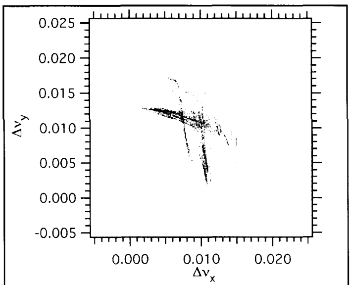
Figure 19. An intensity plot of the distribution of tunes for all 30 antiproton bunches.
