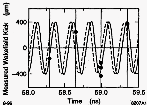
Fig. 2: The average kick in amplitude and sign is plotted versus the time for the different positron buckets. The solid curve has a frequency f = 4142 MHz while f = 4144.5 MHz for the dashed curve.
