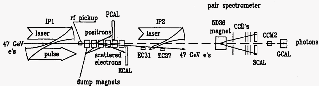
Fig. 8. Sketch of the experiment with the addition of a second laser interaction point to study pair creation by light.
