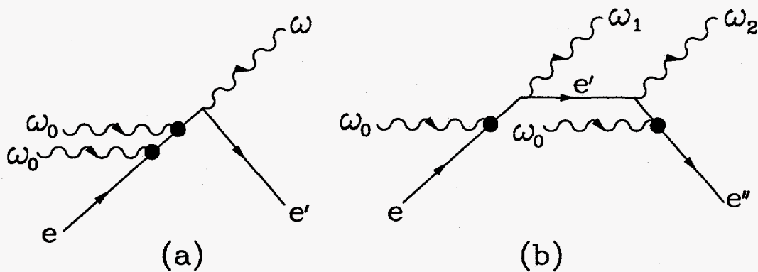
Fig. 2. Diagrams representing (a) n = 2 nonlinear Compton scattering, and (b) double ordinary Compton scattering.
