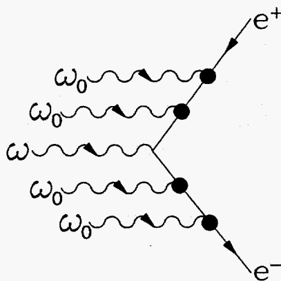
Fig. 3. Diagram representing multiphoton pair creation.
