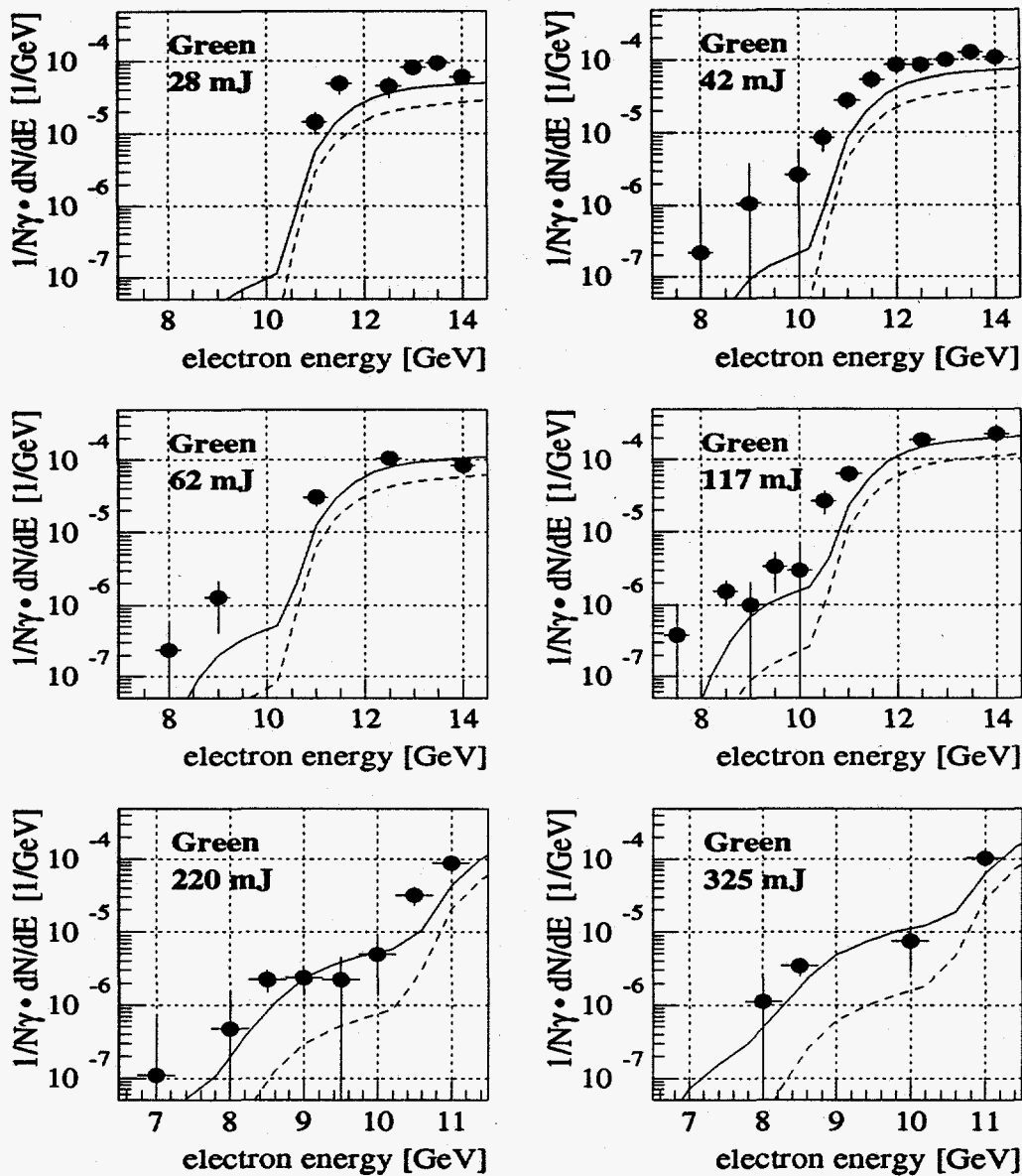
Fig. 16. Energy spectra of scattered electrons for green laser pulses with circular polarization and nominal energies between 28 mJ and 325 mJ. The data (filled-in circles) has been scaled to standard values of the interaction geometry. The solid line represents the full simulation, and the dashed line shows the simulated contribution for multiple ordinary Compton scattering only.
