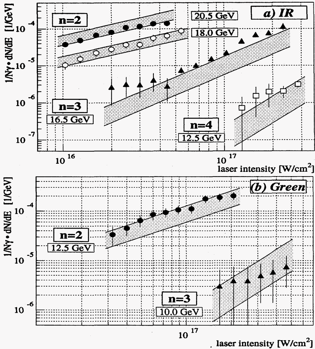
Fig. 17. The normalized rate of scattered electrons of energies corresponding to n = 2, 3, and 4 laser photons per interaction versus the intensity of the laser field at the interaction point for (a) infrared and (b) green laser pulses. The bands represent a simulation of the experiment including an uncertainty in laser intensity of \Delta I/I = 0.3 for infrared and \Delta I/I = {}^{+0.5}_{-0.3} for green.
