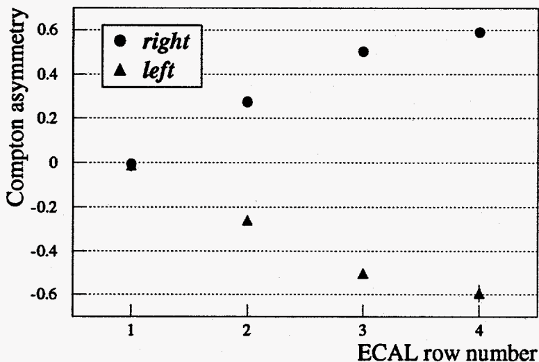
Fig. 12. Measured Compton asymmetry in the top four ECAL rows for right and left circularly polarized laser beams.
