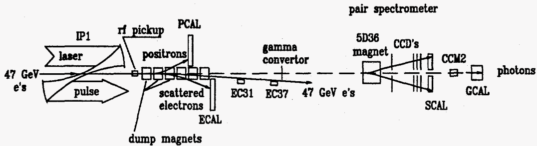
Fig. 7. Sketch of the experiment with the addition of a pair spectrometer to analyze converted Compton photons.
