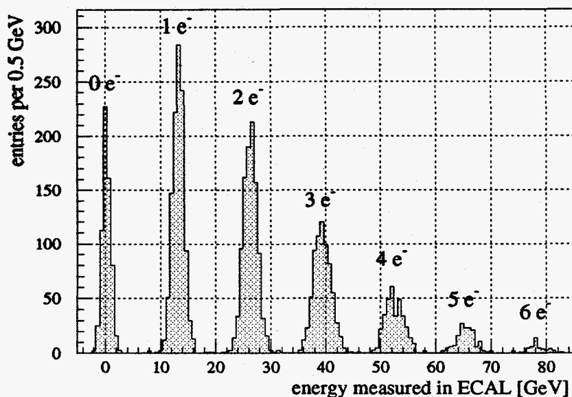
Fig. 6. Energy measured by the calorimeter ECAL during a calibration run with 13 GeV electrons.
