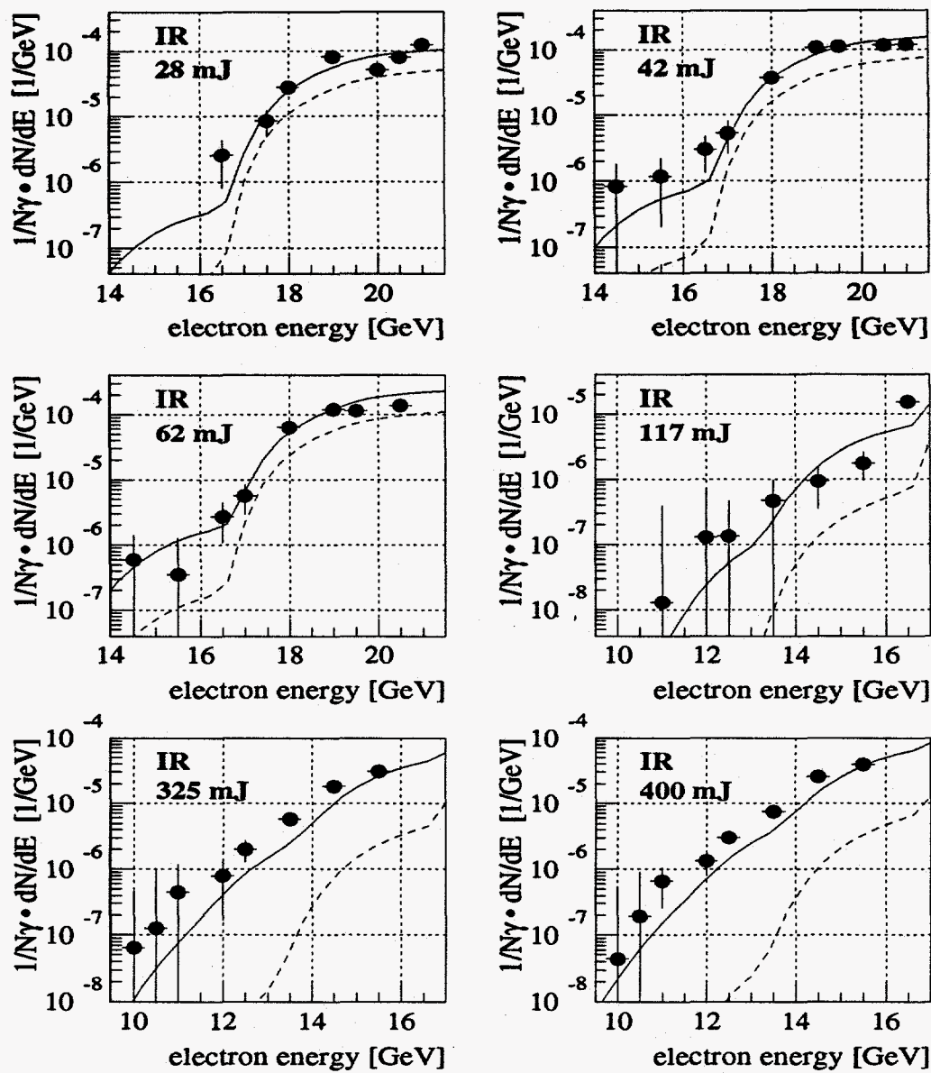
Fig. 15. Energy spectra of scattered electrons for infrared laser pulses with circular polarization and nominal energies between 28 mJ and 400 mJ. The data (filled-in circles) has been scaled to standard values of the interaction geometry. The solid line represents the simulation, and the dashed line shows the simulated contribution for multiple ordinary Compton scattering only.
