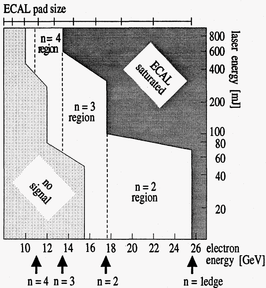
Fig. 13. Data collection strategy for the infrared laser beam. The size of an ECAL pad is shown at the top of the figure. The minimum energy of an electron scattered off n laser photons is indicated at the bottom.
