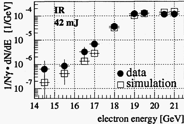
Fig. 14. Energy spectra of scattered electrons as observed in the ECAL calorimeter for infrared laser pulses of 42 mJ energy.
