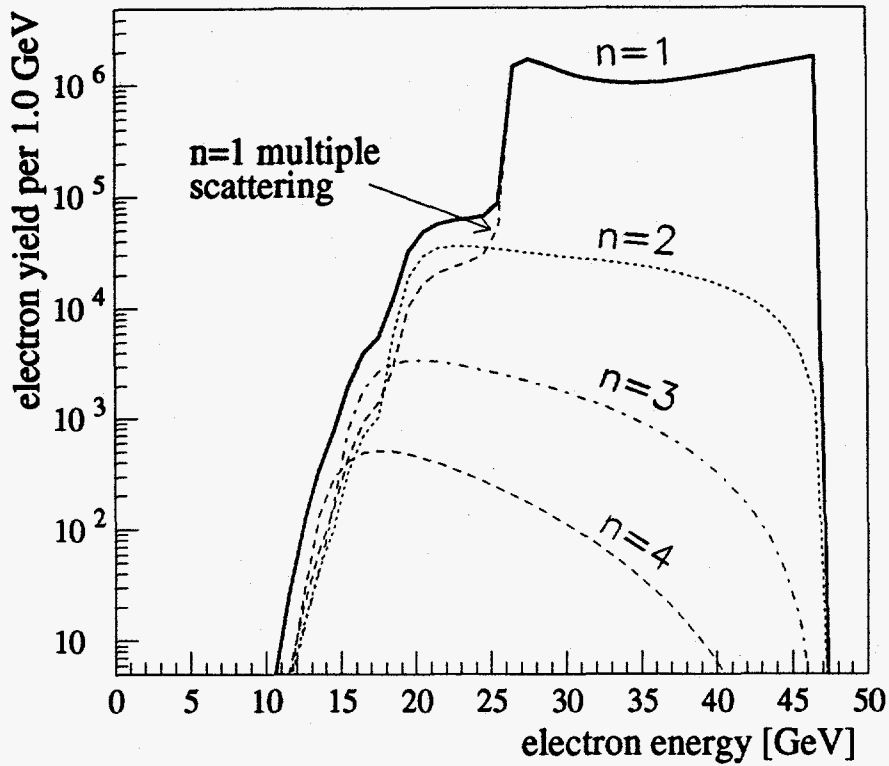
Fig. 1. Calculated yield of scattered electrons from the collision of 5 \times 10^9 46.6 GeV electrons with a circularly polarized 1054 nm laser pulse with intensity parameter \eta = 0.5 .
