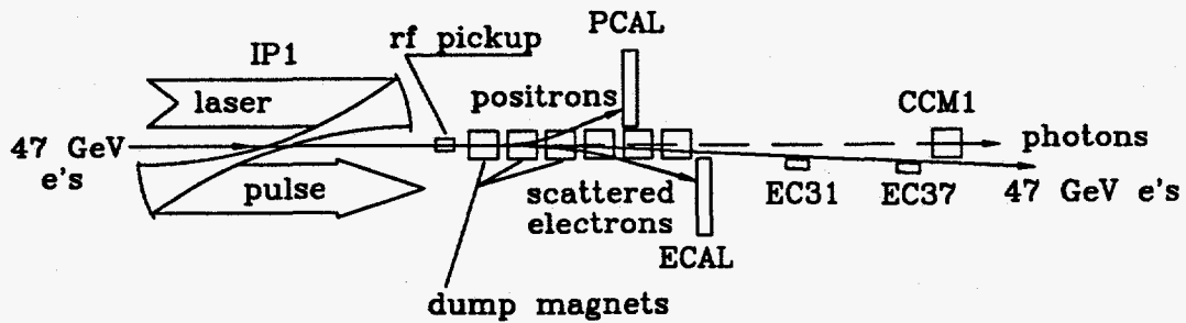
Fig. 4. Sketch of experiment E-144 to detect scattered electrons and positrons produced in e -laser collisions at the SLAC Final Focus Test Beam.
