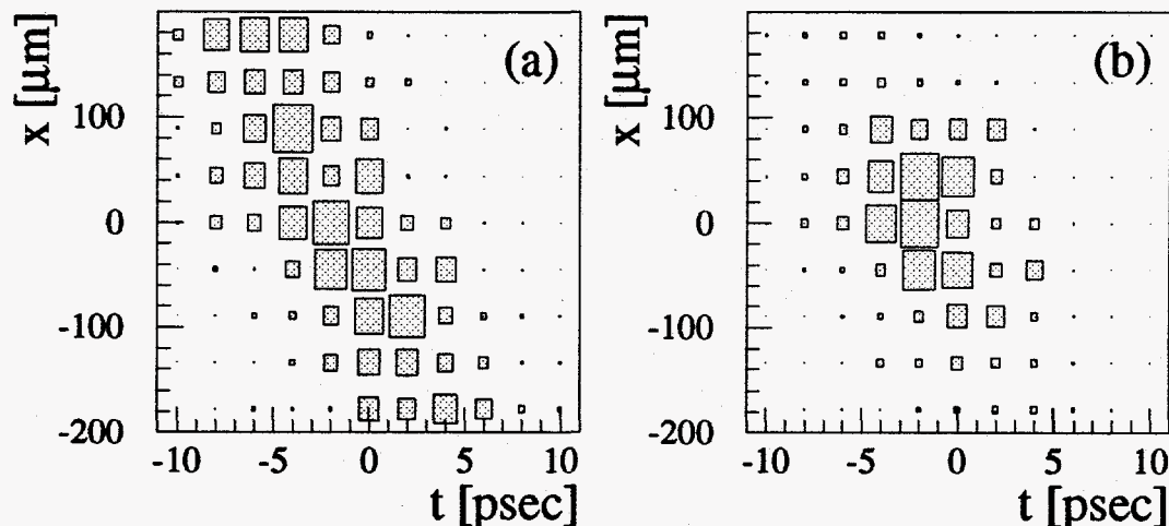
Fig. 11. Observed rates of (a) ordinary and (b) nonlinear and multiple Compton scattering as a function of x and t offsets between the electron and laser beams. The area of each box is proportional to the signal size.
