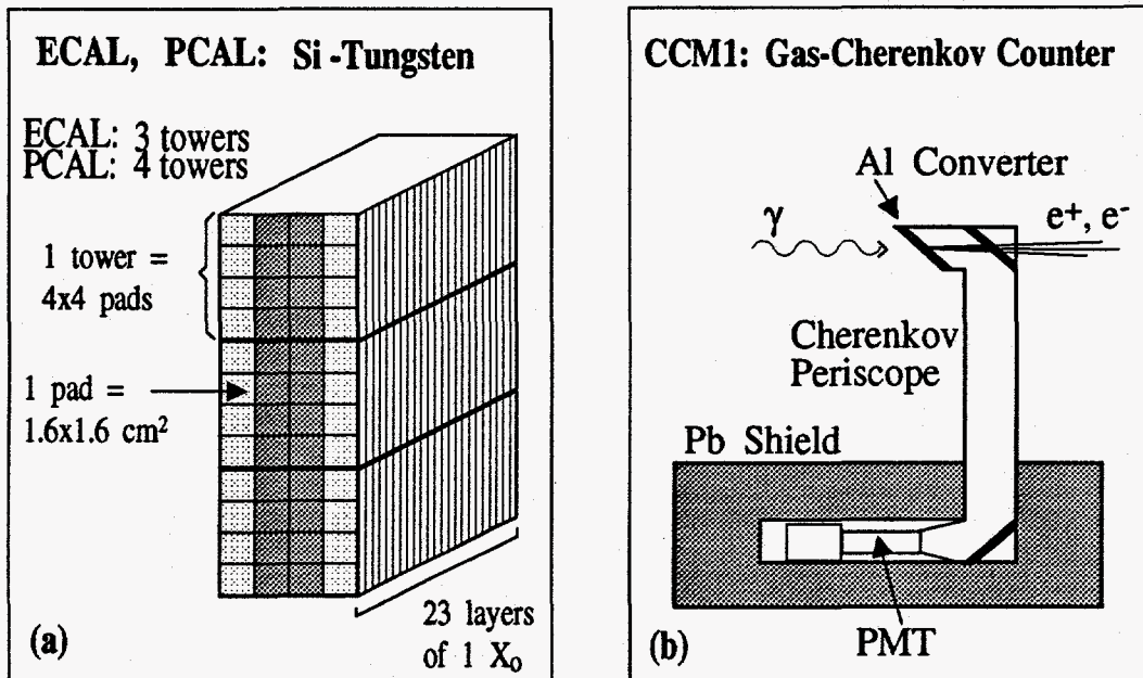
Fig. 5. (a) The Silicon-Tungsten calorimeters ECAL and PCAL. (b) The gas Cherenkov monitor CCM1; monitors EC31 and EC37 are of similar construction.
