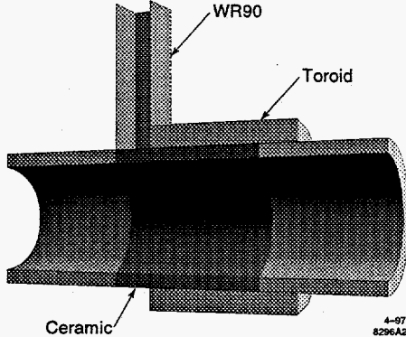
Figure 4: Model for the numerical calculation of beam-waveguide coupling using MAFIA [4].
