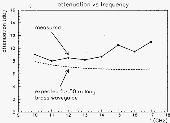
Figure 6: Measured attenuation of TE_{10} mode.
