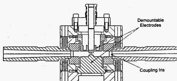
Fig. 4. TM 020 RF breakdown test cavity assembly
