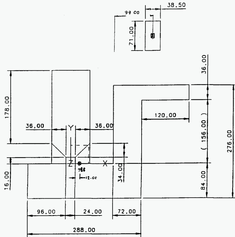
Fig. 1. Two-dimensional model of HFIR reactor vessel subjected to dynamic impact caused by a drop of the GE-2000 cask. The cask weighs 25,000 lb and the weight drops from a height of 20 ft.
