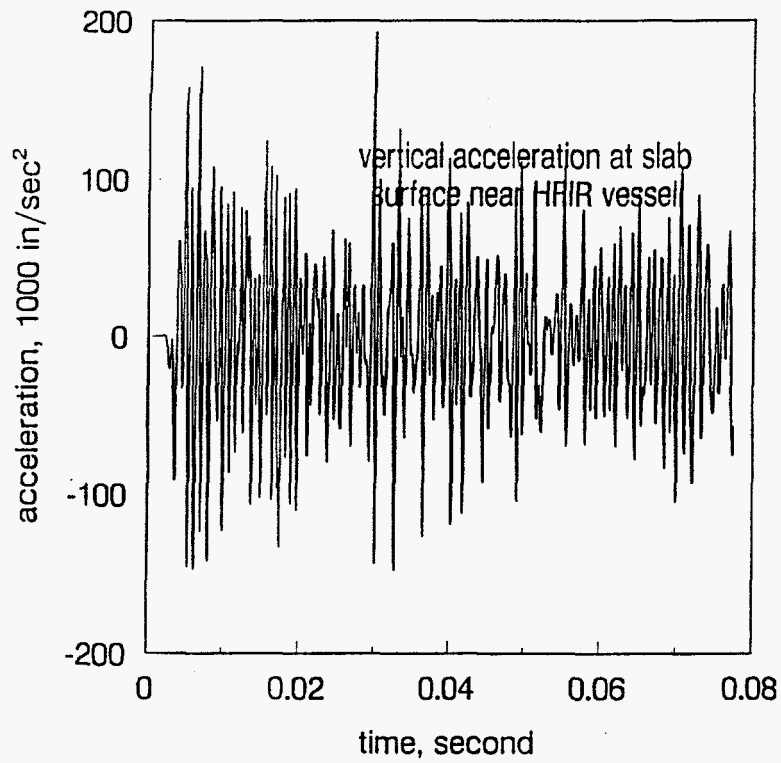
Fig. 4b. Vertical acceleration at the surface of the reactor supporting concrete slab near the HFIR lower vessel wall at node 786.
