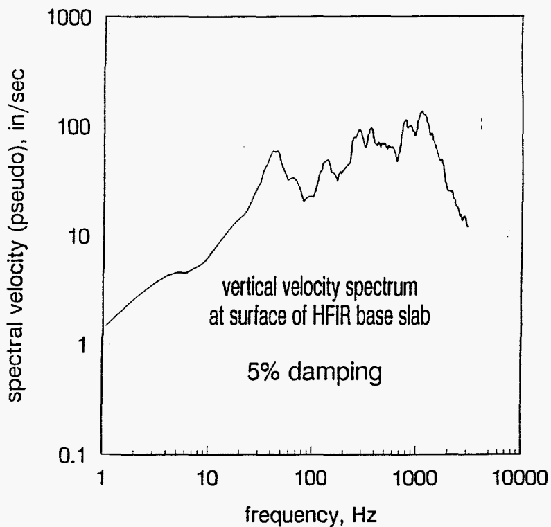
Fig. 5b. Vertical velocity response spectrum at node 786.
