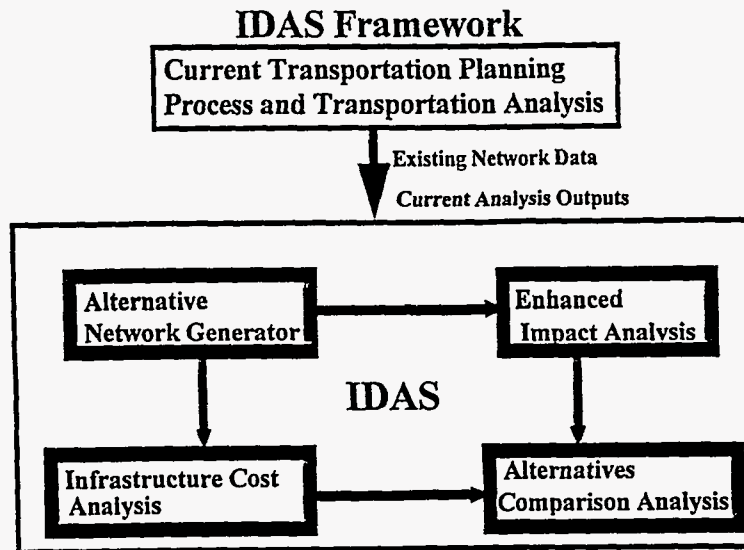
Figure 1—IDAS Framework
