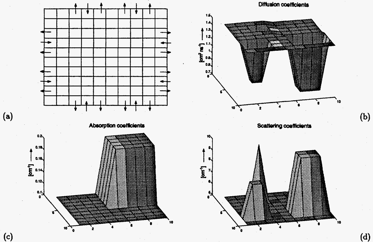
Figure 1. (a) Shows the set-up for a 10x10 grid with 0.1 cm separation between grid points. The arrows pointing inward show the location of the sources and the arrows pointing outward show the detector positions. (b), (c), and (d) show the diffusion, absorption, and scattering coefficients respectively.
