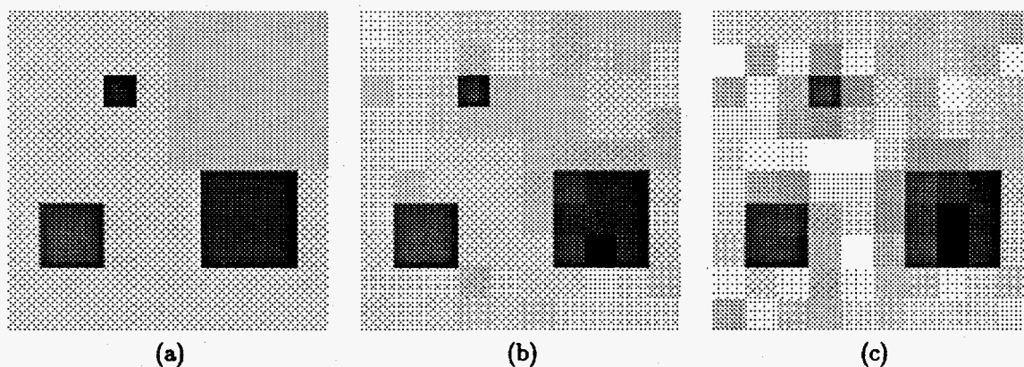
Figure 3. (a) Original diffusion coefficients. Reconstructed diffusion coefficients for the 10x10 grid using the GGMRF image model with (b) p = 1.1 , and (c) p = 2.0 (Quadratic regularization). Note that white in the images corresponds to 1.54 \text{ cm}^2\text{ns}^{-1} and black corresponds to 0.58 \text{ cm}^2\text{ns}^{-1} .
