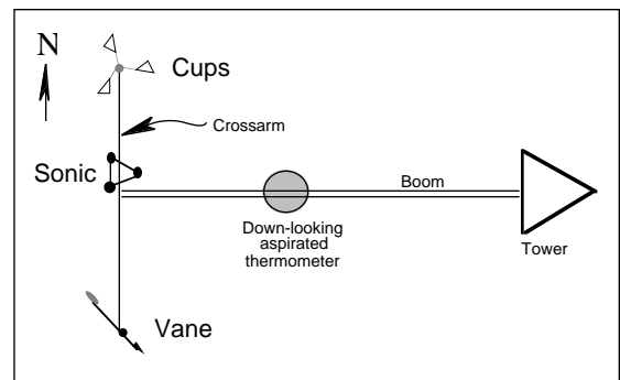
Figure 1. Sensor, crossarm, boom and tower layout.
