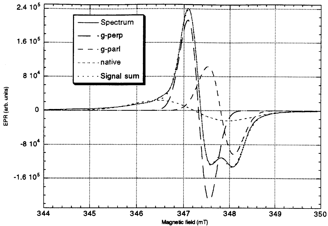
Figure 4 Deconvoluted spectra of enamel given 100 Gy dose.
