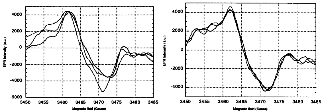
Figure . Powdered enamel sample shaken between spectra. Left, no rotation. Right, with rotation during measurement. Spectra are low bandpass filtered to show differences clearly. (From Haskell, et al., 1996A).
