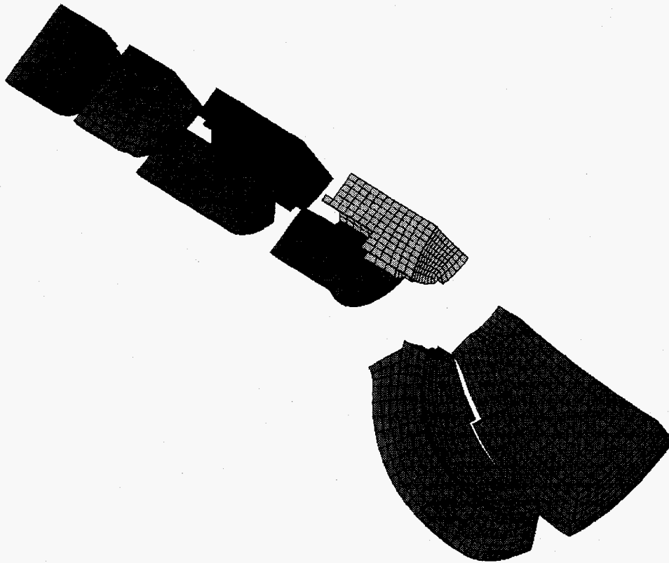
FIG. 1. The chalice mesh, decomposed for 8 processors by CHACO [3].
