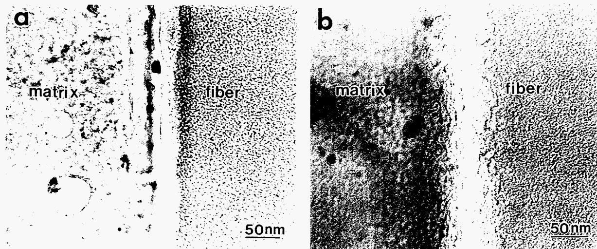
Fig. 5 TEM bright field images of fiber/matrix interfacial region:(a) MAS5/SiC; (b) MAS0/SiC
