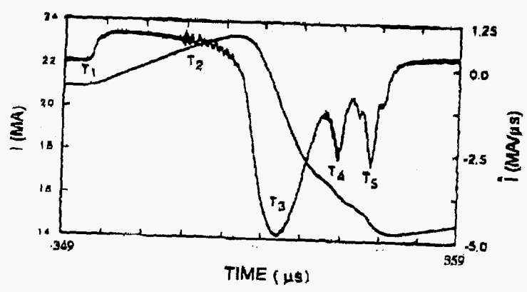
Figure 6c. I(A) and I(B) during switching and transfer phase. t_1 is initial motion of EFF, t_2 is closing switch time, t_3 is peak transfer time, and t_4 and t_5 are PFS switching and implosion times.
